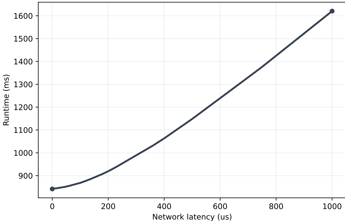
Fig. 5 Llama7B Composite-LP historical mode Paper/reference
