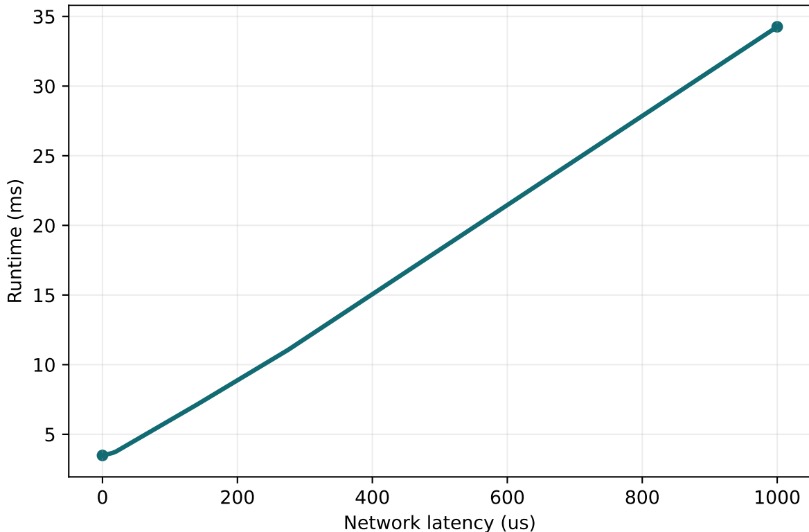
Fig. 3 AllReduce 128MiB, 16 nodes, auto channels Regenerated
