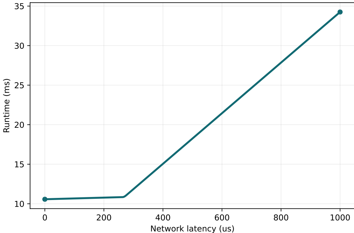
Fig. 3 AllReduce 128MiB, 16 nodes, 1 channel Regenerated
