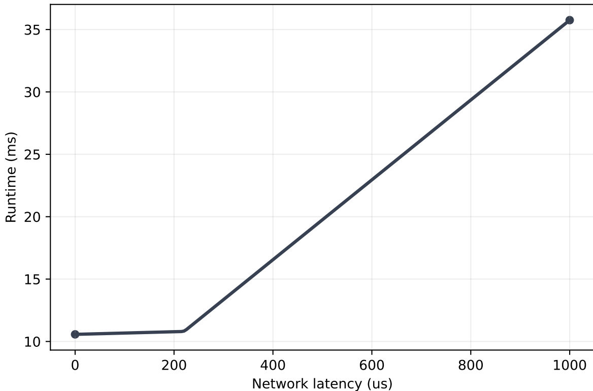
Fig. 3 AllReduce 128MiB, 16 nodes, 1 channel Paper/reference
