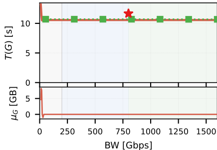
Grok (4096 GPUs) — Bandwidth
