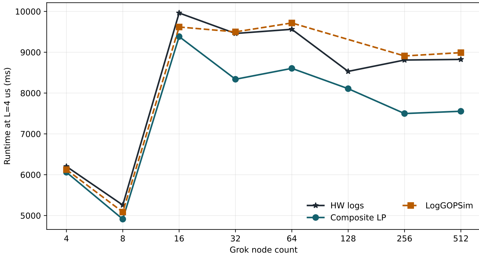
Grok scaling: measured HW vs predicted runtime
