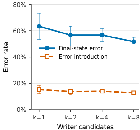
Incremental typed mechanism
