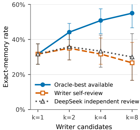
Generation vs. selection
