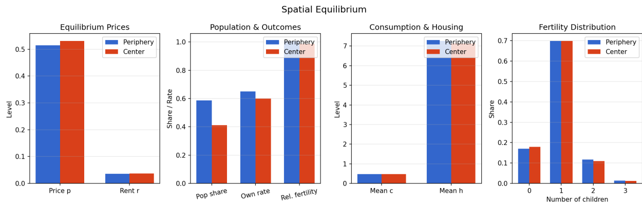
Figure 6: Market equilibrium
