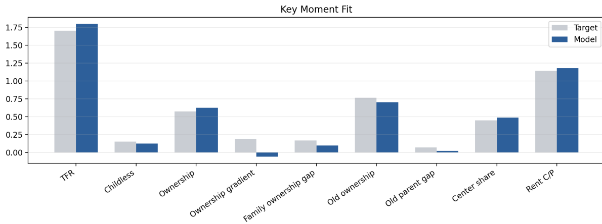
Figure 1: Key moment fit
