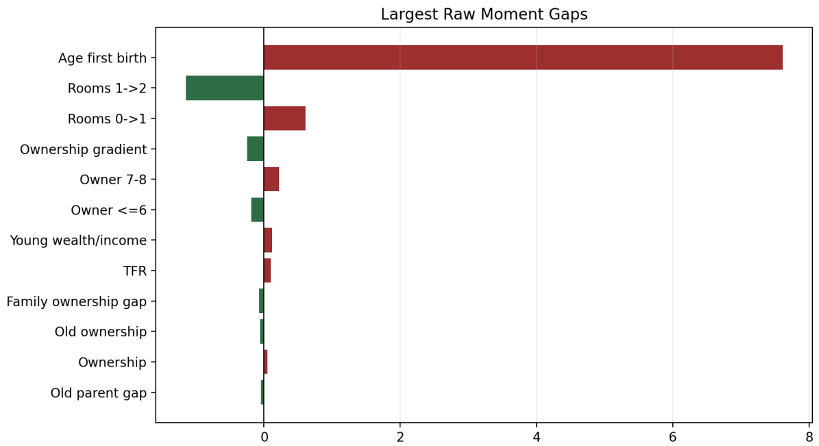
Figure 3: Largest raw moment gaps
