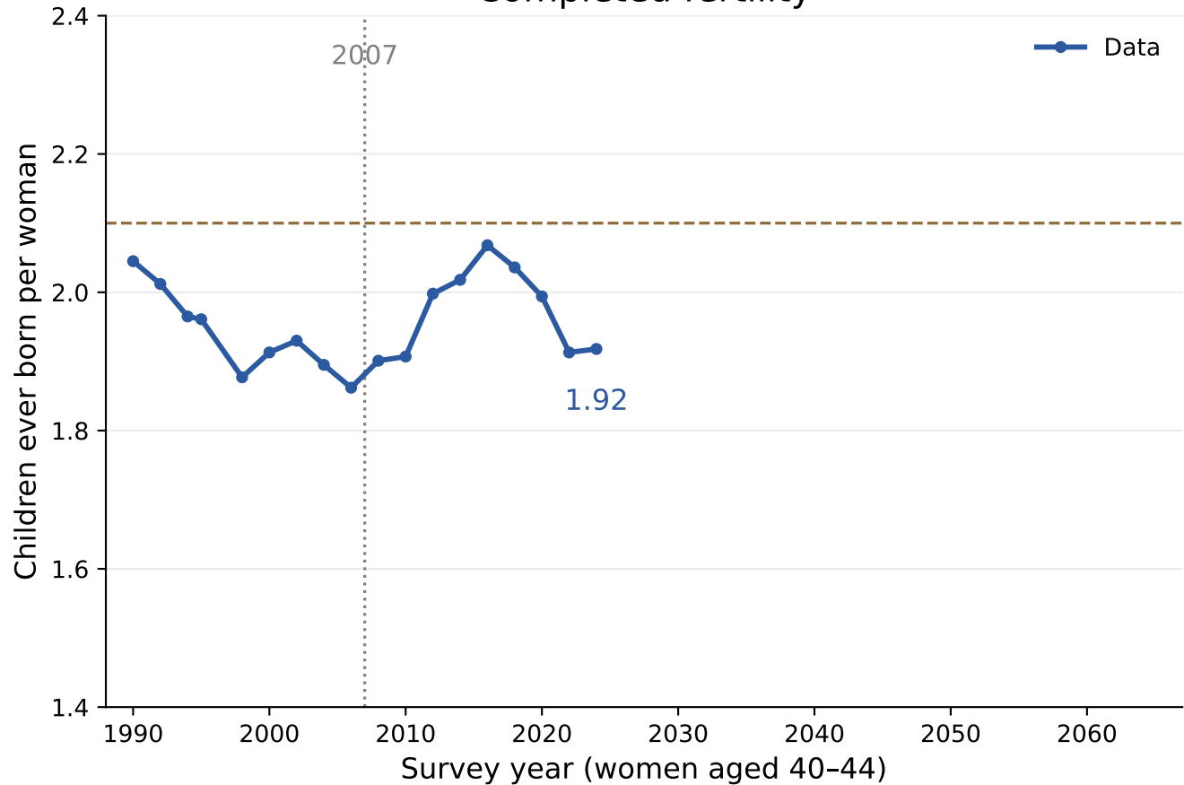
Completed fertility
