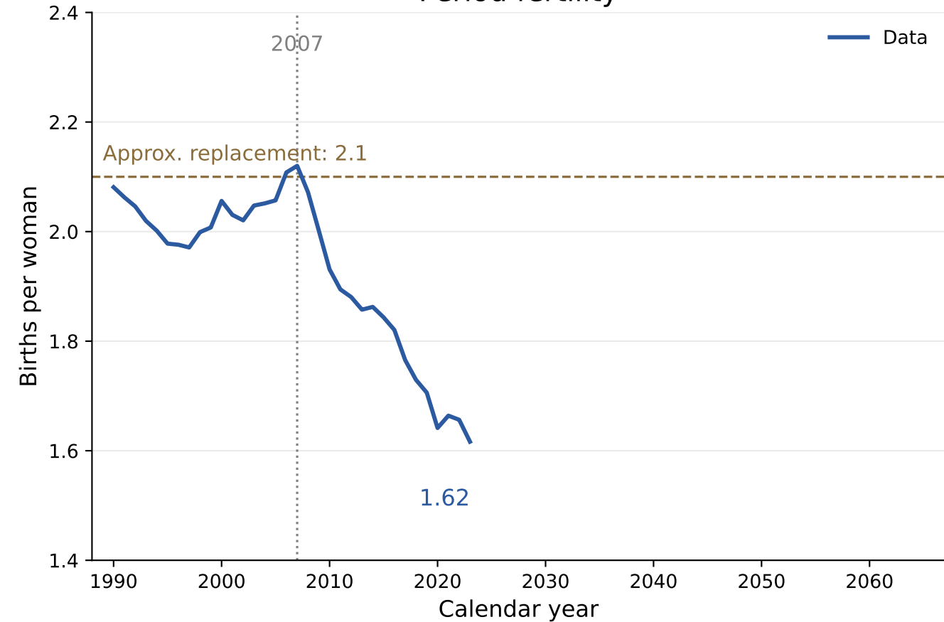
Period fertility
