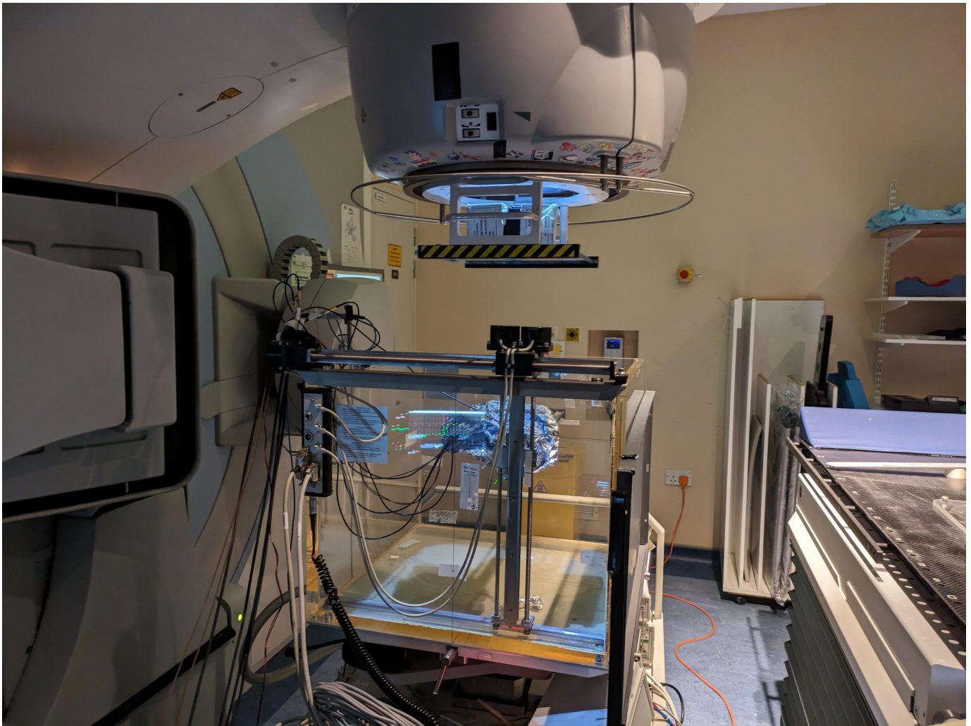
Beam monitoring of a high-rate linac for radiotherapy (Dublin, Ireland)
