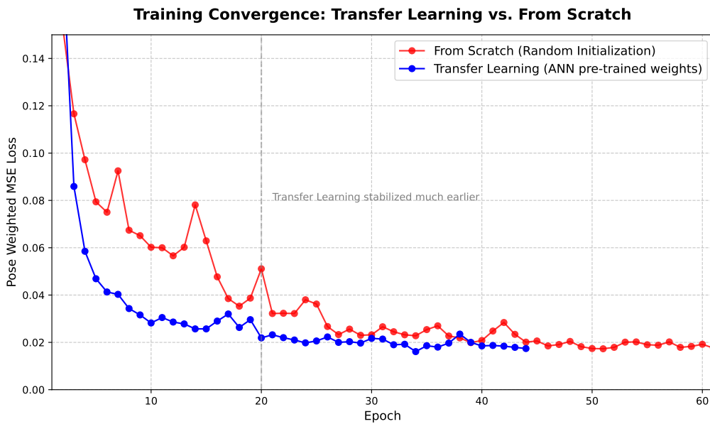
Figure 7: Comparison of the Custom Pose Weighted Mean Squared Error (MSE) Loss progression over 60 epochs. The Transfer Learning approach (blue) demonstrates stable convergence, whereas training from scratch (red) exhibits instability and error spikes.
