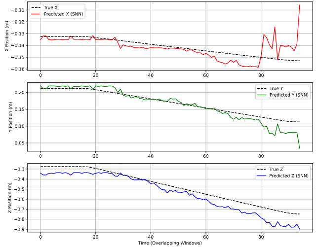
Figure 6: Trajectory errors caused by sequential spike attenuation when adding a 3rd convolutional layer, exhibiting tracking loss during the final approach.
