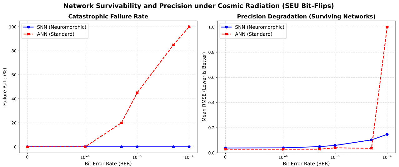
Figure 10: Network survivability and precision under simulated cosmic radiation (Monte Carlo SEU injection). Left: Failure rate as a function of BER. Right: Precision degradation (Mean RMSE) of the surviving network inferences.
