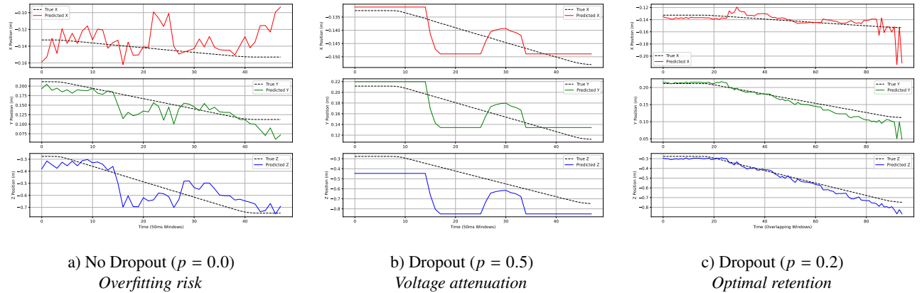
Figure 4: Sensitivity analysis on the Dropout probability ( p ). Without dropout (a), the network risks overfitting on dominant features. A standard p = 0.5 (b) causes voltage attenuation and tracking errors in sparse DVS data. The optimized p = 0.2 (c) balances regularization with spike propagation.
