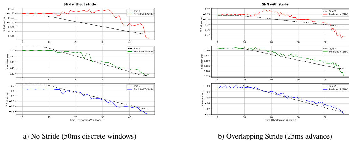
Figure 2: Impact of the overlapping stride on spatial tracking. Without stride (a), the network successfully tracks the target but exhibits noticeable high-frequency jitter and lower temporal resolution. The overlapping stride (b) doubles the temporal resolution (from \sim 45 to > 90 windows), preserving temporal continuity and yielding a smoother tracking curve during the approach.
