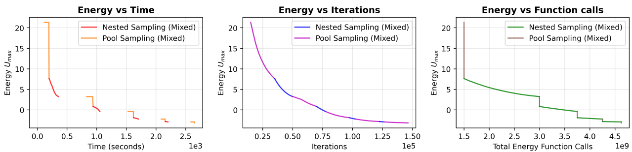
Figure 9: Benchmark graphs of the mixed scheme, looking at energy scaling with execution time, global steps and energy function calls.
