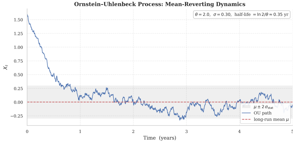
Figure 8.1: OU process
