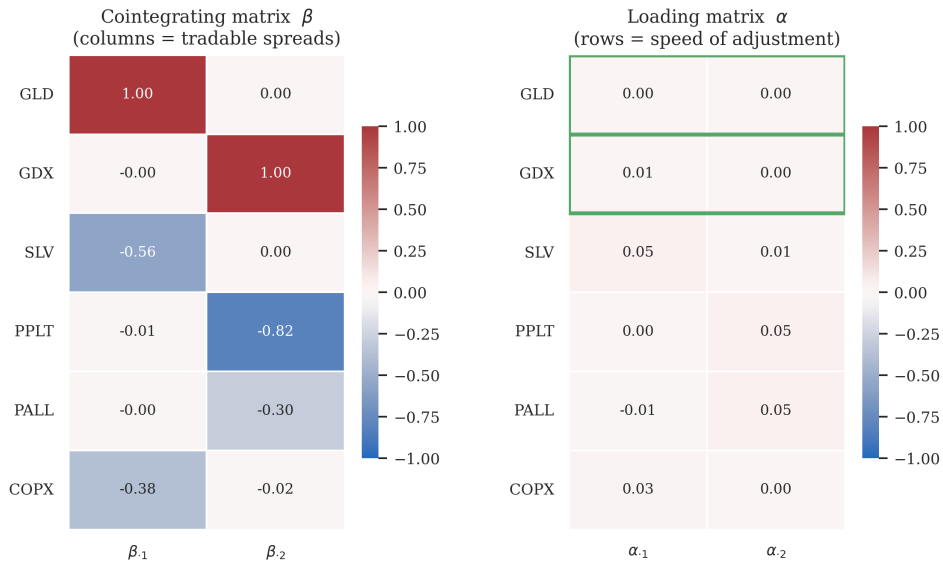
VECM Decomposition \Pi = \alpha\beta' : Spreads, Adjustment Speeds and Price Leaders
