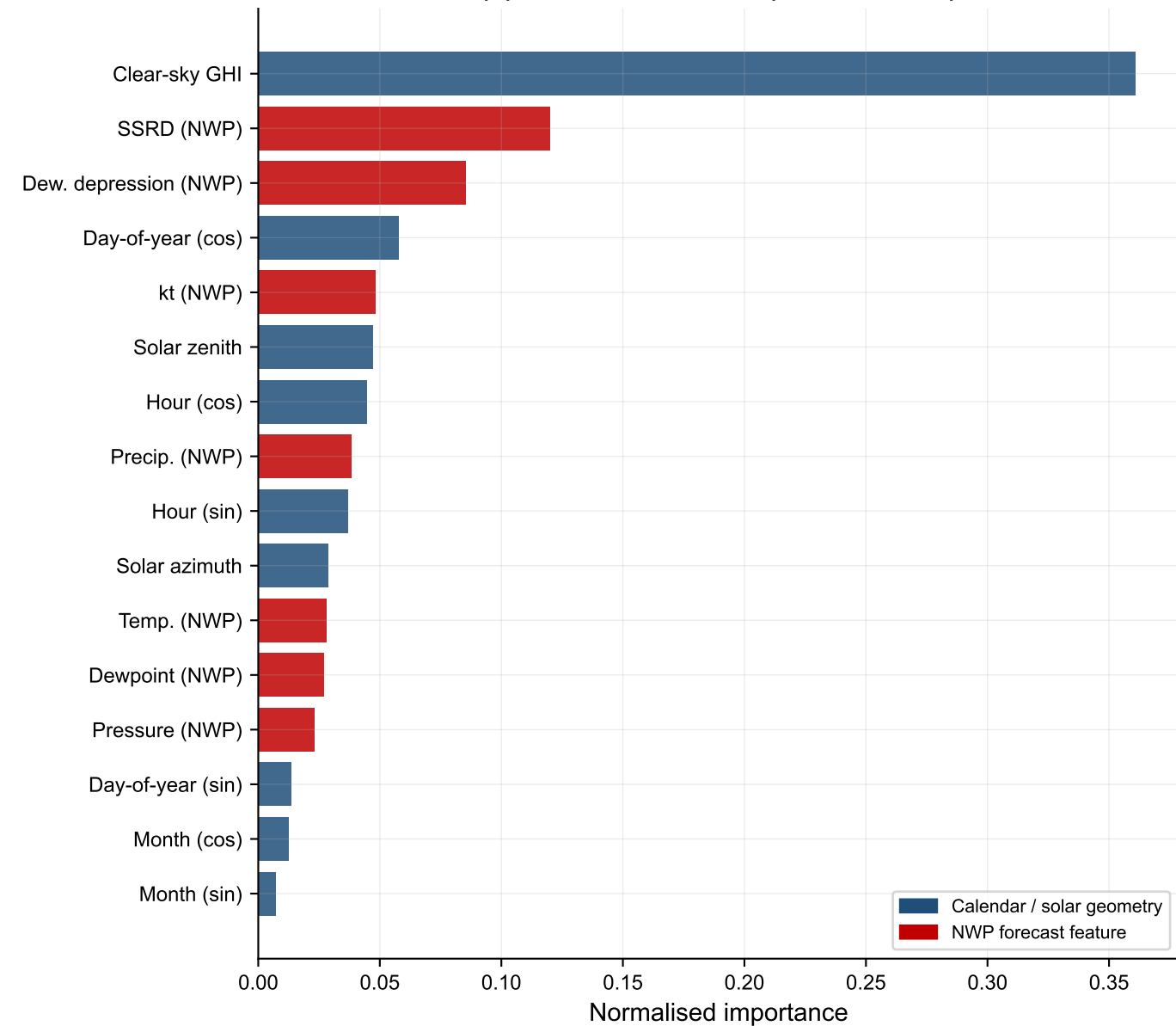
(b) Decoder variables (known future)
