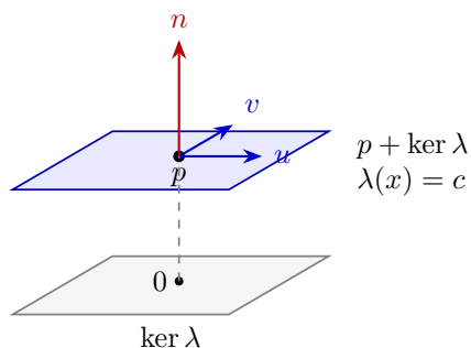
Figure 10.1: An affine plane and its parallel direction plane. The arrows u, v span the direction space; a Euclidean normal n represents the covector. Orthogonality is spatial, not an angle measured on this oblique drawing.
