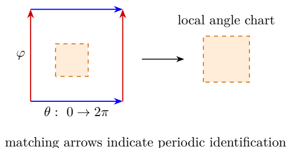
Figure 13.5: The parameter square is an intuition for periodic angles, not a quotient-topology proof. A small open rectangle supplies local coordinates; the full square repeats opposite sides.
