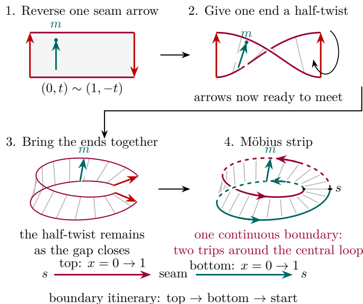
Figure 13.7: A half-twist implements the reversed seam rule. In the second panel the band is viewed obliquely through the twist; crossing strokes are projection effects. The marker m follows the same transverse segment. Dashed rear arcs and white gaps distinguish depth at projected crossings. Starting at s , the purple and teal portions trace one boundary: the edge that starts on top returns along the bottom before closing. See Section C.5 for the local charts.
