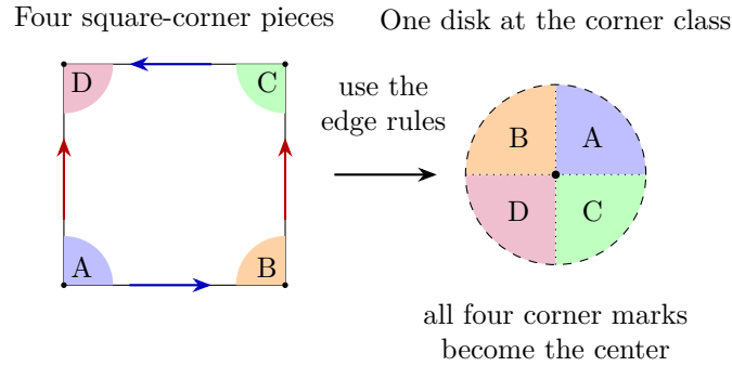
Figure C.6: The Klein-bottle corner chart. Bottom-left A stays in the positive quadrant; bottom-right B translates left. Top-right C and top-left D reflect horizontally and translate down, as in the displayed representative table. The four pieces fill a disk with no missing quadrant, boundary, or singular corner. The outer dashed circle is excluded.
