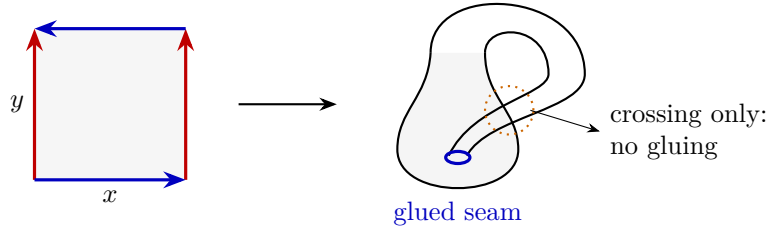
Figure C.7: Klein quotient: (0, y) \sim (1, y) and (x, 0) \sim (1 - x, 1) . The solid blue seam represents the joined circles; the dotted callout marks an incidental crossing of distinct sheets. The drawing in \mathbb{R}^3 is not an embedding. See Figure 13.8 for the deformation and Figure C.6 for the local disk at the corner class.
