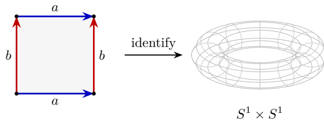
Figure C.3: Torus quotient: (0, y) \sim (1, y) and (x, 0) \sim (x, 1) . The arrows agree on each paired edge, and all four vertices form one class. Figure 13.5 gives the full geometric sequence.
