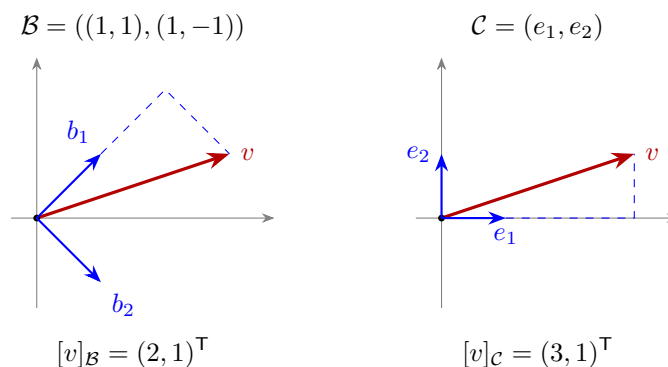
Figure 10.4: One vector, two coordinate columns. The dashed routes build v = 2b_1 + b_2 = 3e_1 + e_2 ; the red vector stays fixed.
