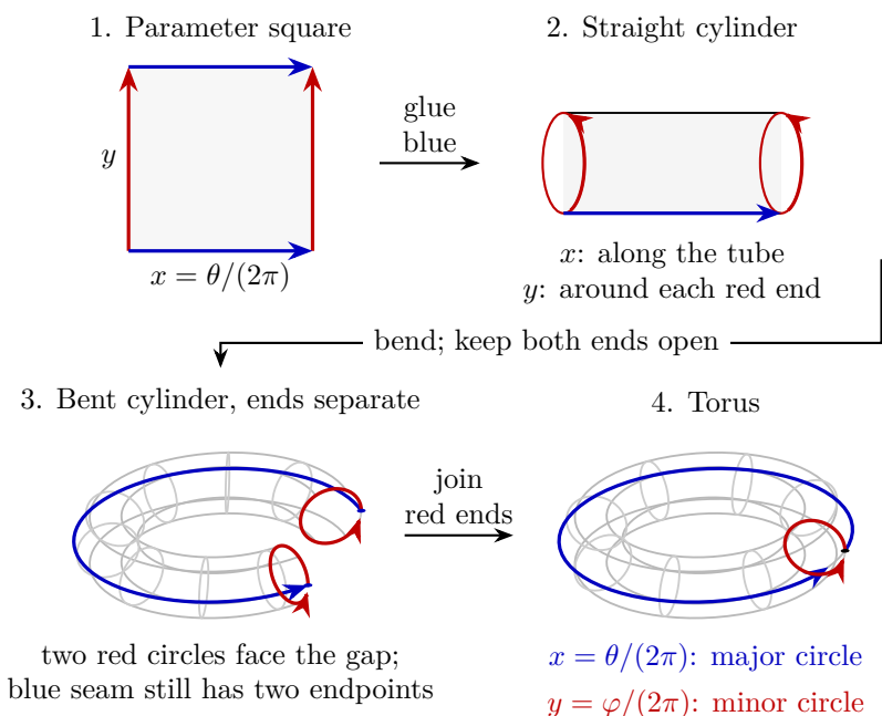
Figure 13.5: Square, straight cylinder, bent cylinder, and torus. Glue the blue edges first, making y circular while x runs along the tube. Bending preserves these directions. The two red end circles remain separate in panel 3; joining corresponding points closes the blue x -curve in panel 4. Either pair can be glued first, but this order agrees throughout with the angles in Figure 13.4. The square is a fundamental domain, not a global chart; see Section C.4.
