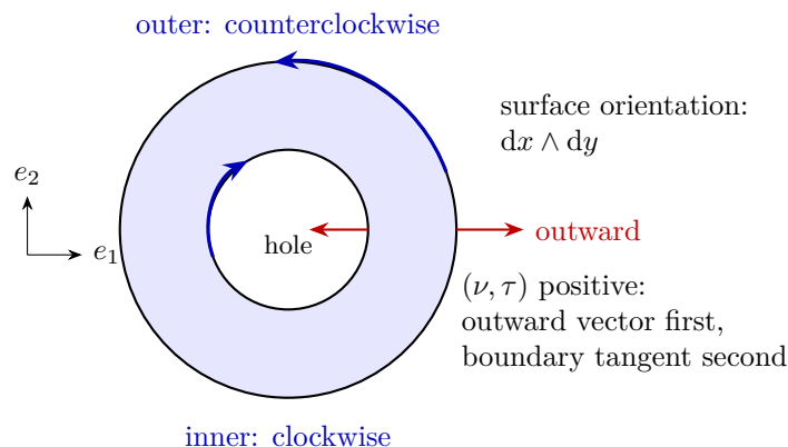
Figure 13.9: Outward-first on a standard oriented annulus. At the rightmost outer point, outward is right and the positive tangent is up. At the rightmost inner point, outward is left into the hole and the positive tangent is down. Thus the two boundary components run in opposite senses.
