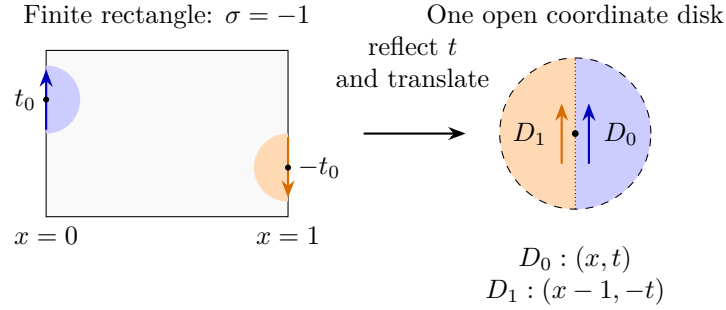
Figure C.5: A Möbius seam chart. The right-edge piece is centered at (1, -t_0) and is reflected transversely before being placed to the left of the piece at (0, t_0) . Both arrows then point in the same chart direction. For the cylinder use (x - 1, t) instead, without reflection. At a boundary endpoint the corresponding quarter-disks assemble into a half-disk. Dashed arcs indicate excluded disk boundaries.
