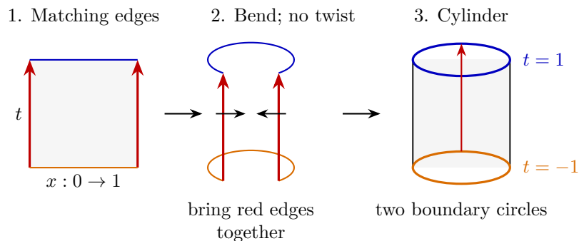
Figure 13.6: The cylinder glues (0, t) to (1, t) . The red arrows match without reversal; bending brings these edges together. The two unglued long edges close separately into the highlighted boundary circles.
