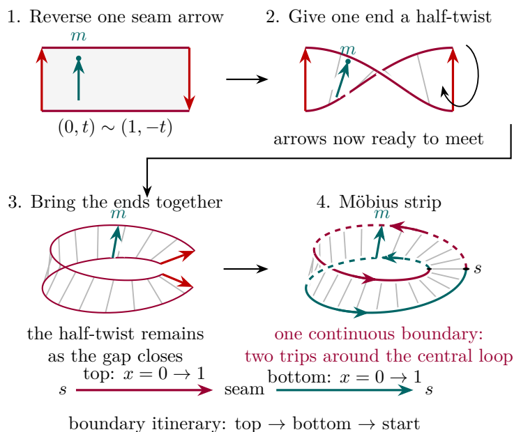
Figure 13.7: A half-twist implements the reversed seam rule. In the second panel the band is viewed obliquely through the twist; crossing strokes are projection effects. The marker m follows the same transverse segment. Dashed rear arcs and white gaps distinguish depth at projected crossings. Starting at s , the purple and teal portions trace one boundary: the edge that starts on top returns along the bottom before closing. See Section C.5 for the local charts.
