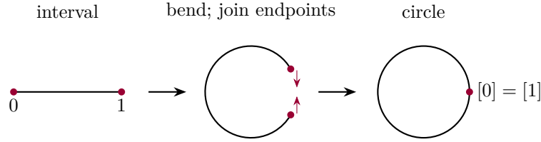
Figure C.1: Joining the interval's two purple endpoints gives one circle point. A neighborhood of that point joins short intervals near both endpoints. This explains the seam without mistaking the whole closed interval for a single circle chart.
