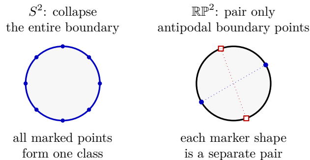
Figure C.9: Two different disk quotients. For the sphere, all of \partial D^2 collapses together. For the projective plane, u \sim -u only on the boundary; interior points stay distinct. Dotted chords indicate pairings, not curves collapsed in the disk.
