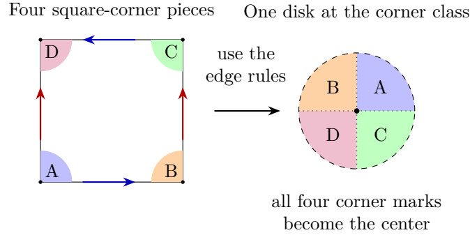
Figure C.7: The Klein-bottle corner chart. Bottom-left A stays in the positive quadrant; bottom-right B translates left. Top-right C and top-left D reflect horizontally and translate down, as in the displayed representative table. The four pieces fill a disk with no missing quadrant, boundary, or singular corner. The outer dashed circle is excluded.
