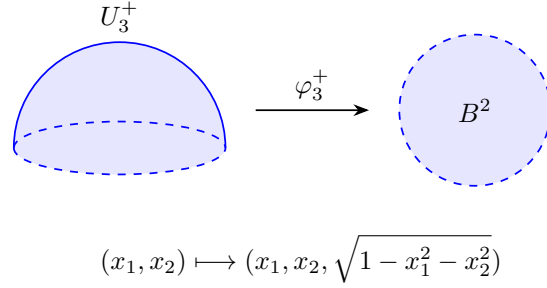
Figure 13.2: Deleting the third coordinate maps the open upper hemisphere to the open unit disk. The formula below reconstructs the hemisphere; both boundary circles are excluded.
