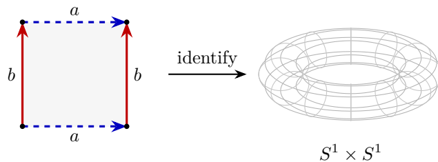
Figure C.3: Torus quotient: (0, y) \sim (1, y) and (x, 0) \sim (x, 1) . The dashed a -edges and solid b -edges distinguish the two pairs. The arrows agree on each paired edge, and all four vertices form one class. Figure 13.5 gives the full geometric sequence.
