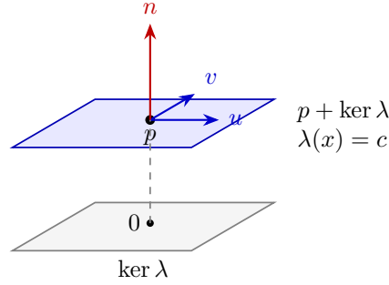
Figure 10.5: An affine plane and its parallel direction plane. The arrows u, v span the direction space; a Euclidean normal n represents the covector. Orthogonality is spatial, not an angle measured on this oblique drawing.
