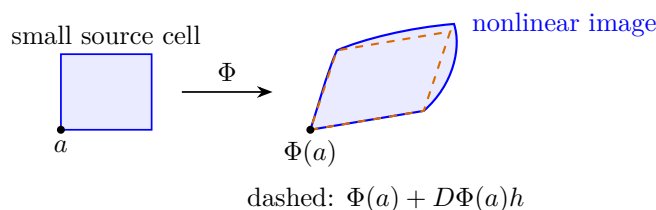
Figure 12.1: The derivative gives a first-order parallelogram model, not an exact image. Its area is |\det D\Phi(a)| times the source area; the nonlinear error is controlled as the cell shrinks.
