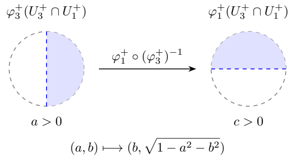
Figure 13.3: The same sphere overlap has two different coordinate images: a right half-disk and an upper half-disk. All displayed boundaries are excluded.
