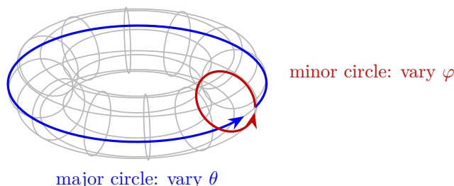
Figure 13.4: A wireframe of the embedded torus shows both independent circular directions. Hidden curves remain visible in this transparent schematic; periodic parameters are not a single global chart.
