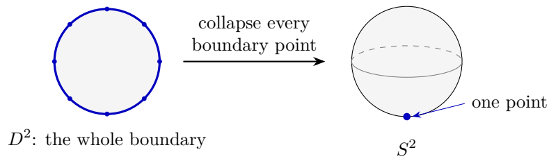
Figure C.2: The rule for D^2 / \partial D^2 : every marked boundary point belongs to one class, shown as the south pole; interior points remain distinct.
