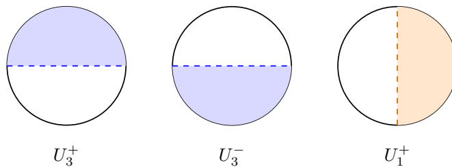
Figure 13.1: Front-view silhouettes of three hemisphere domains; dashed great-circle boundaries are excluded. Upper and lower hemispheres miss the equator, so side hemispheres are needed too. The six domains U_i^\pm cover the sphere and overlap.
