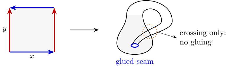
Figure C.6: Klein quotient: (0, y) \sim (1, y) and (x, 0) \sim (1 - x, 1) . The solid blue seam represents the joined circles; the dotted callout marks an incidental crossing of distinct sheets. The drawing in \mathbb{R}^3 is not an embedding. See Figure 13.8 for the deformation and Figure C.7 for the local disk at the corner class.
