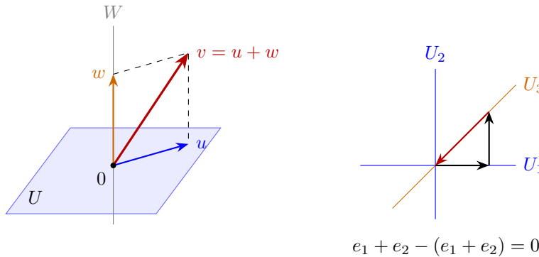
Figure 10.3: Left: a complementary plane and line give unique components; the drawing is oblique and does not assert orthogonality. Right: three lines can meet pairwise only at zero while admitting a nonzero relation.
