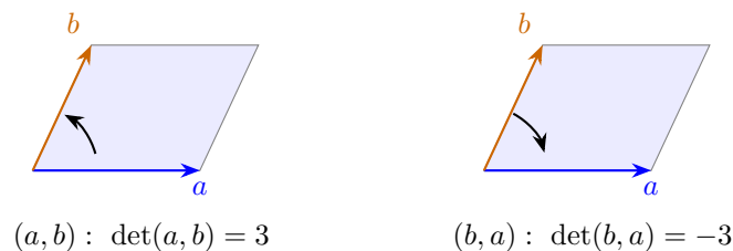
Figure 10.6: Swapping the ordered edges reverses orientation while preserving area. Here a = (2, 0) and b = (0.7, 1.5) ; both parallelograms have area 3.
