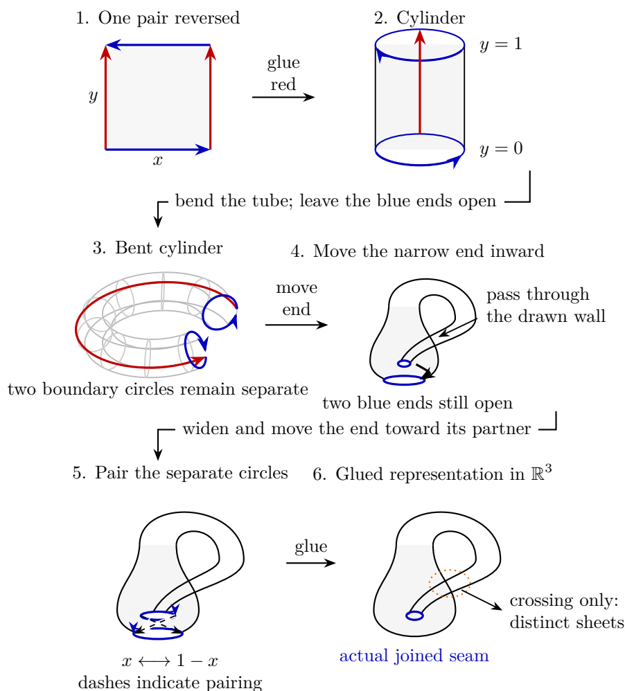
Figure 13.8: Klein-bottle gluing: (0, y) \sim (1, y) and (x, 0) \sim (1 - x, 1) . The bent cylinder keeps two boundary circles separate. Panels 4–5 move one end through the drawn wall, widen it, and display the reversed matching before identification in panel 6. The crossing in the \mathbb{R}^3 picture is not an additional identification. The abstract Klein bottle has ordinary disk neighborhoods and no self-intersection. Figure C.7 verifies the corner neighborhood.
