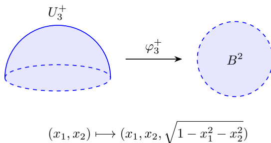
Figure 13.8: Deleting the third coordinate maps the open upper hemisphere to the open unit disk. The formula below reconstructs the hemisphere; both boundary circles are excluded.
