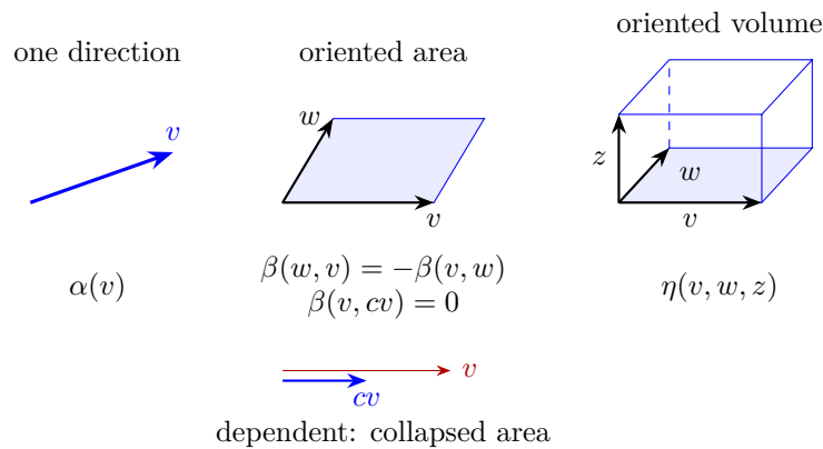
Figure 13.6: Alternating measurements progress from a vector to an ordered parallelogram to an ordered parallelepiped. Reordering two inputs reverses the sign; dependent inputs give zero.
