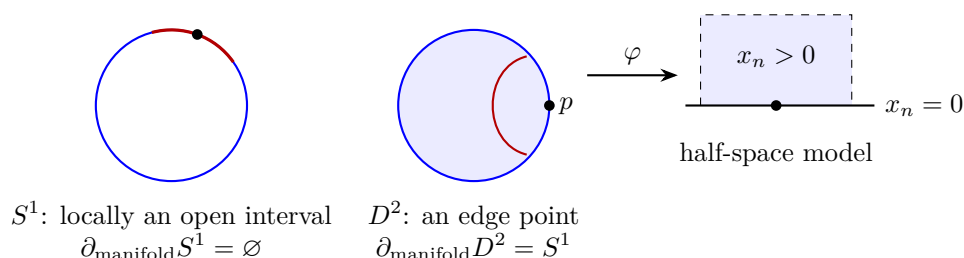
Figure 13.15: Manifold boundary is detected by local models, not by an ambient drawing. The whole circle is its boundary as a subset of the plane, but it has no manifold boundary. A disk edge flattens to the genuine face of a half-space.
