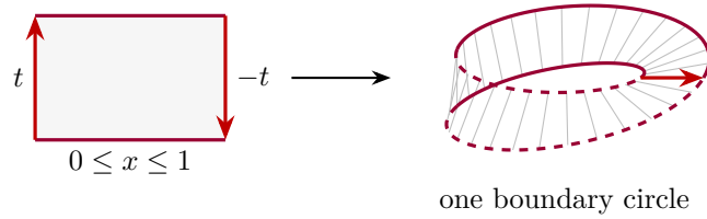
Figure C.4: Möbius quotient: (0, t) \sim (1, -t) . Opposite arrows encode the reversal. The two long edges join into the single emphasized boundary; dashes indicate its rear portions. Figure 13.13 shows the deformation, while Figure C.5 checks local charts.
