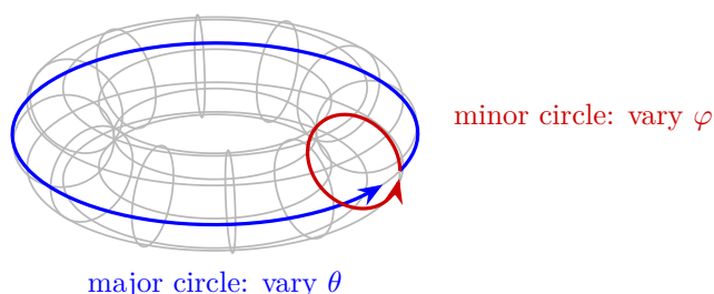
Figure 13.10: A wireframe of the embedded torus shows both independent circular directions. Hidden curves remain visible in this transparent schematic; periodic parameters are not a single global chart.
