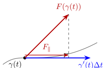
Figure 13.1: The dot product extracts the force component along displacement. The blue vector follows the velocity \gamma'(t) and approximates the actual short displacement along the curve.
