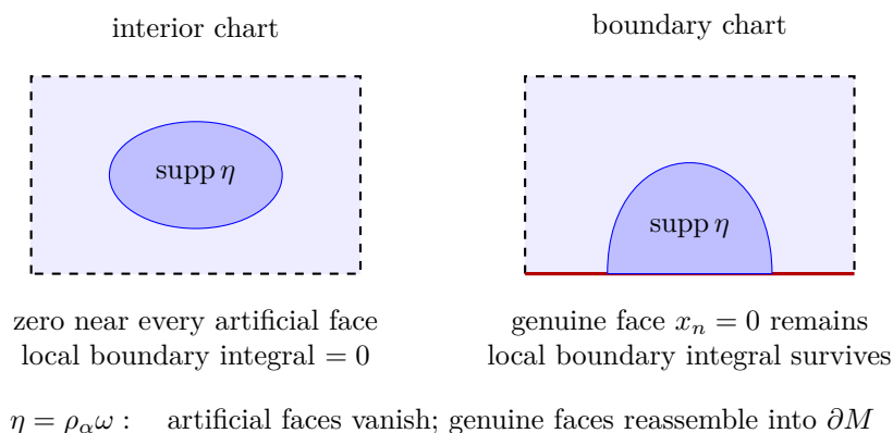
Figure 13.20: Local Stokes applied to a chart-supported form. Compact support removes artificial boundary terms. Smooth extension across the genuine face need not be zero, and this is exactly where the manifold boundary integral comes from.
