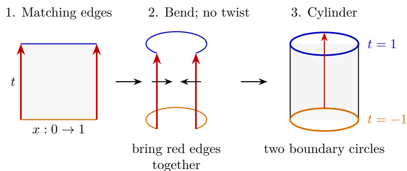
Figure 13.12: The cylinder glues (0, t) to (1, t) . The red arrows match without reversal; bending brings these edges together. The two unglued long edges close separately into the highlighted boundary circles.
