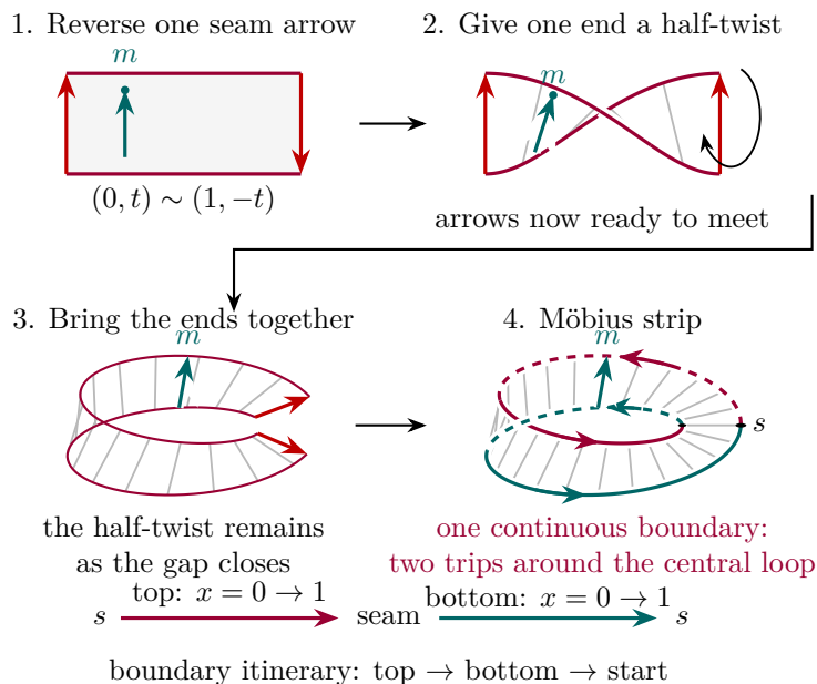
Figure 13.13: A half-twist implements the reversed seam rule. In the second panel the band is viewed obliquely through the twist; crossing strokes are projection effects. The marker m follows the same transverse segment. Dashed rear arcs and white gaps distinguish depth at projected crossings. Starting at s , the purple and teal portions trace one boundary: the edge that starts on top returns along the bottom before closing. See Section C.5 for the local charts.
