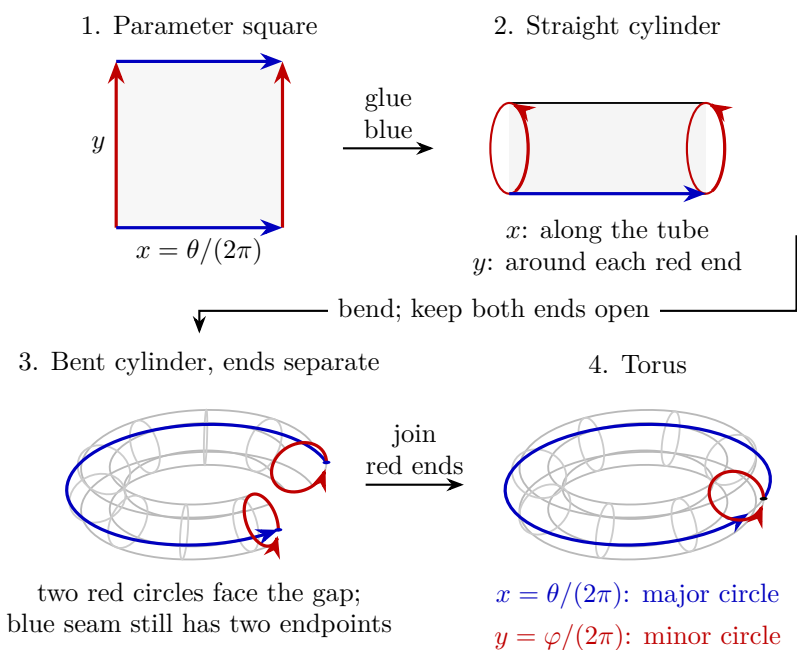
Figure 13.11: Square, straight cylinder, bent cylinder, and torus. Glue the blue edges first, making y circular while x runs along the tube. Bending preserves these directions. The two red end circles remain separate in panel 3; joining corresponding points closes the blue x -curve in panel 4. Either pair can be glued first, but this order agrees throughout with the angles in Figure 13.10 . The square is a fundamental domain, not a global chart; see Section C.4 .
