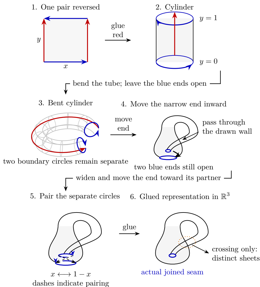
Figure 13.14: Klein-bottle gluing: (0, y) \sim (1, y) and (x, 0) \sim (1 - x, 1) . The bent cylinder keeps two boundary circles separate. Panels 4–5 move one end through the drawn wall, widen it, and display the reversed matching before identification in panel 6. The crossing in the \mathbb{R}^3 picture is not an additional identification. The abstract Klein bottle has ordinary disk neighborhoods and no self-intersection. Figure C.7 verifies the corner neighborhood.
