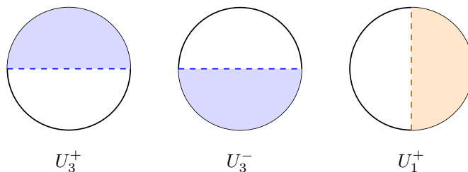
Figure 13.7: Front-view silhouettes of three hemisphere domains; dashed great-circle boundaries are excluded. Upper and lower hemispheres miss the equator, so side hemispheres are needed too. The six domains U_i^\pm cover the sphere and overlap.
