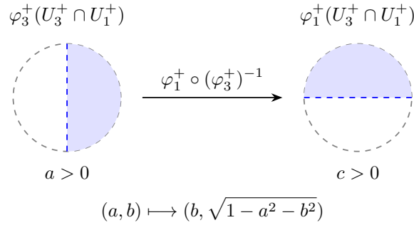
Figure 13.9: The same sphere overlap has two different coordinate images: a right half-disk and an upper half-disk. All displayed boundaries are excluded.
