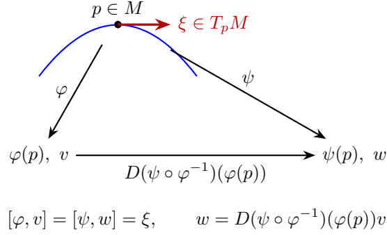
Figure 13.16: One intrinsic direction, two coordinate representatives. The transition derivative changes the vector column, while the equivalence class stays fixed. The arrows to coordinates are local chart descriptions.
