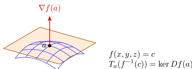
Figure 11.1: The regular level surface has tangent direction space \ker Df(a) . Its affine tangent plane passes through a ; the gradient is normal to it.
