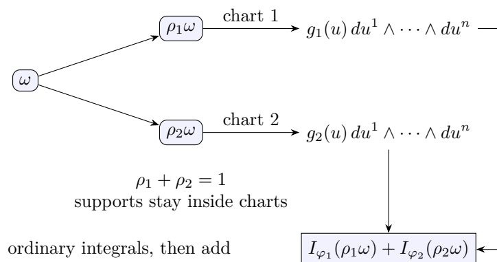
Figure 13.19: Two-chart integration: multiply by smooth weights, express each piece in coordinates, integrate its scalar coefficient, and add. The weights fade to zero near artificial chart edges. The same architecture works with any locally finite chart cover.
