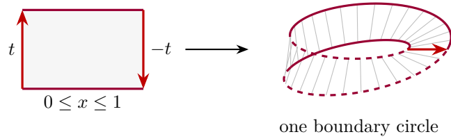
Figure C.4: Möbius quotient: (0, t) \sim (1, -t) . Opposite arrows encode the reversal. The two long edges join into the single emphasized boundary; dashes indicate its rear portions. Figure 13.17 shows the deformation, while Figure C.5 checks local charts.
