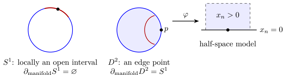
Figure 13.8: Manifold boundary is detected by local models, not by an ambient drawing. The whole circle is its boundary as a subset of the plane, but it has no manifold boundary. A disk edge flattens to the genuine face of a half-space.
