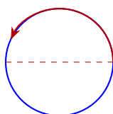
circle: paths, but missing chords
