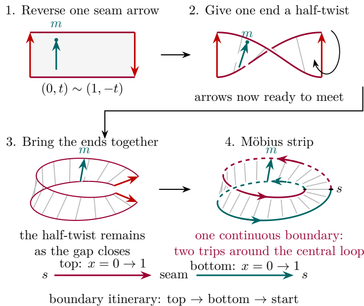
Figure 13.17: A half-twist implements the reversed seam rule. In the second panel the band is viewed obliquely through the twist; crossing strokes are projection effects. The marker m follows the same transverse segment. Dashed rear arcs and white gaps distinguish depth at projected crossings. Starting at s , the purple and teal portions trace one boundary: the edge that starts on top returns along the bottom before closing. See Section E.5 for the local charts.
