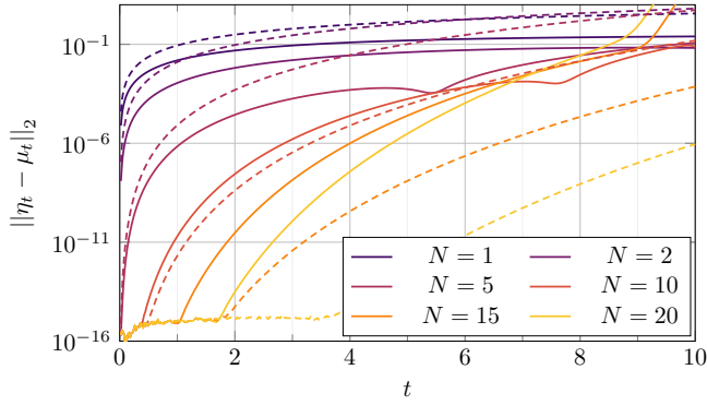
Figure 3: Error norm between the exact reduced evolution Rx_t and the approximated reduced evolution z_t for different values of the approximation order N . The dashed curves represent an approximation obtained by truncating the Taylor expansion of the exponential for different values of the truncation order N .
