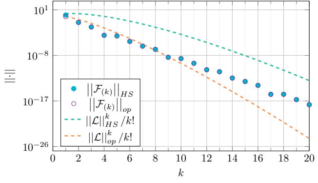
Figure 2: Operator and Hilbert-Schmidt norm of the first 20 F(k) terms (left) and of the first 50 E(k) terms when with N = 20 (right).
