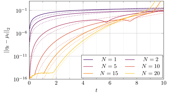
Figure 3: Error norm between the exact reduced evolution \eta_t and the approximated reduced evolution \mu_t for different values of the approximation order N . The dotted curves represent a curve-fit for the function \alpha t^{N+1} for different values of N .
