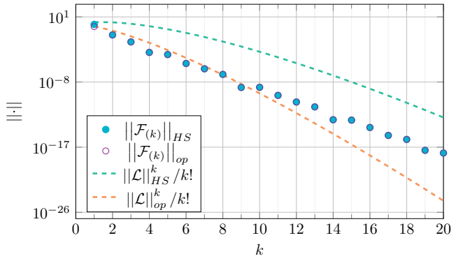
Figure 2: Operator and Hilbert-Schmidt norm of the first 20 \mathcal{F}_{(k)} terms (left) and of the first 50 \mathcal{E}_{(k)} terms when with N = 20 (right).
