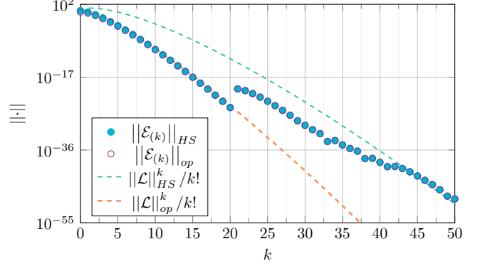
Figure 2: Operator and Hilbert-Schmidt norm of the first 20 \mathcal{F}_{(k)} terms (left) and of the first 50 \mathcal{E}_{(k)} terms when with N = 20 (right).
