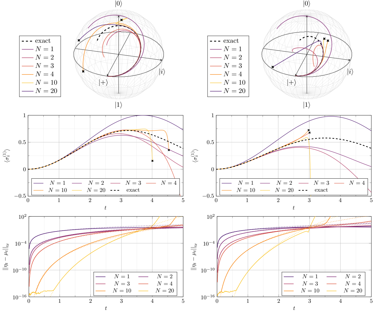
Figure 4. Simulations of the dissipative central spin model in the purely Hamiltonian setting ( \Lambda = 0 ) on the left and in the dissipative setting ( \Lambda = 0.8 ) on the right. The exact evolution and various degrees of approximations ( N = 1, 2, 3, 4, 10, 20 ) are shown in each figure. The first row shows the trajectory of the state of the central state \rho_S in the Bloch sphere; the second row shows the magnetization of the central spin in the \sigma_z direction versus time; the third row shows the trace norm error between the exact trajectory \eta_t and the reduced one \mu_t , i.e. \|\eta_t - \mu_t\|_{\text{tr}} versus time for different values of the approximation N and with dotted curve representing a fitted \alpha t^{N+1} curve. The black crosses denote points where the evolved state \mu_t exits the set of density operators.
