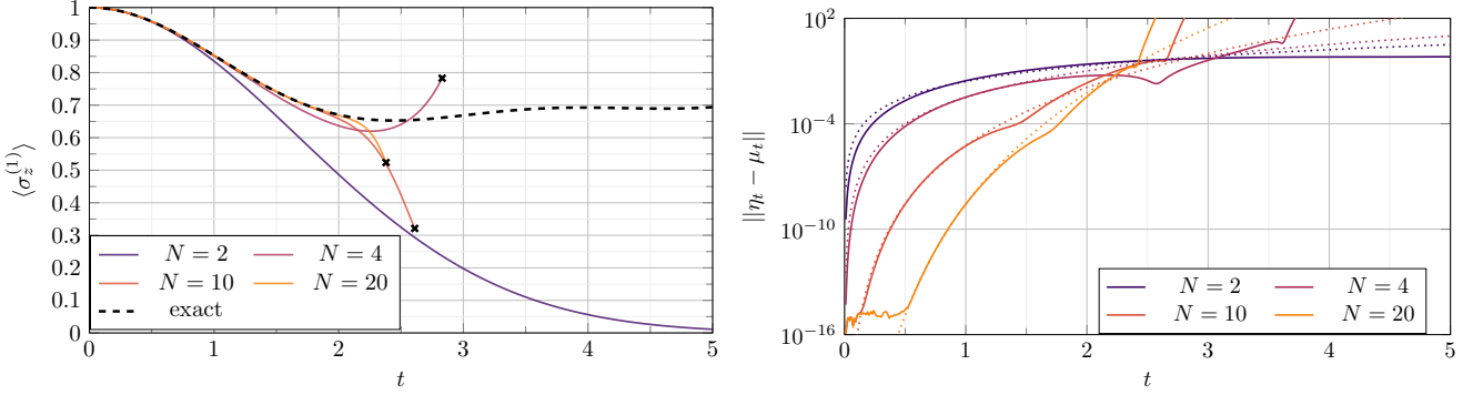
Figure 5. Simulation of the Ising spin chain. Magnetization of the first spin of the chain \langle \sigma_z^{(1)} \rangle versus time on the left and the error norm \|\eta_t - \mu_t\|_2 versus time on the right. Various approximation's degrees N = 2, 4, 10, 20 are shown in each figure. The black crosses denote the points where the evolved state \mu_t exits the n -dimensional simplex, i.e. \mu_t is no longer a probability distribution while the dotted curves on the right again represent fitted curves of \alpha t^{N+1} .
