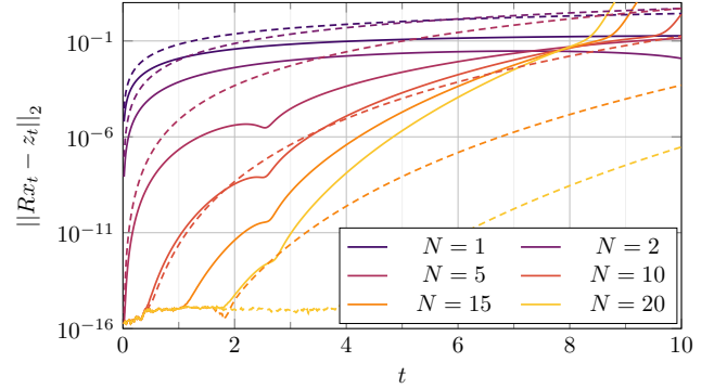
Figure 3. The continuous lines represent the error norm between the exact reduced evolution Rx_t and the approximated reduced evolution z_t for different values of the approximation order N . The dashed curves represent an approximation obtained by truncating the Taylor expansion of the exponential for different values of the truncation order N .
