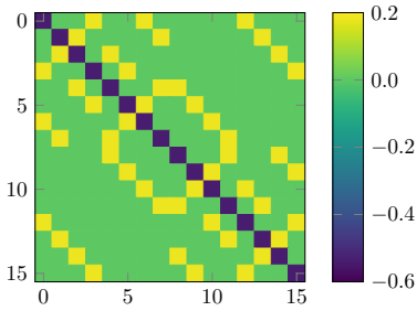
Figure 6. Graphical representation of the term \mathcal{F}_{(2)} for the time-dependent generator \mathcal{F}_t of the Ising spin chain model.
