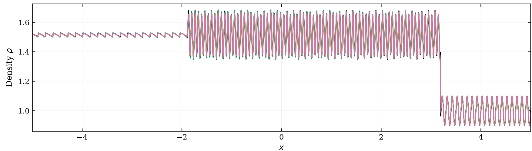
Resolved entropy-wave train
