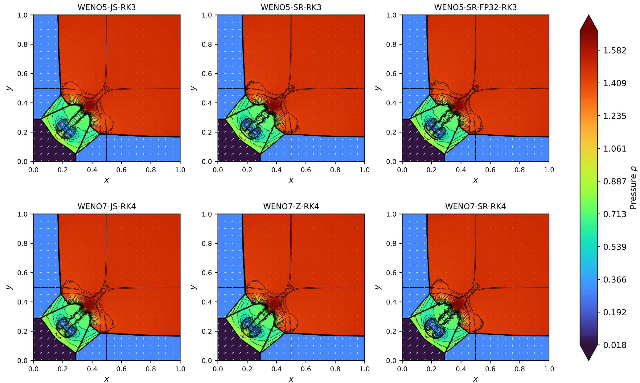
Two-dimensional Riemann configuration C.3 at t = 0.50
