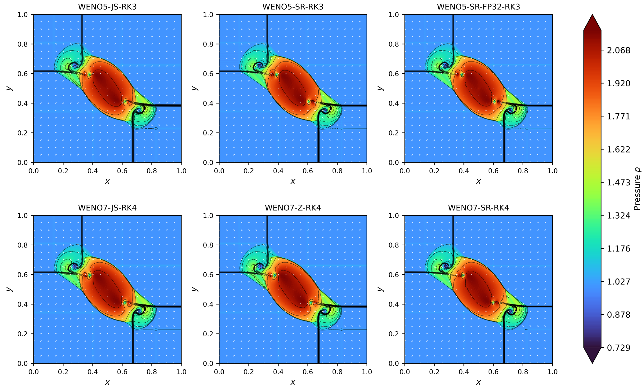
Two-dimensional Riemann configuration C.5 at t = 0.23
