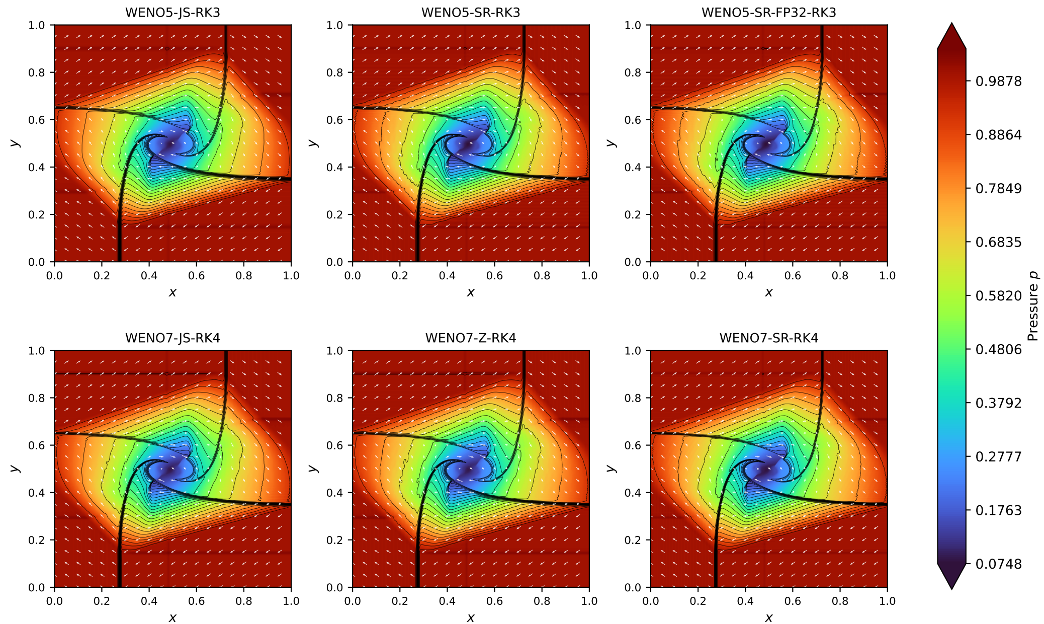
Two-dimensional Riemann configuration C.6 at t = 0.30
