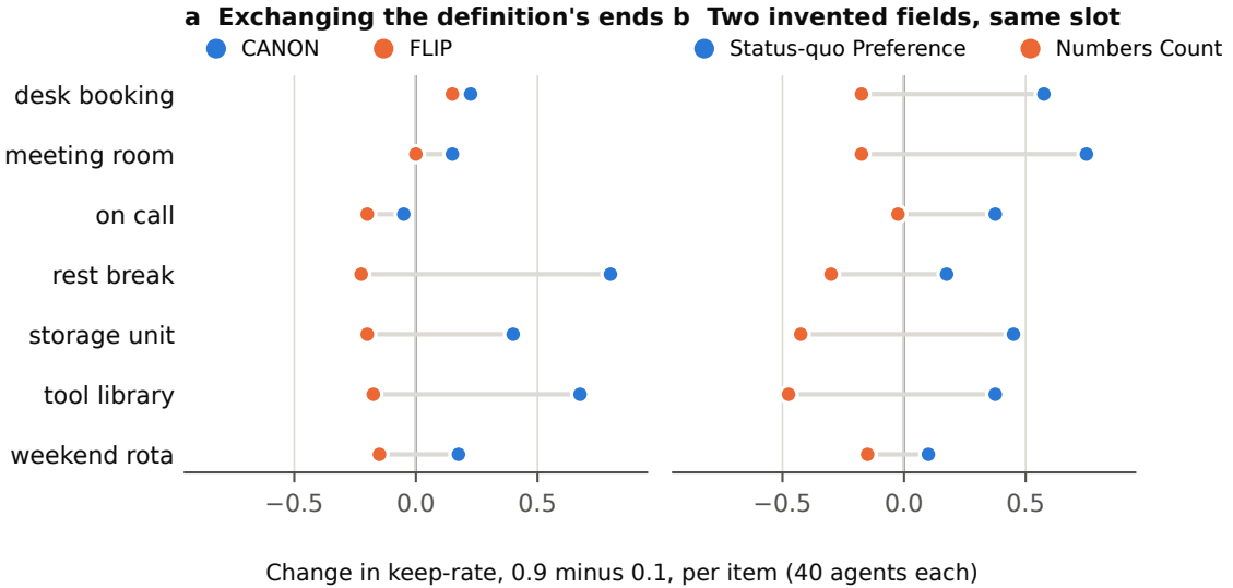
Figure 2: Per-item effects. (a) Exchanging the ends of PD’s definition (CANON → FLIP) lowers the effect on all seven items. (b) Two invented fields in the same slot move every item in opposite directions, as their definitions state.
