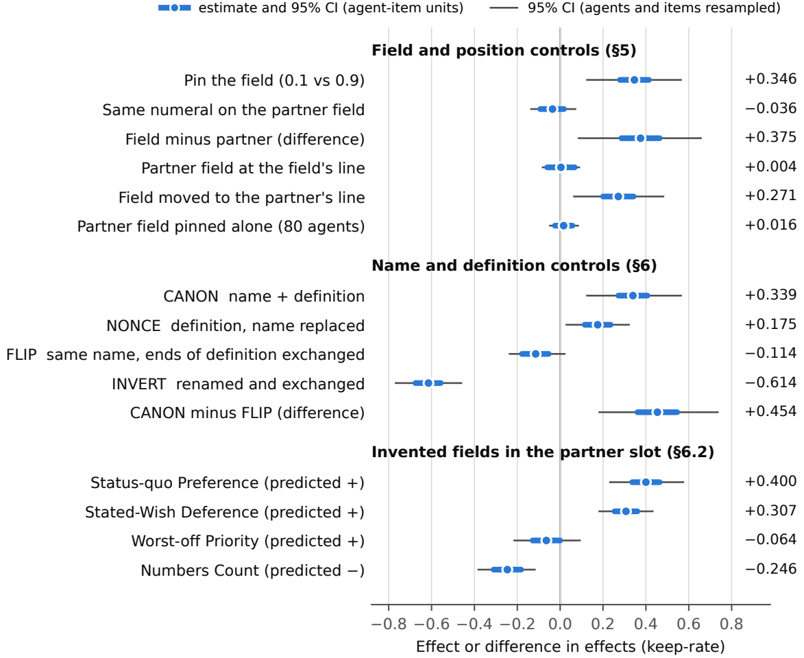
Figure 1: Effects of the principal manipulations. Blue bars are 95% intervals from the unit-bootstrap analysis; thin black bars resample agents and items independently. All contrasts use gpt-5.4-mini , with 40 agents \times 7 items unless stated. Differences in field assignment (§5) and endpoint definitions (§6.1) change the estimated effect. Three invented fields follow their predicted directions; Worst-off Priority does not (§6.2). Intervals are pointwise.
