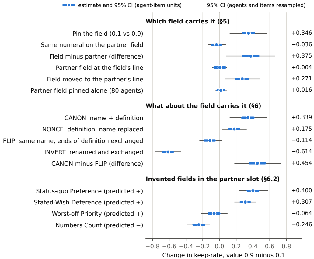
Figure 1: Effects of the principal manipulations. Thick bars are 95% intervals over agent-item units (the prespecified analysis); thin bars resample agents and items independently. All contrasts use gpt-5.4-mini , with 40 agents \times 7 items unless stated. Moving the numeral off the field, or putting it at the field's line on the partner, removes the effect (§5). Editing the field's definition sets the effect's direction (§6.1). Invented fields follow their own definitions (§6.2).
