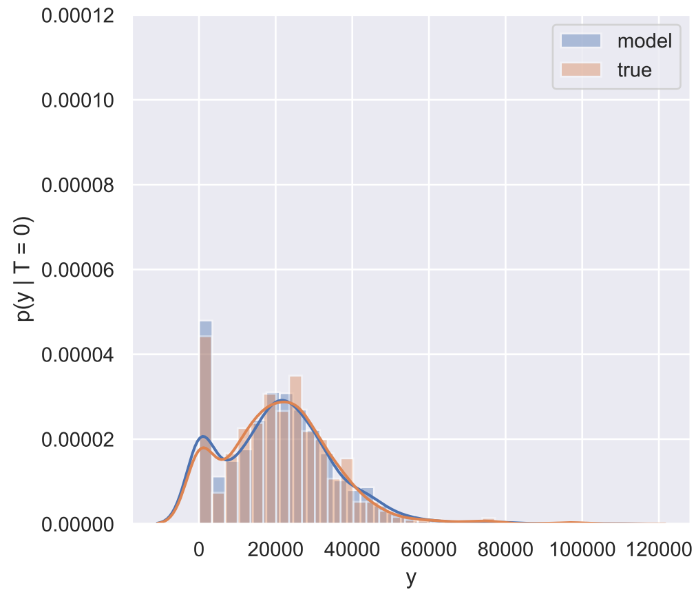
TarNet Joint Kernel Density Estimate Plots
