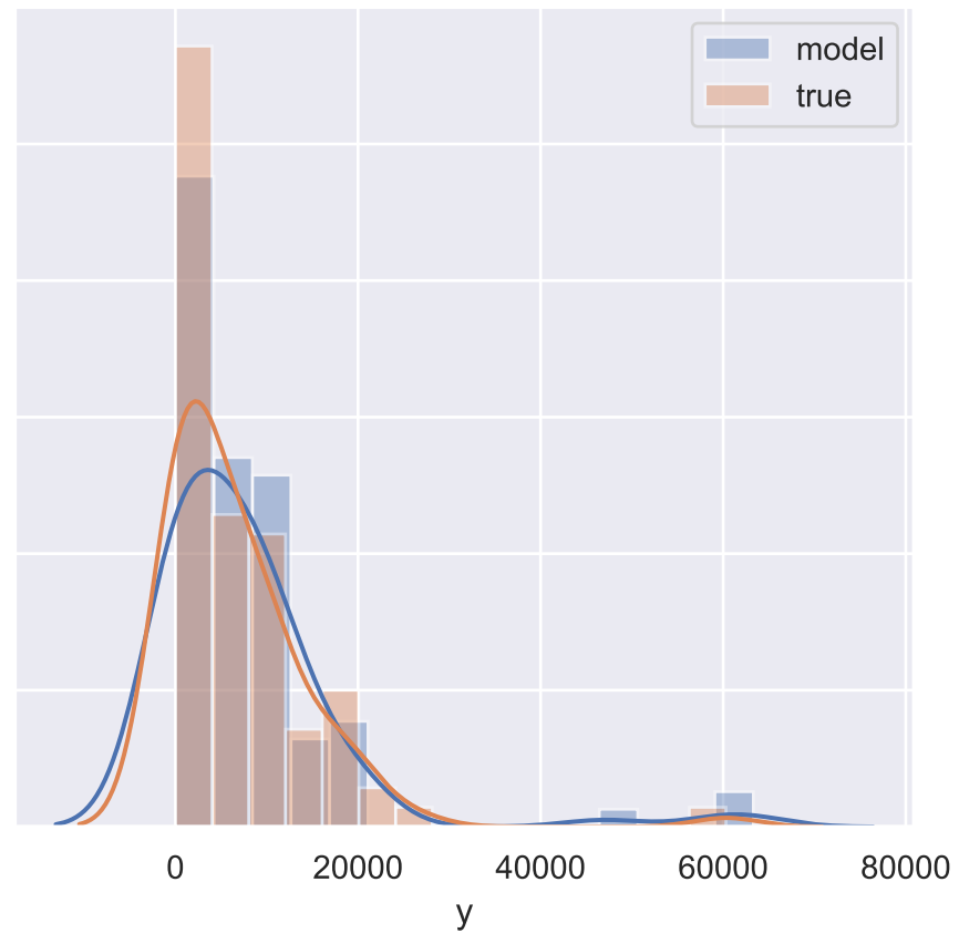
TarNet Joint Kernel Density Estimate Plots
