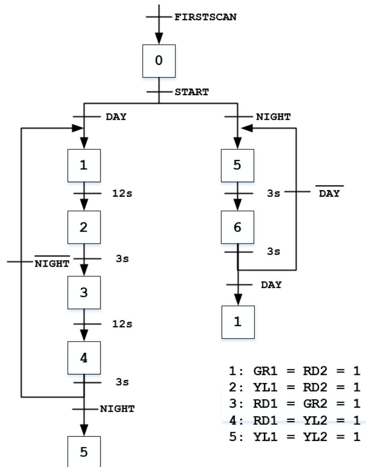
Figure 2: The Grafcet
