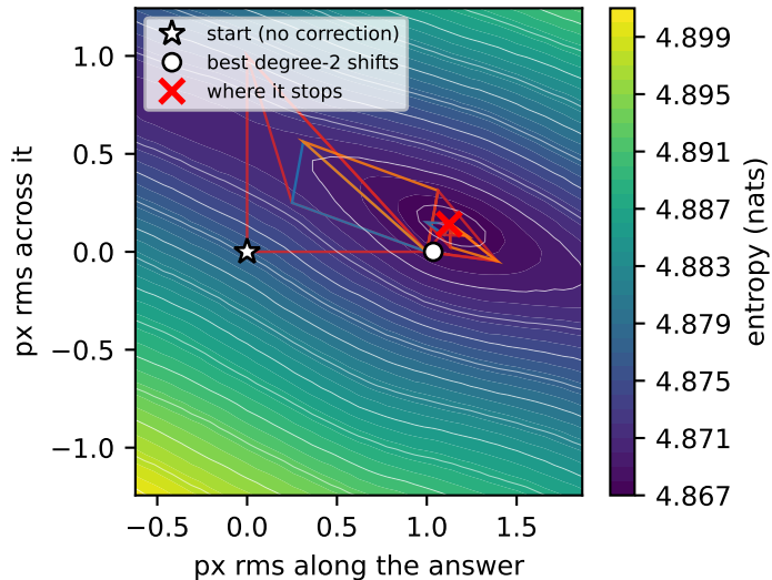
31 simplices on the real objective (a 2-D slice of the degree-2 stage)
