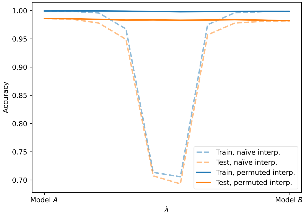
Accuracy between the two models (epoch 49)
