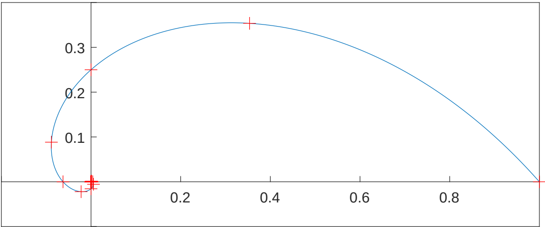
図 1 \left(\frac{\sqrt{2}}{4}(1+i)\right)^n ( 0 \leq n \leq 32 )
