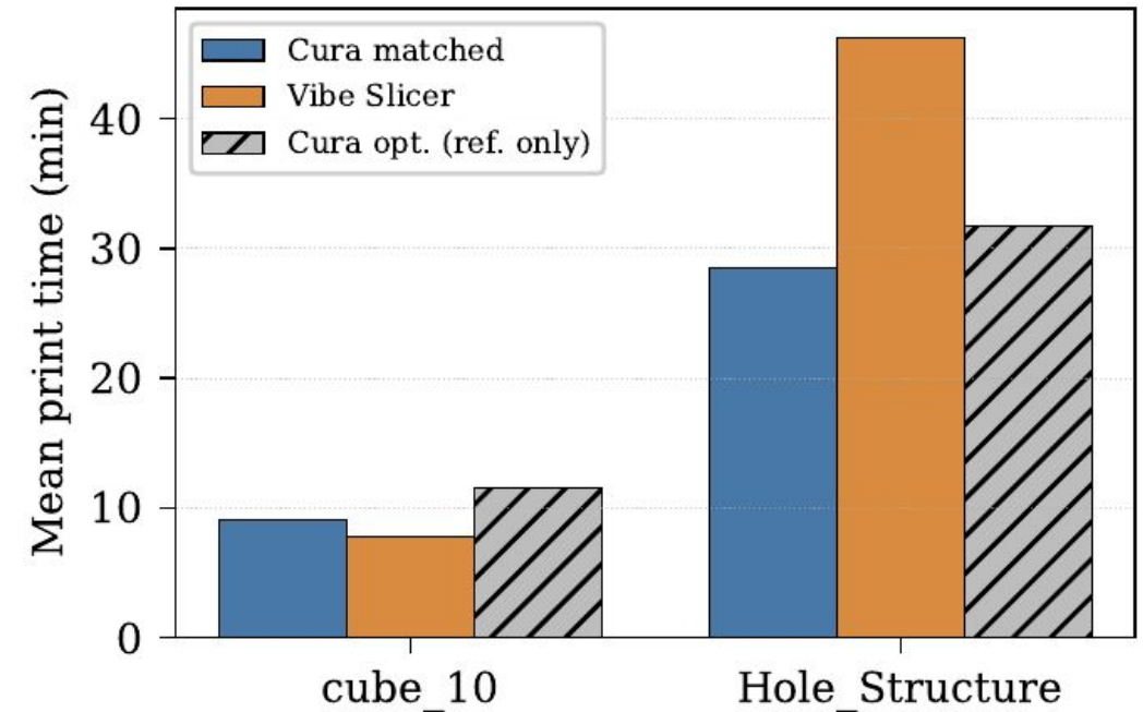
Mean print time per object
