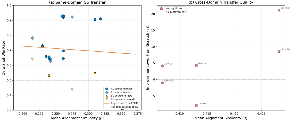
Figure 6: Transfer quality analysis. (a) Same-domain Go transfers: RL-trained sources (blue) consistently outperform BC sources (orange), regardless of alignment similarity. (b) Cross-domain transfers: 4 of 6 pairs show positive improvement, though high variance prevents significance.
