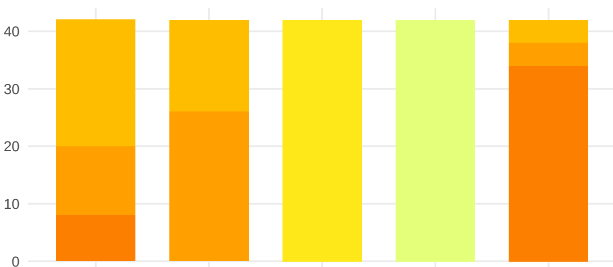
Serialize
