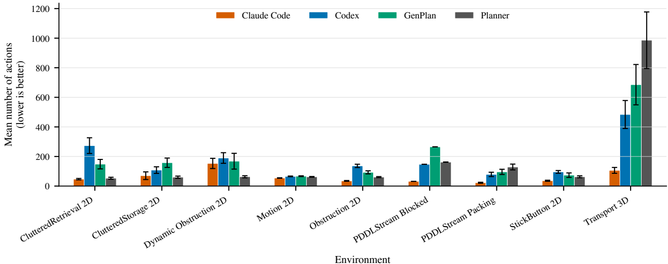
Actions on jointly solved held-out episodes
