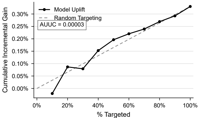
Qini curve (incentive_250_loyalty_pts)
