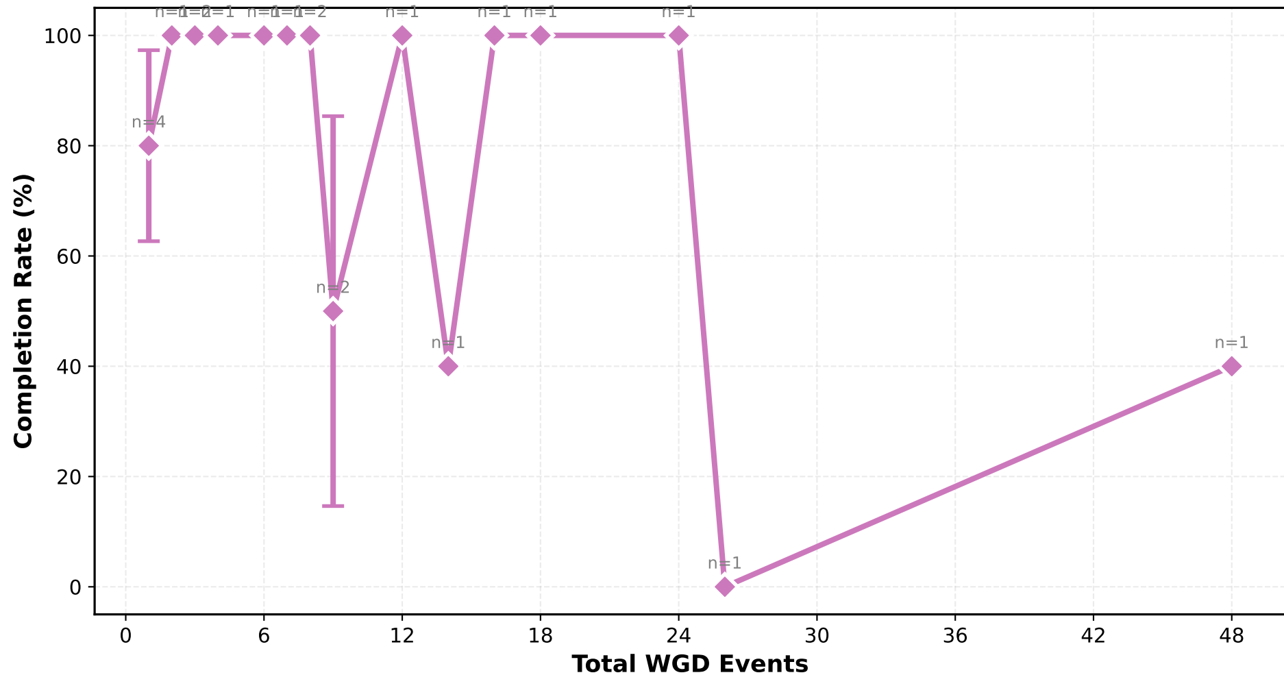
polyphest_p90 Completion Rate vs Total WGD Events (ILS Low)
