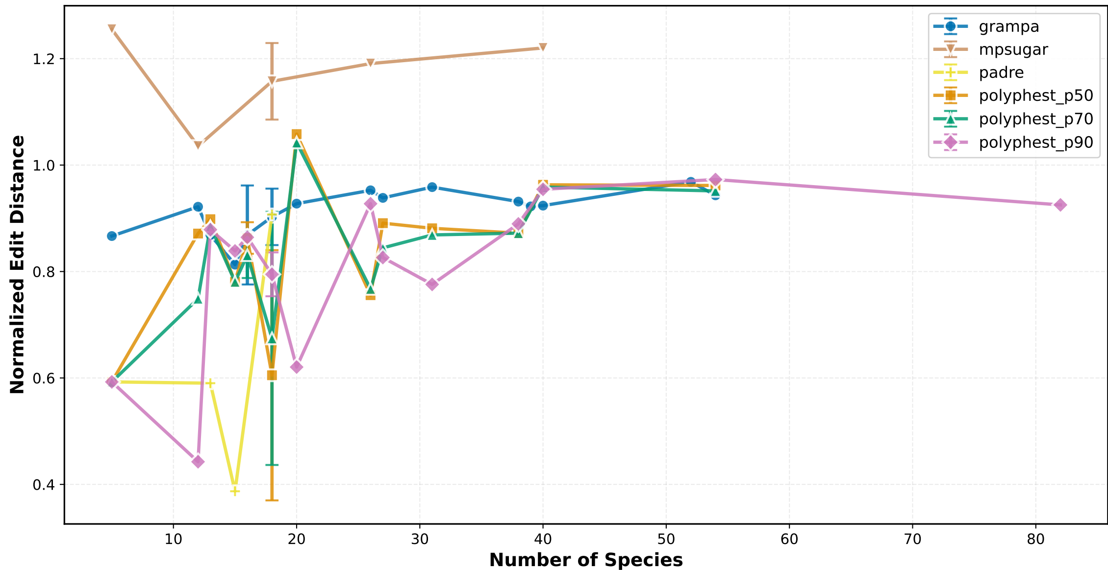
Normalized Edit Distance vs Number of Species ILS Low
