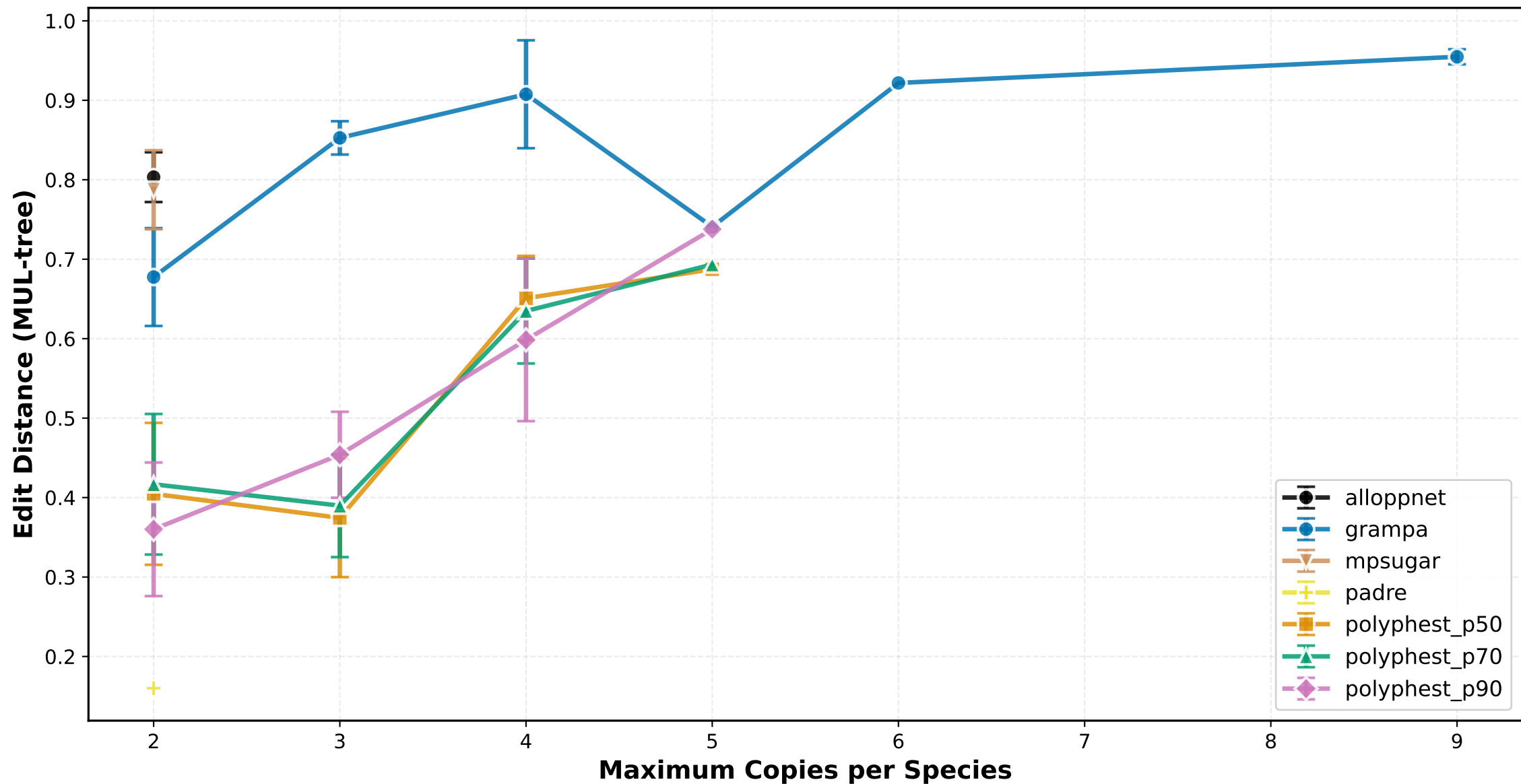
Edit Distance (MUL-tree) vs Maximum Copies per Species ILS Medium
