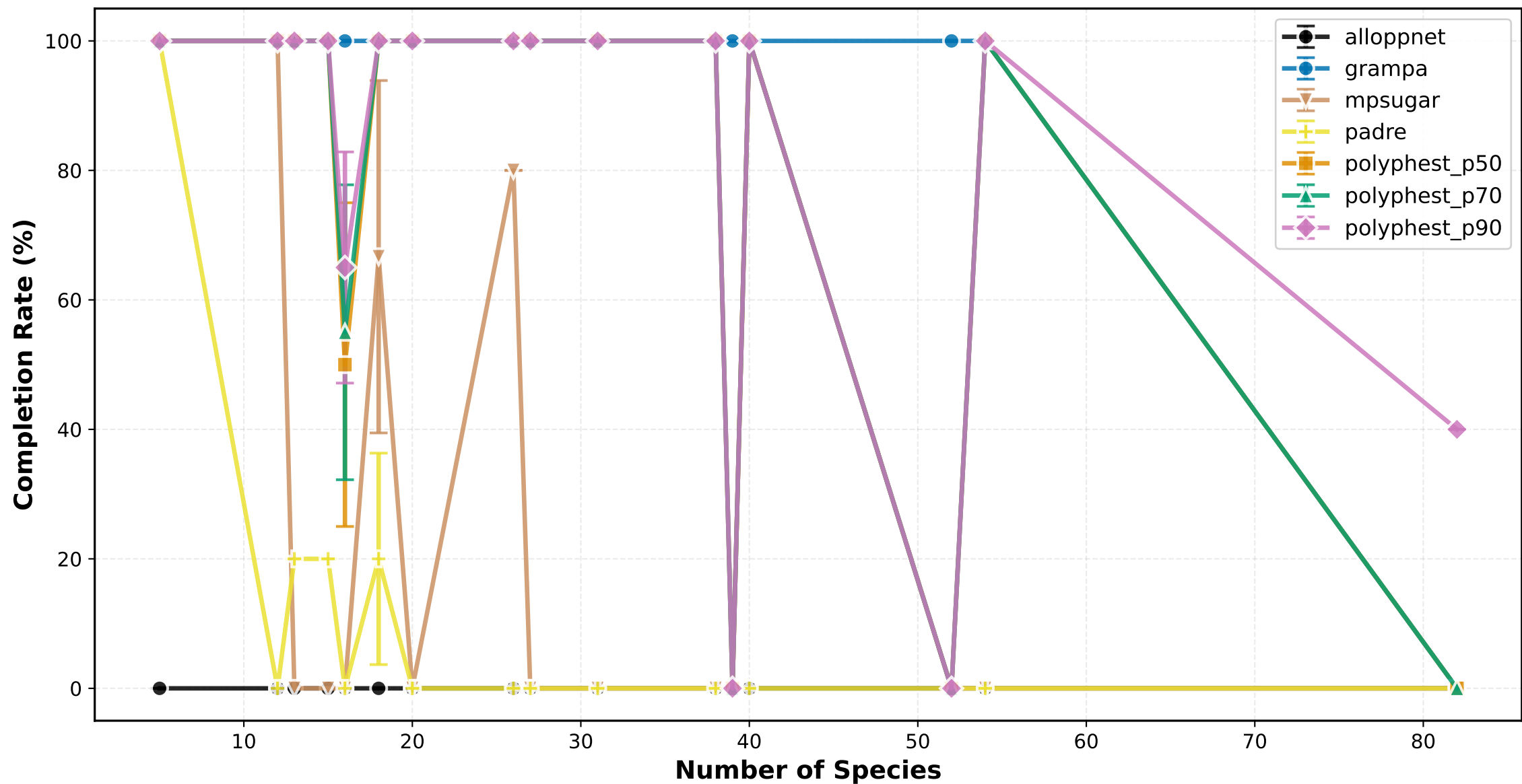
Completion Rate vs Number of Species ILS Low
