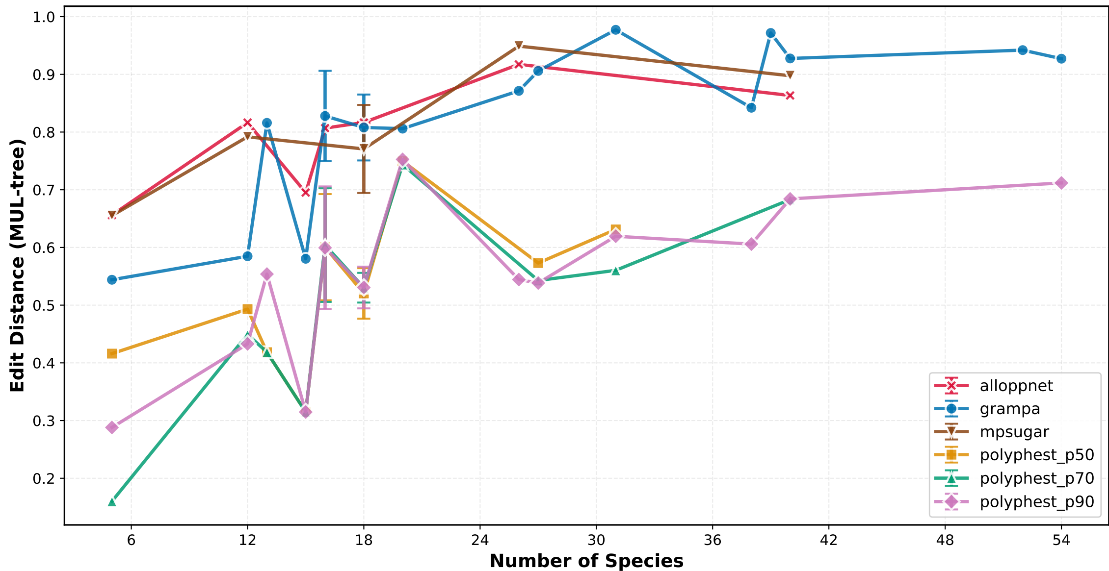
Edit Distance (MUL-tree) vs Number of Species ILS High
