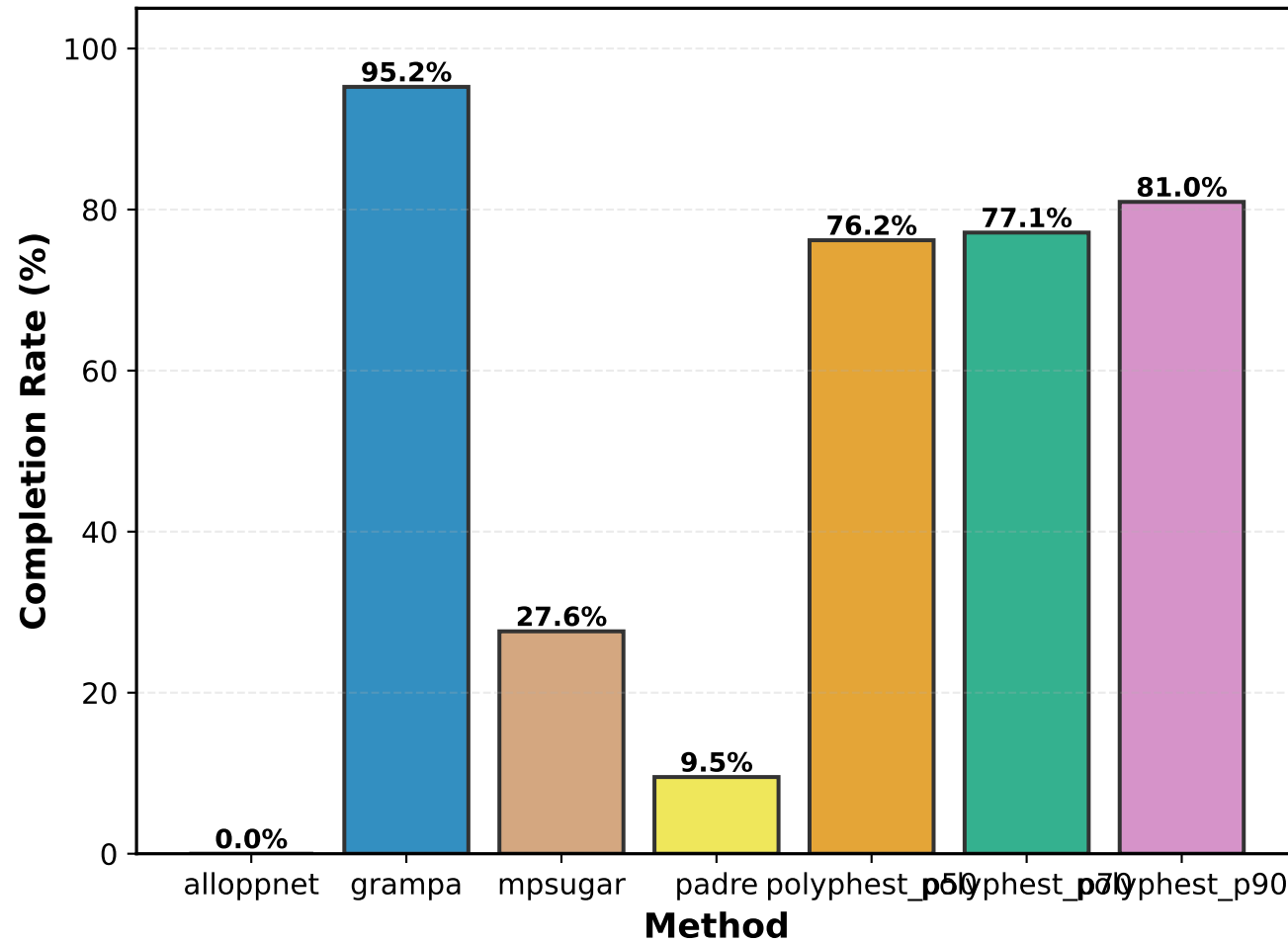
Completion Rate by Method
