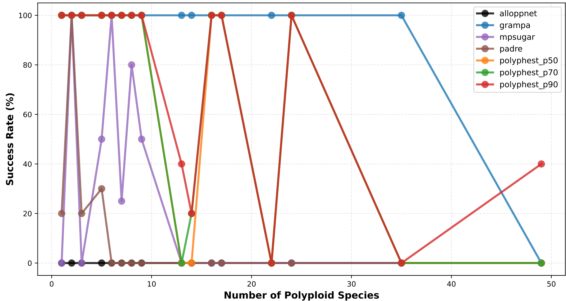
Success Rate vs Number of Polyploids conf_ils_low_10M (ILS low)
