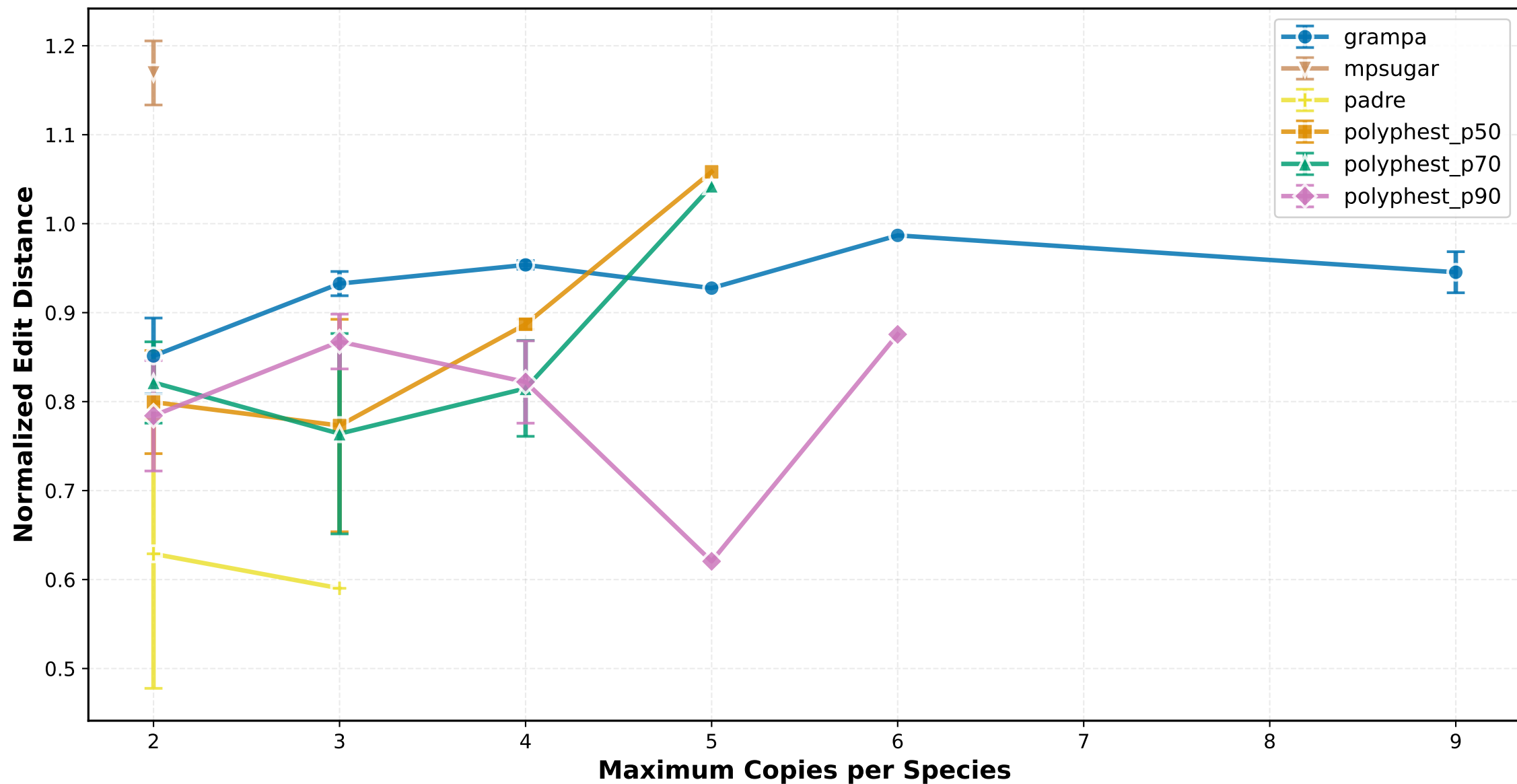
Normalized Edit Distance vs Maximum Copies per Species ILS Low
