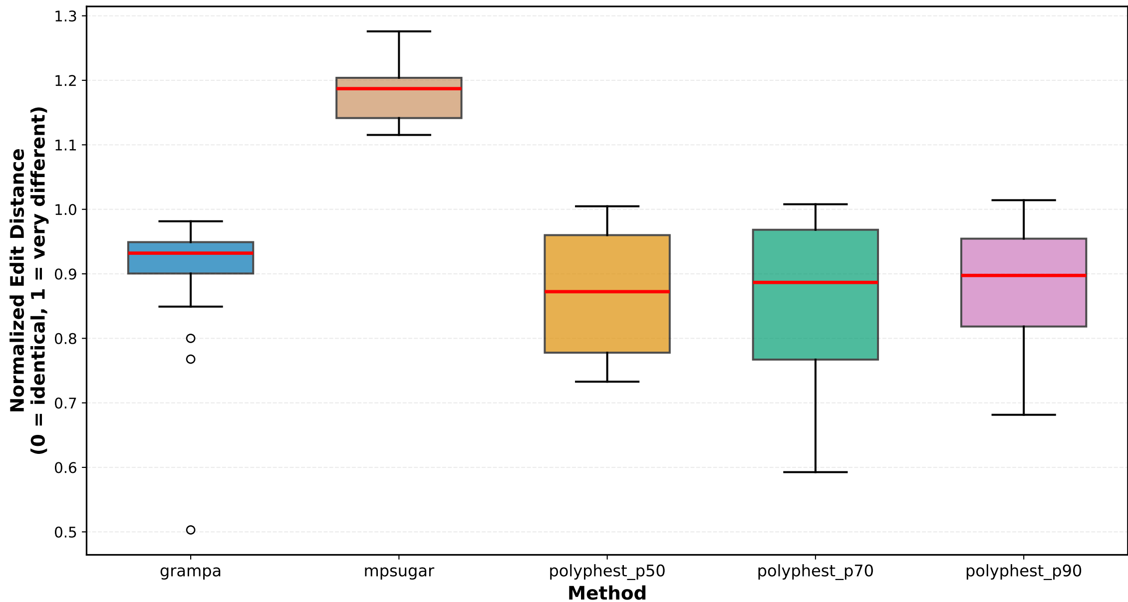
Edit Distance Distribution (ILS High)
