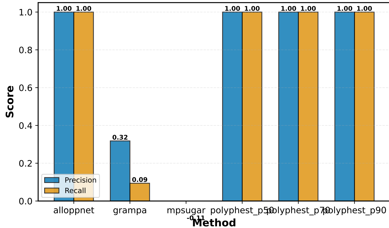
Polyploid Identification: Precision vs Recall
