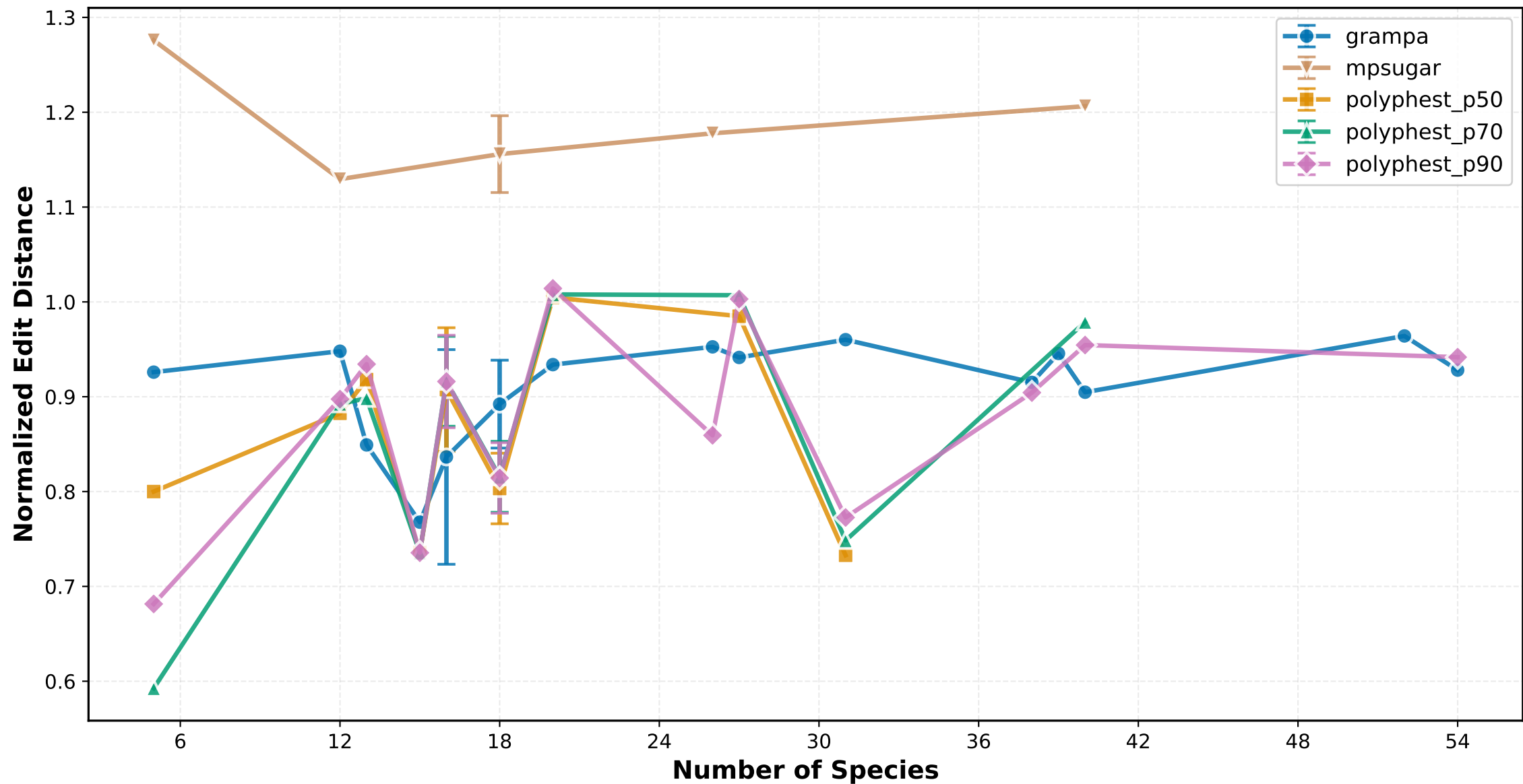
Normalized Edit Distance vs Number of Species ILS High
