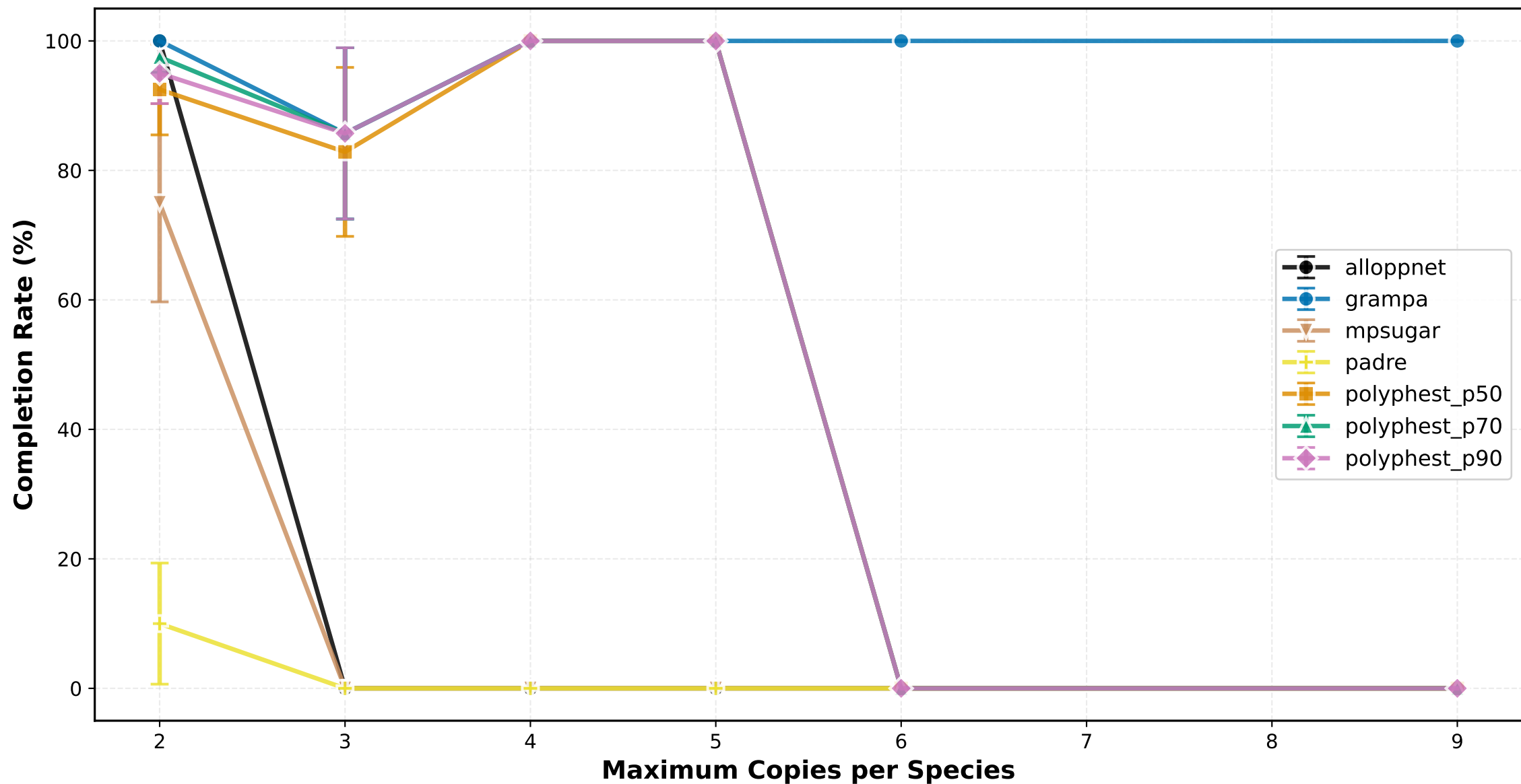
Completion Rate vs Maximum Copies per Species ILS Medium
