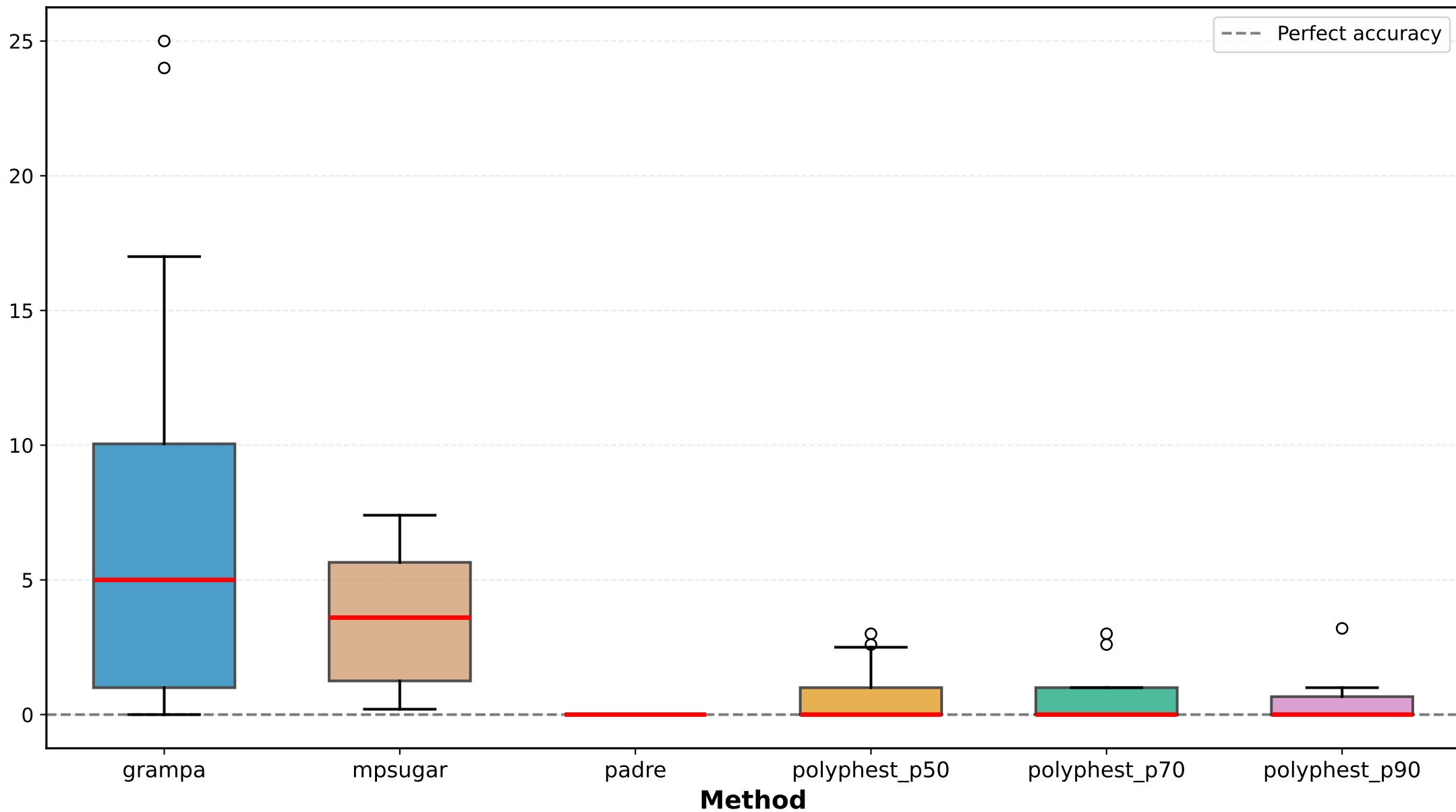
Reticulation Count Error Distribution (ILS Medium)
