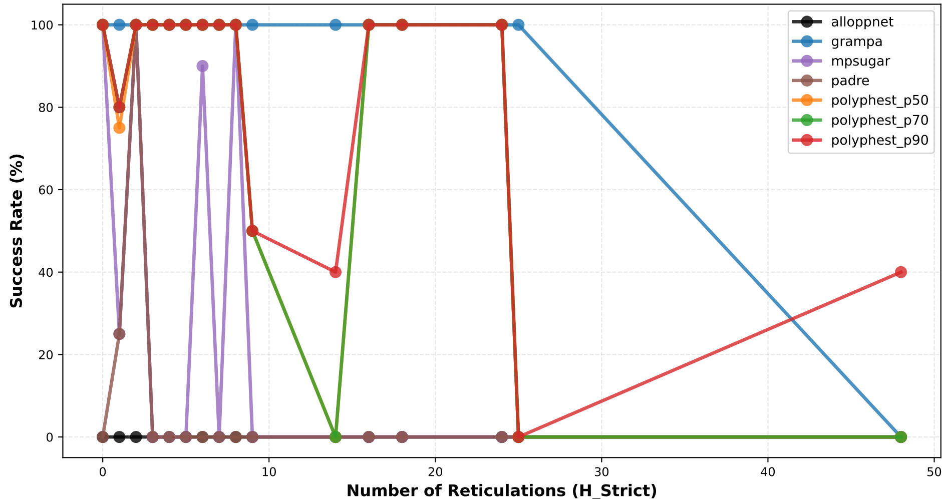
Success Rate vs Number of Reticulations conf_ils_low_10M (ILS low)
