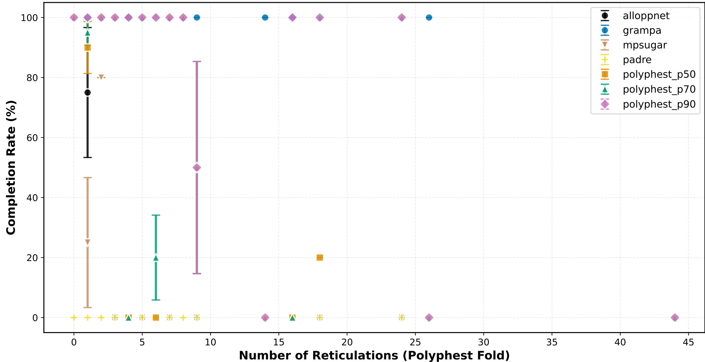
Completion Rate vs Number of Reticulations (Polyphest Fold) ILS High
