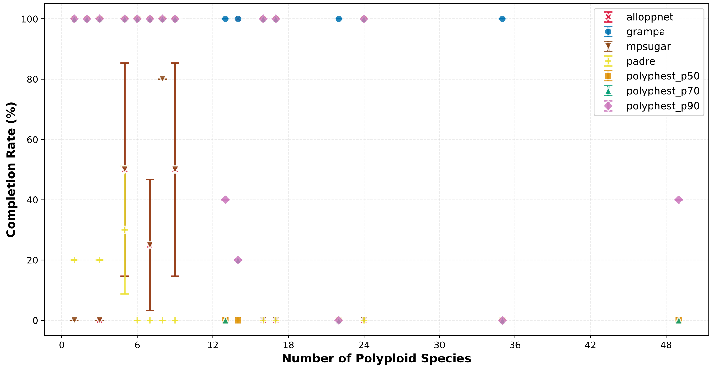
Completion Rate vs Number of Polyploid Species ILS Low
