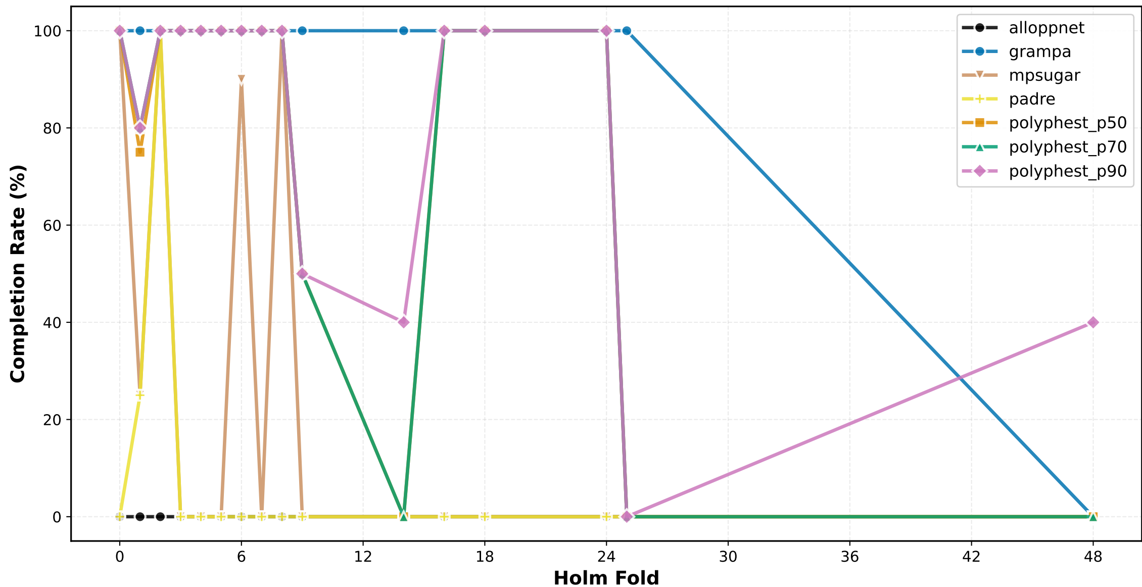
Completion Rate vs Holm Fold ILS Low
