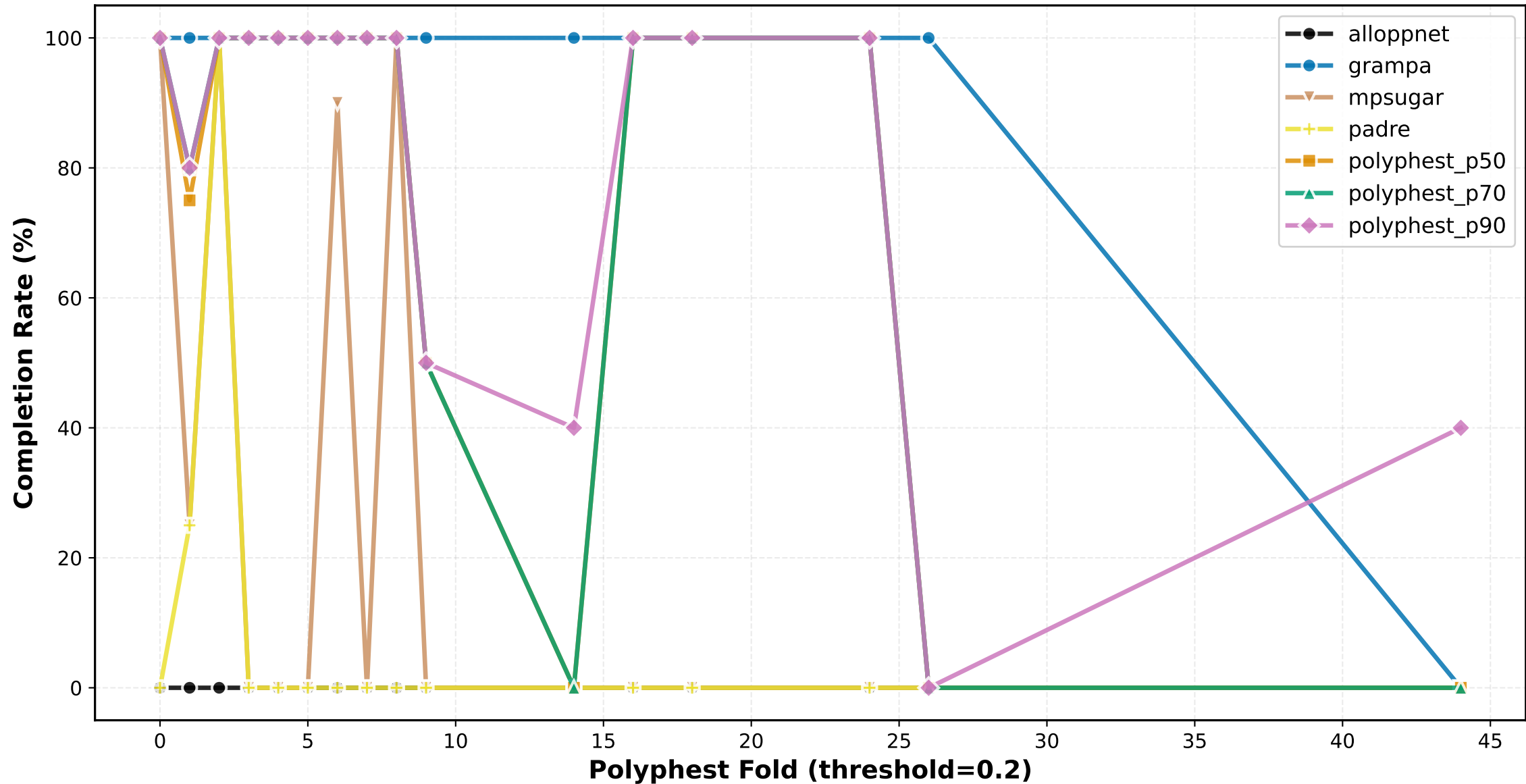
Completion Rate vs Polyphest Fold (threshold=0.2) ILS Low
