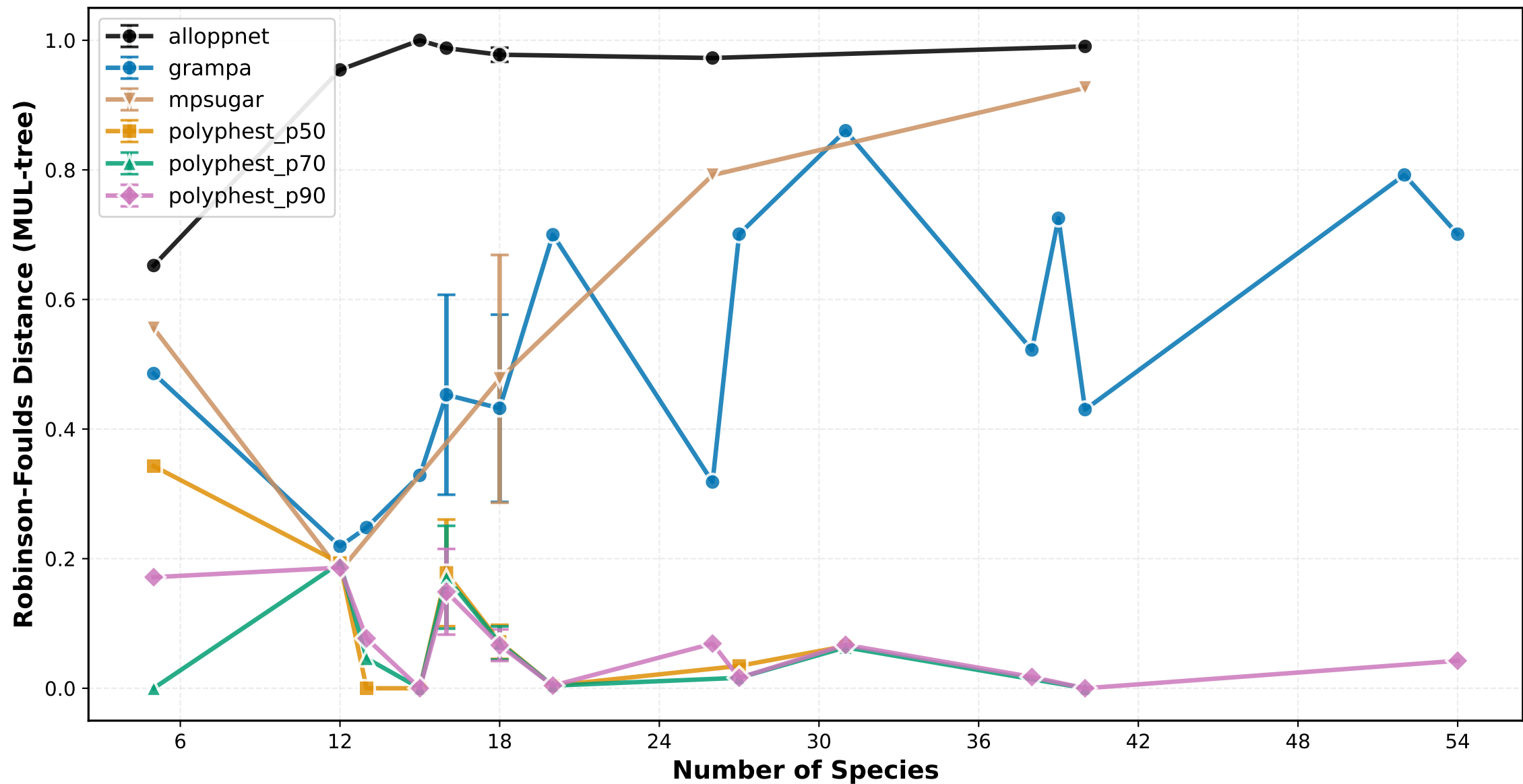
Robinson-Foulds Distance (MUL-tree) vs Number of Species ILS High
