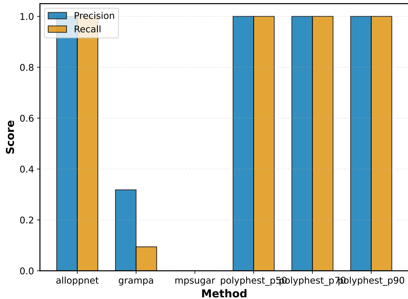
Polyploid Identification: Precision vs Recall
