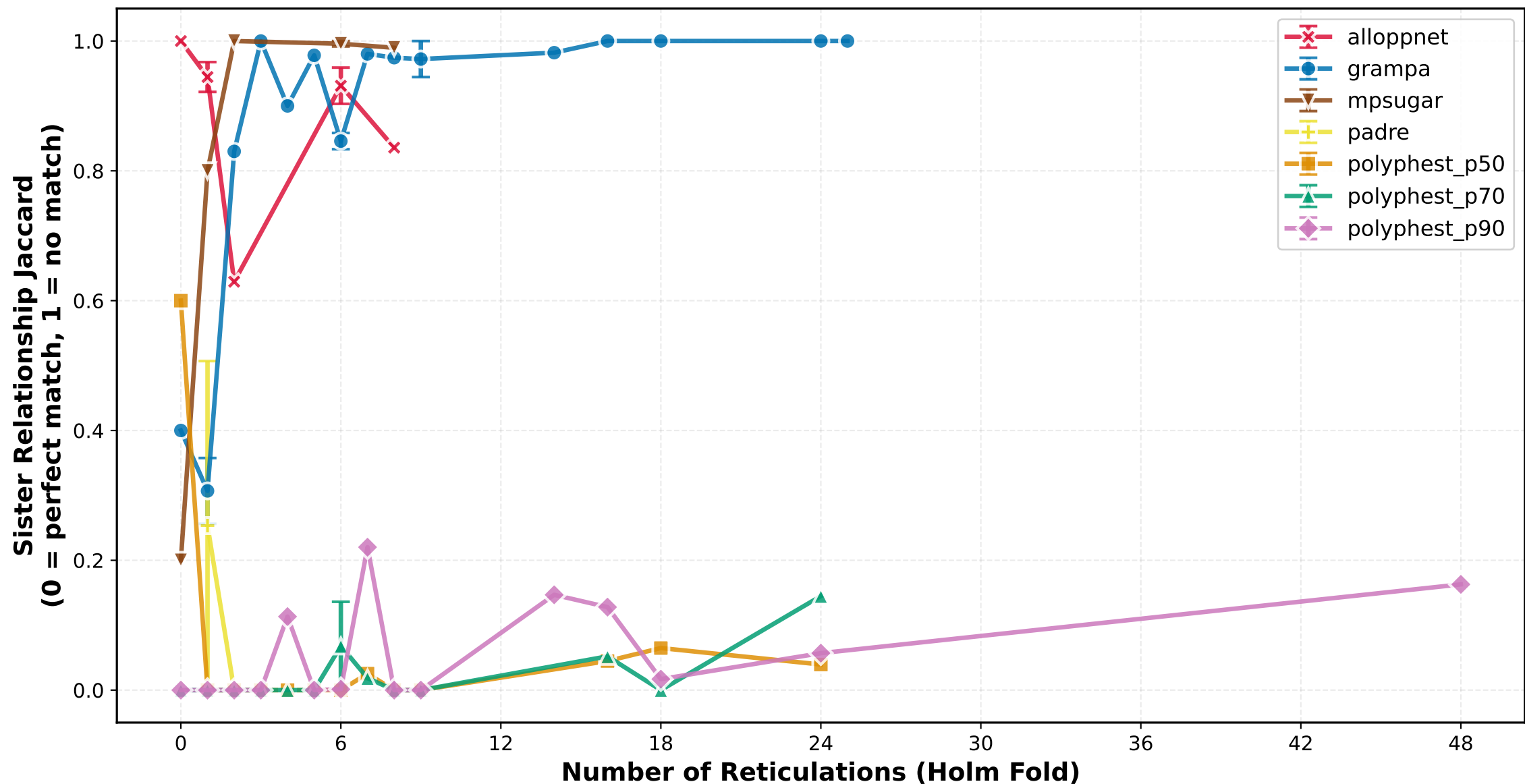
Sister Relationship Jaccard vs Number of Reticulations (Holm Fold)
