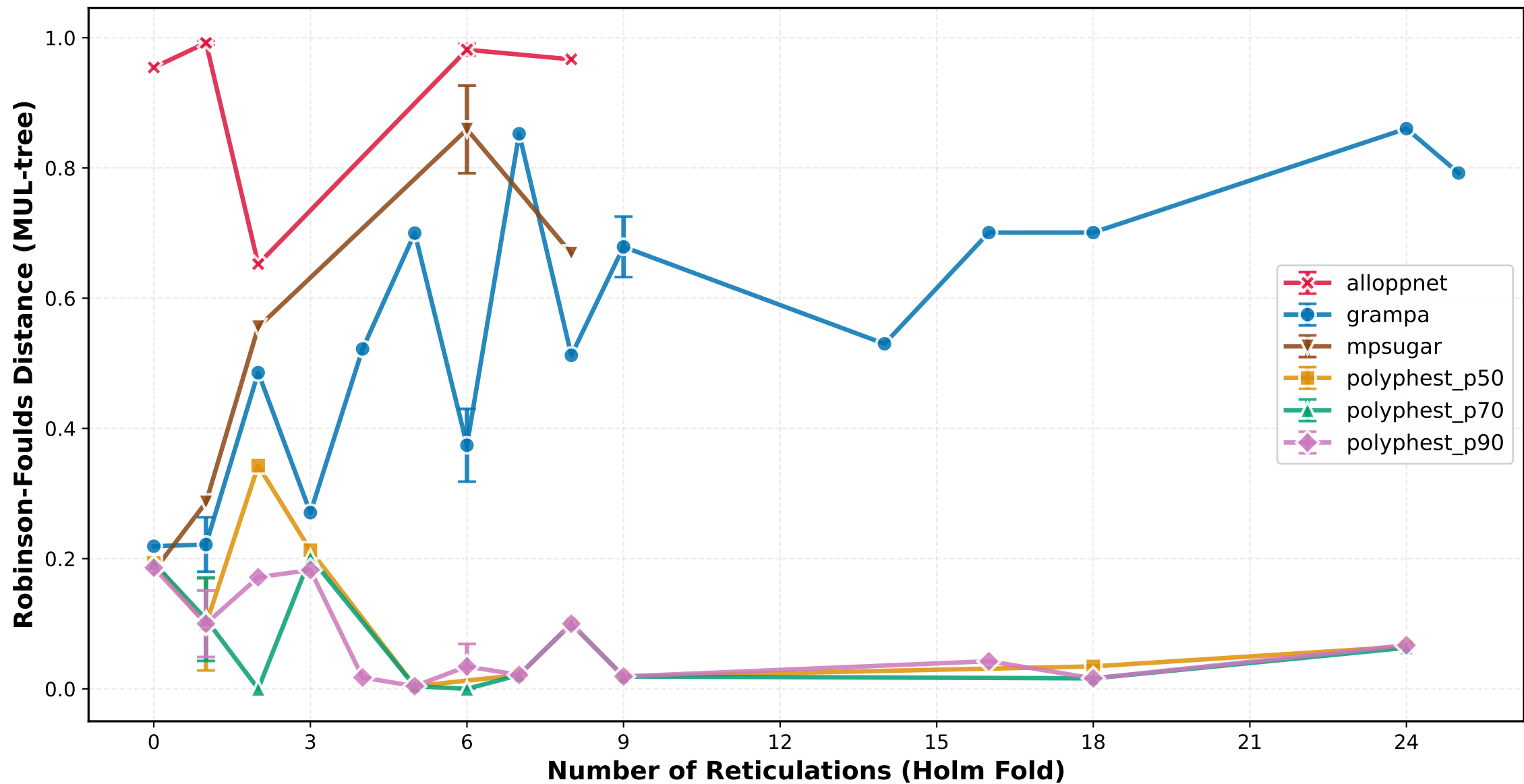
Robinson-Foulds Distance (MUL-tree) vs Number of Reticulations (Holm Fold) ILS High
