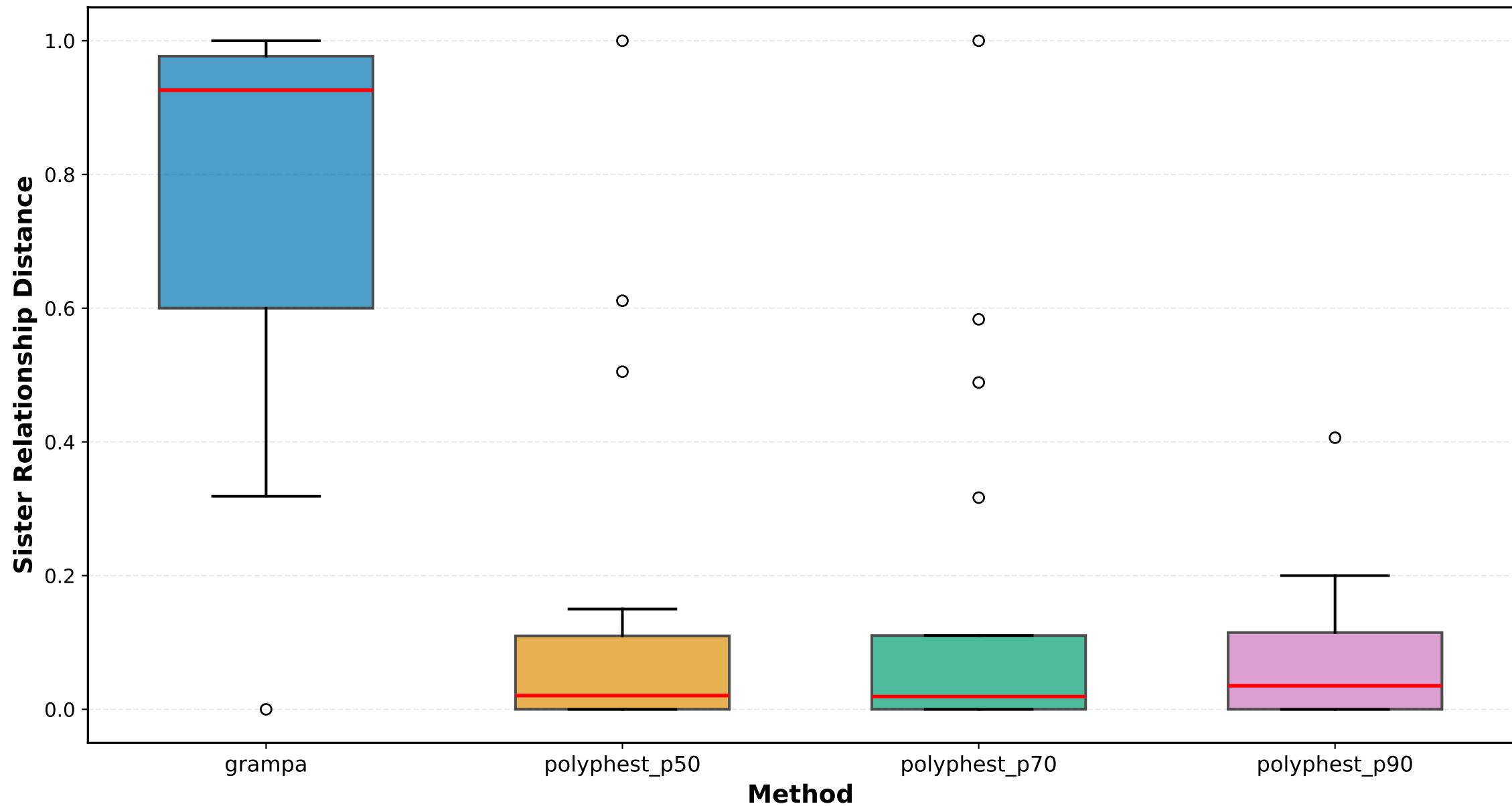
Sister Relationship Distance Distribution (ILS Low)
