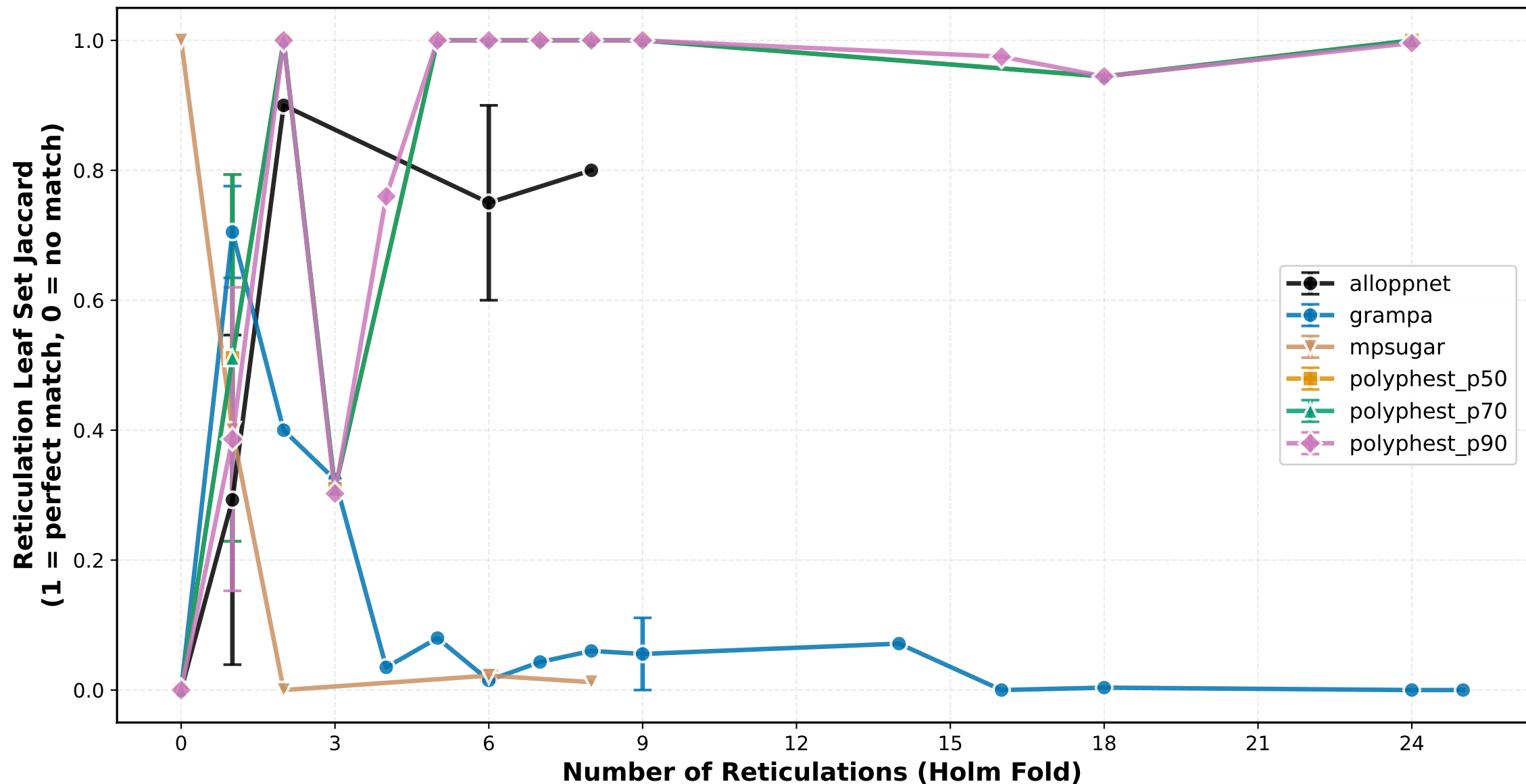
Reticulation Leaf Set Jaccard vs Number of Reticulations (Holm Fold) ILS High
