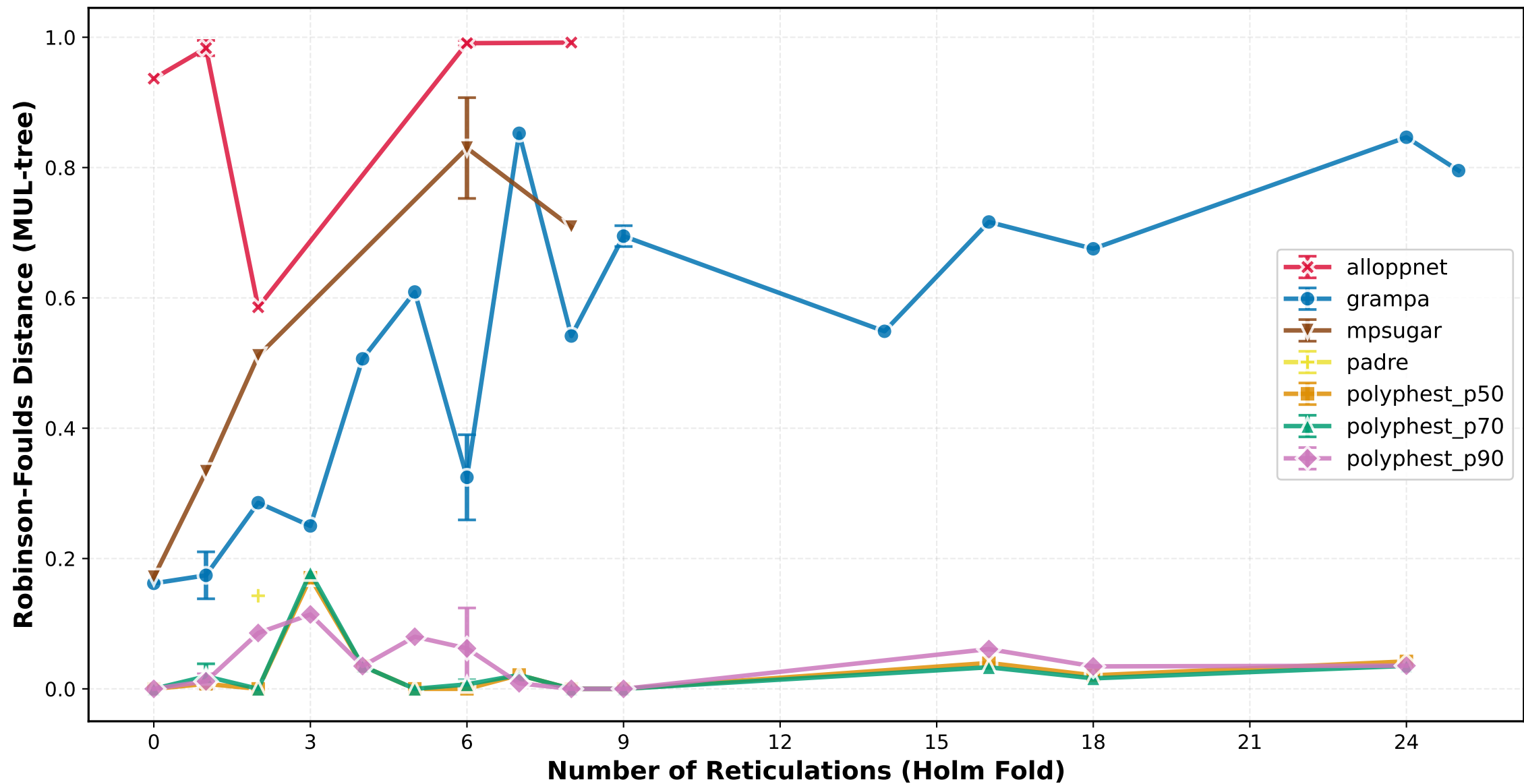
Robinson-Foulds Distance (MUL-tree) vs Number of Reticulations (Holm Fold) ILS Medium
