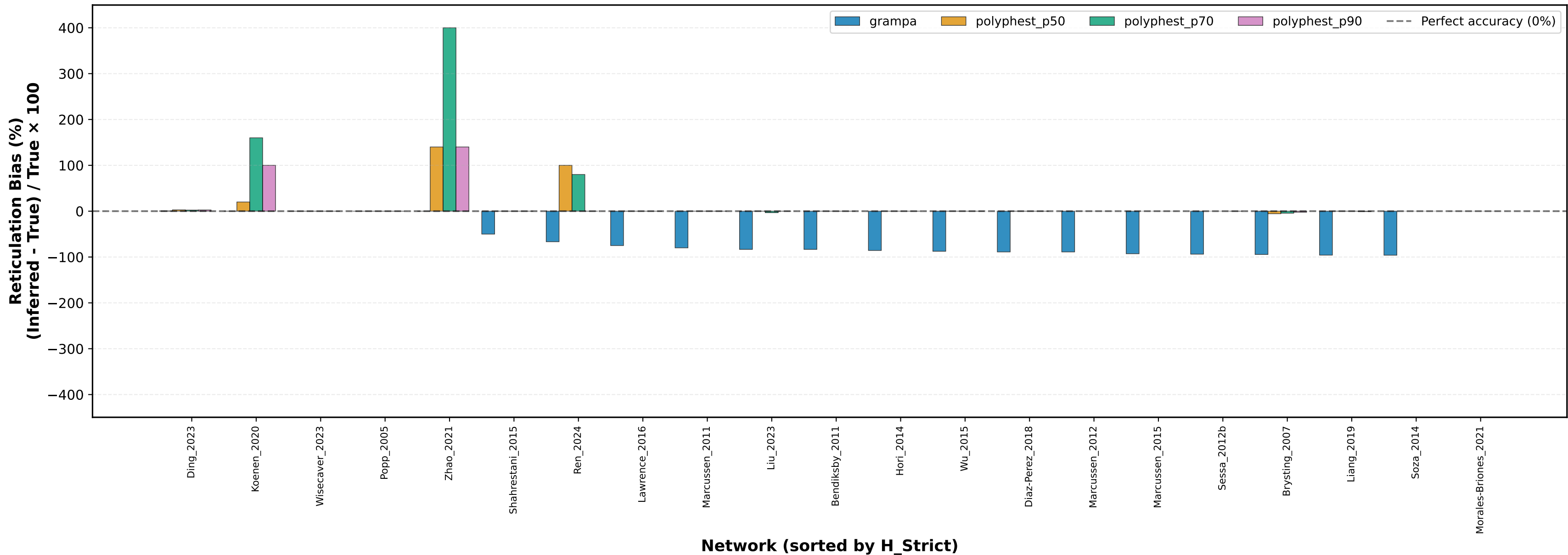
Per-Network Reticulation Bias (ILS Medium)
