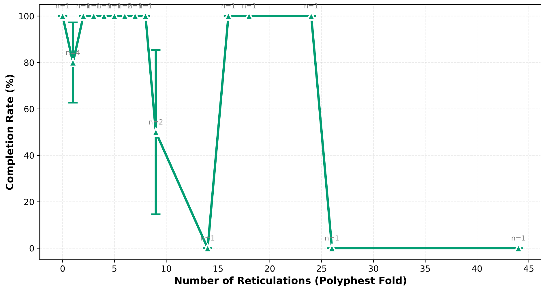
polyphest_p70 Completion Rate vs Number of Reticulations (Polyphest Fold) (ILS Low)
