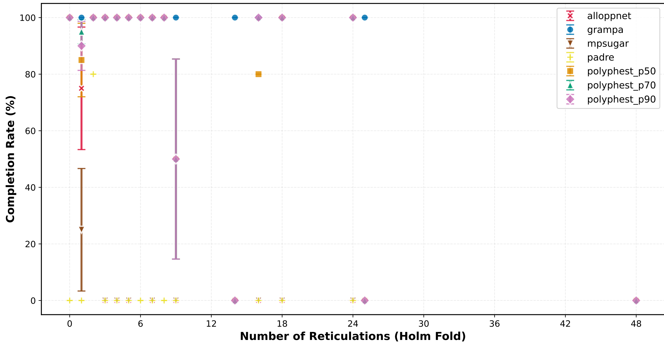
Completion Rate vs Number of Reticulations (Holm Fold) ILS Medium
