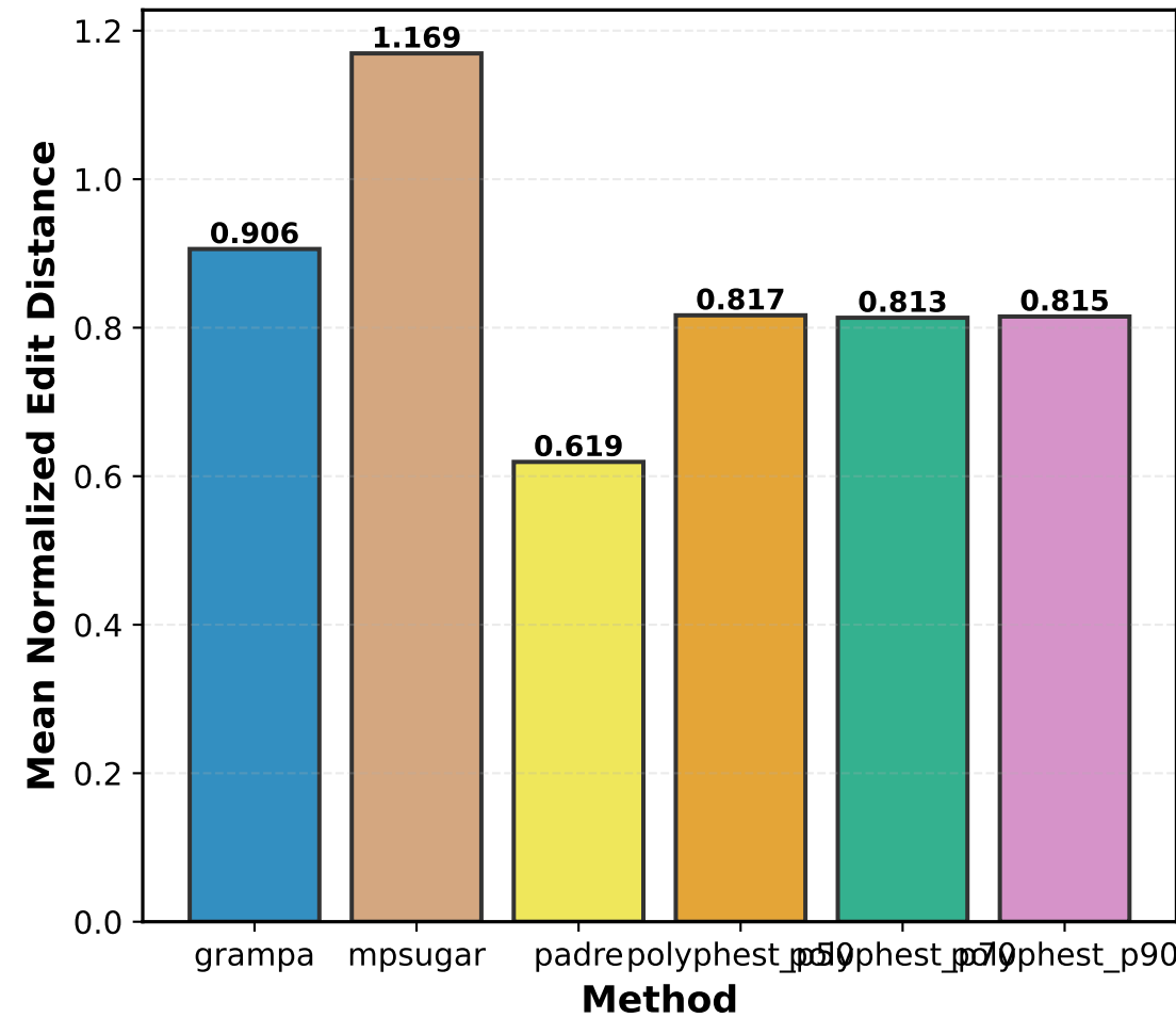
Network Accuracy (lower = better)
