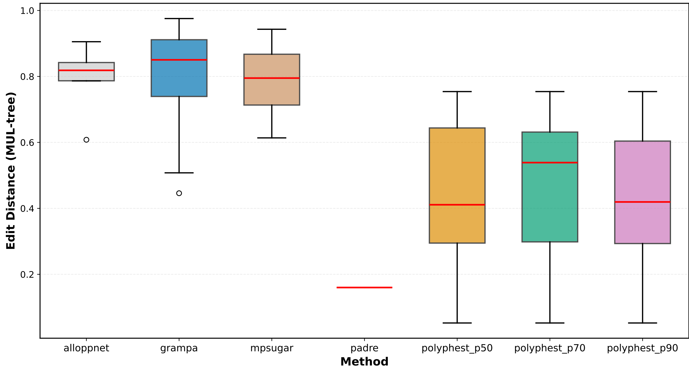
Edit Distance (MUL-tree) Distribution (ILS Medium)
