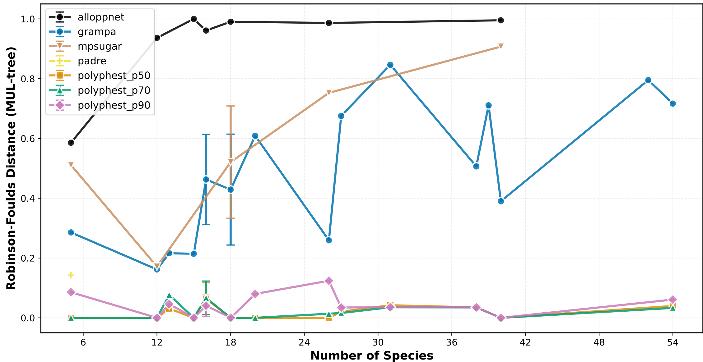
Robinson-Foulds Distance (MUL-tree) vs Number of Species ILS Medium
