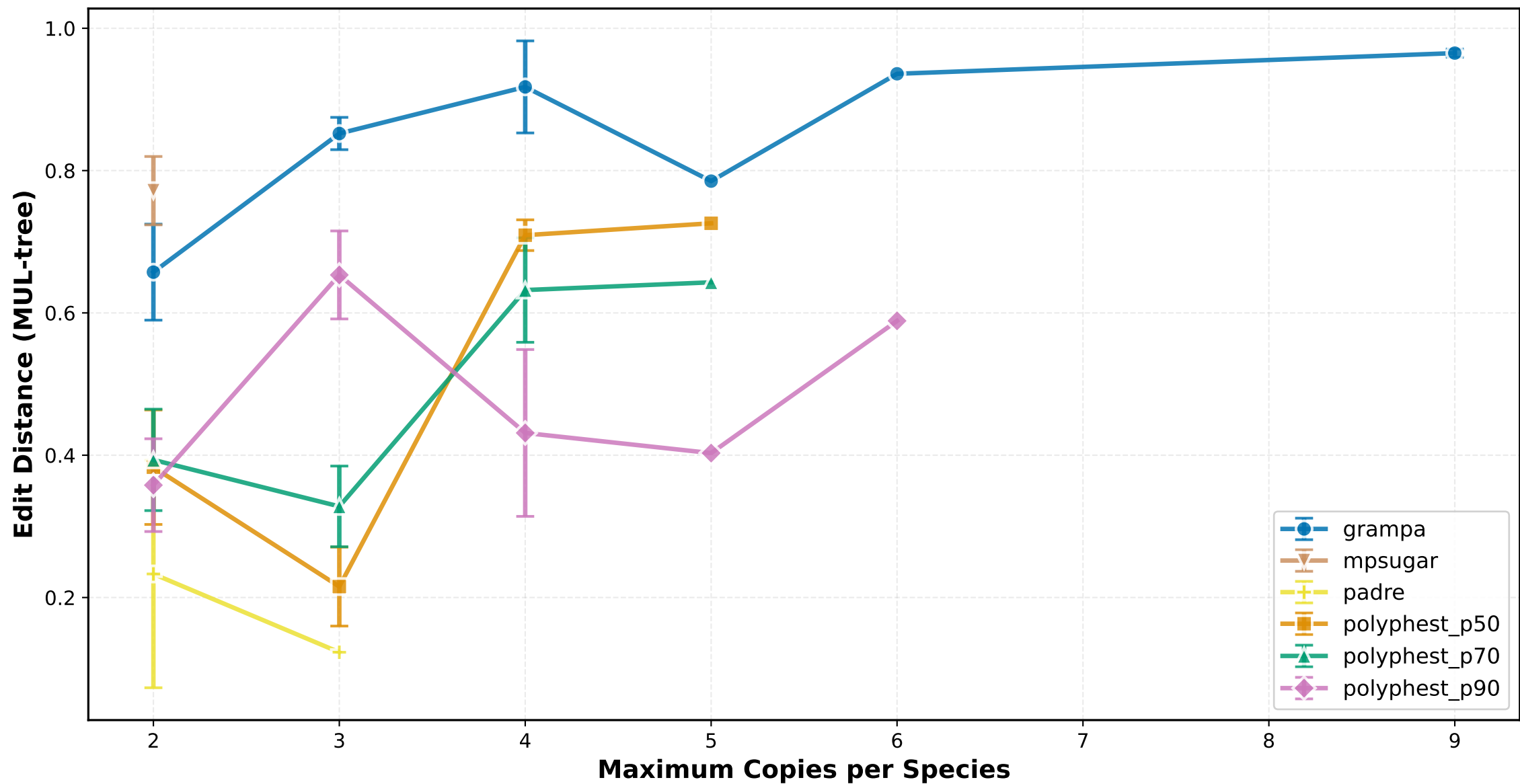
Edit Distance (MUL-tree) vs Maximum Copies per Species ILS Low
