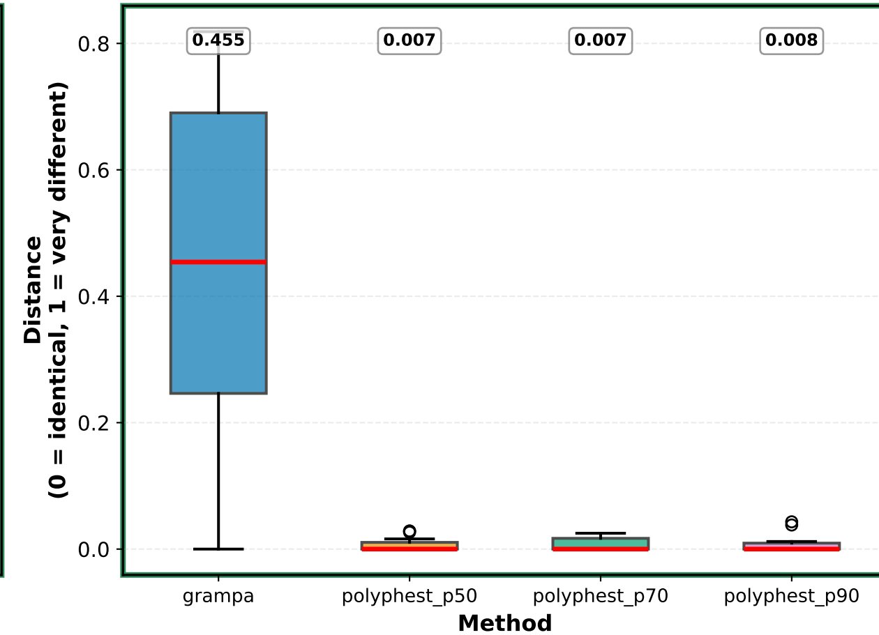
RF Distance (MUL-tree)
