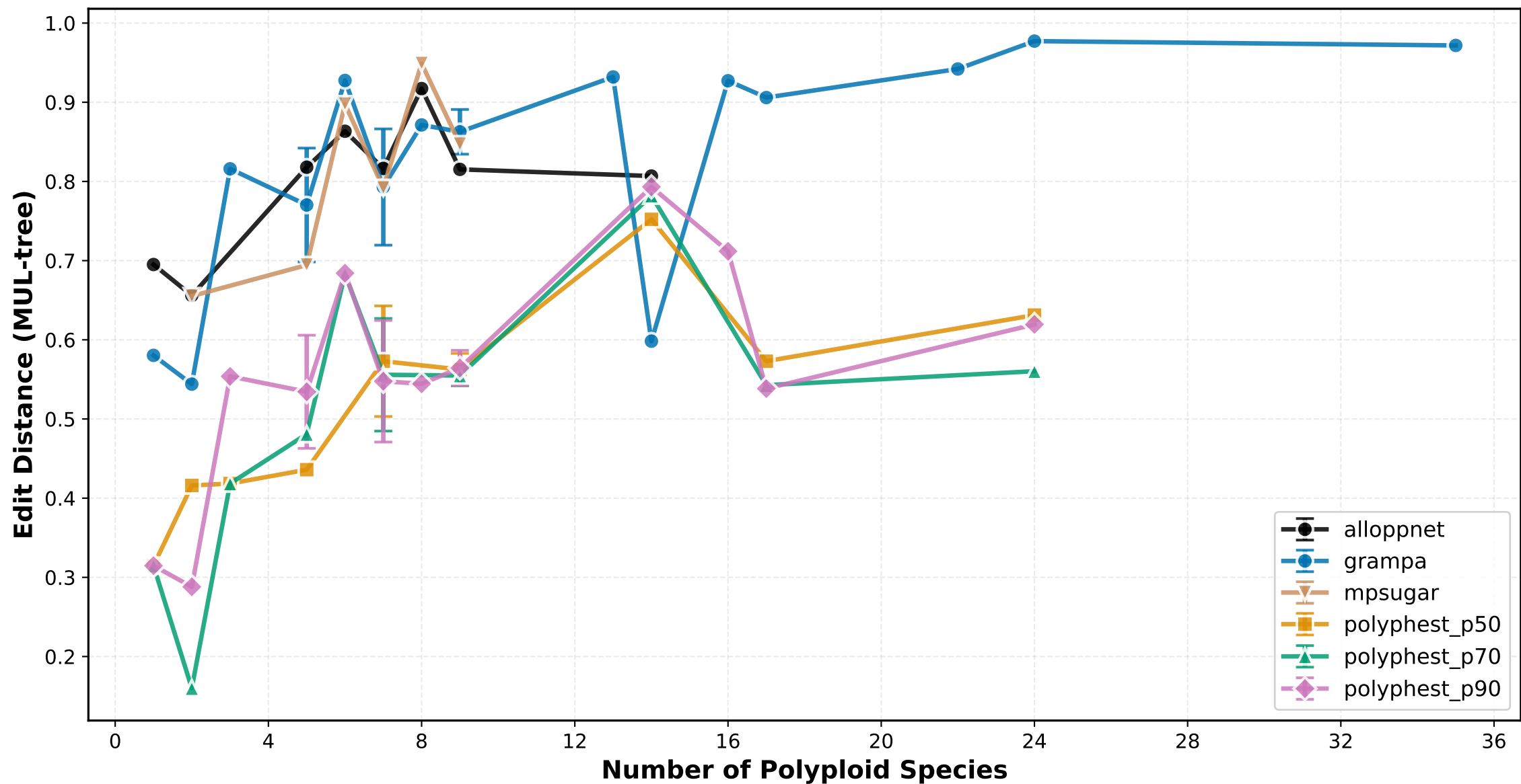
Edit Distance (MUL-tree) vs Number of Polyploid Species ILS High
