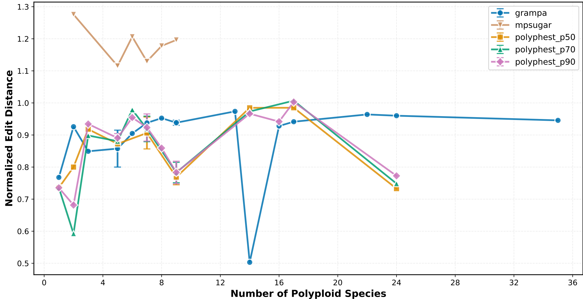
Normalized Edit Distance vs Number of Polyploid Species ILS High
