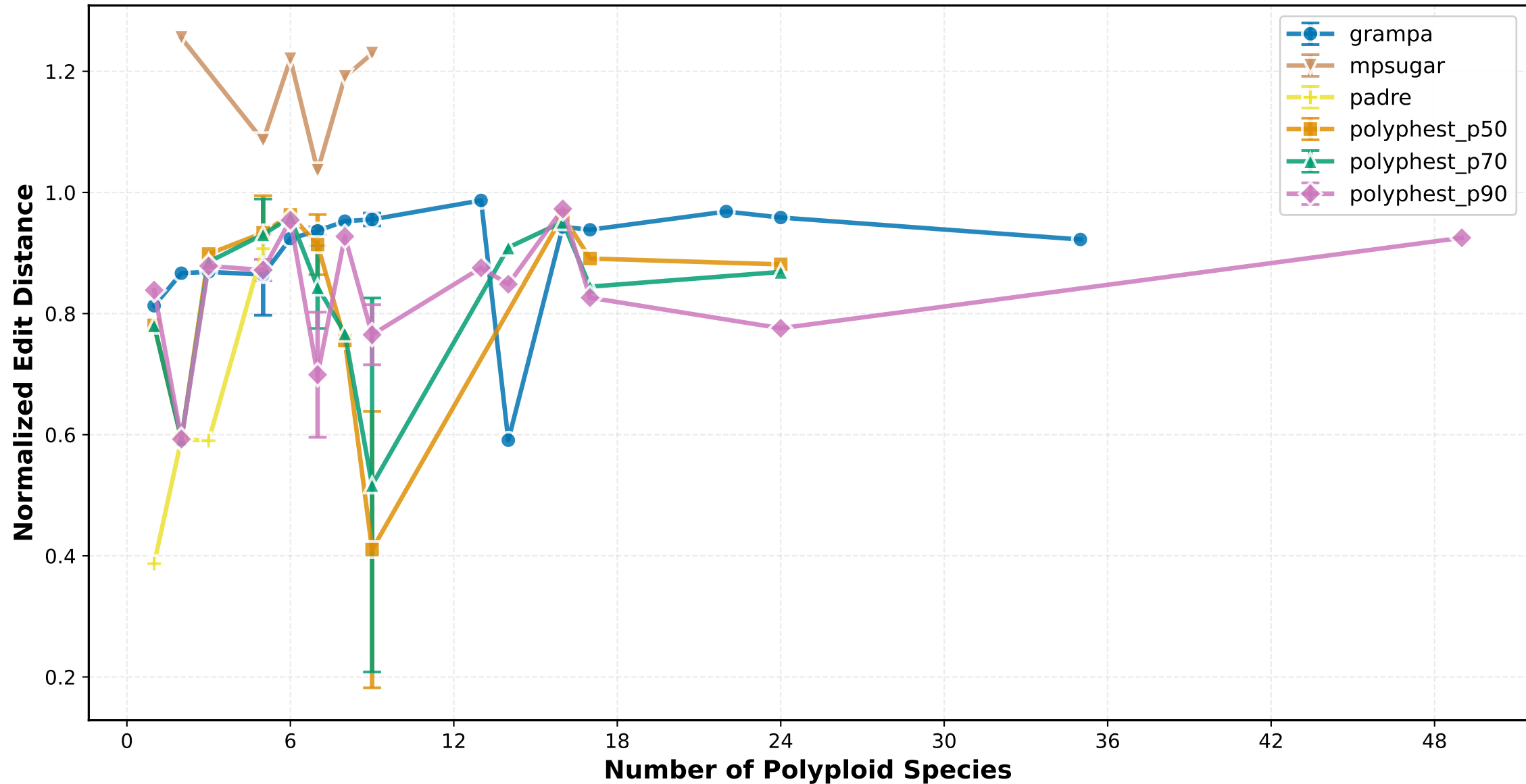
Normalized Edit Distance vs Number of Polyploid Species ILS Low
