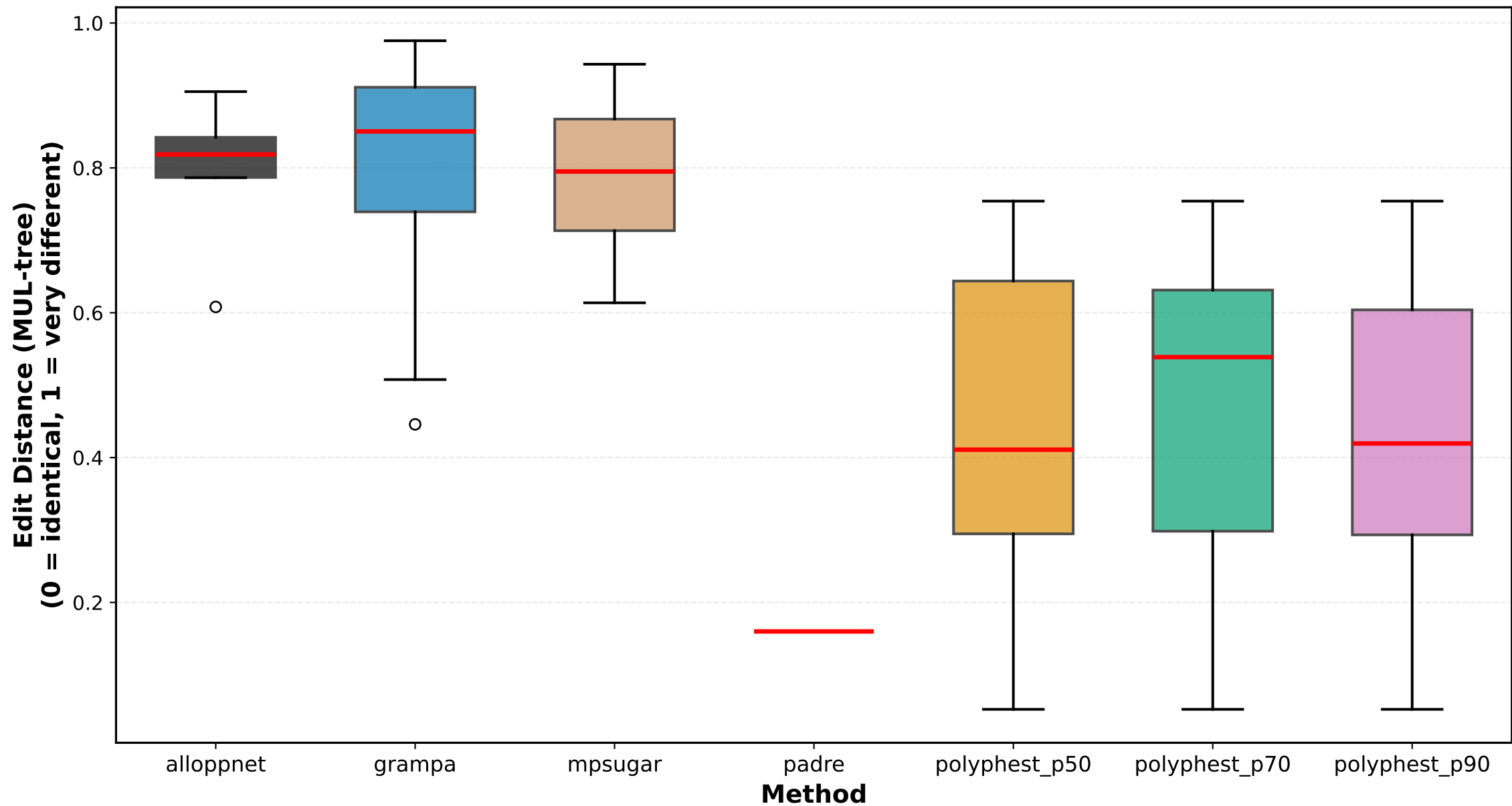
Edit Distance Distribution - MUL-tree (ILS Medium)
