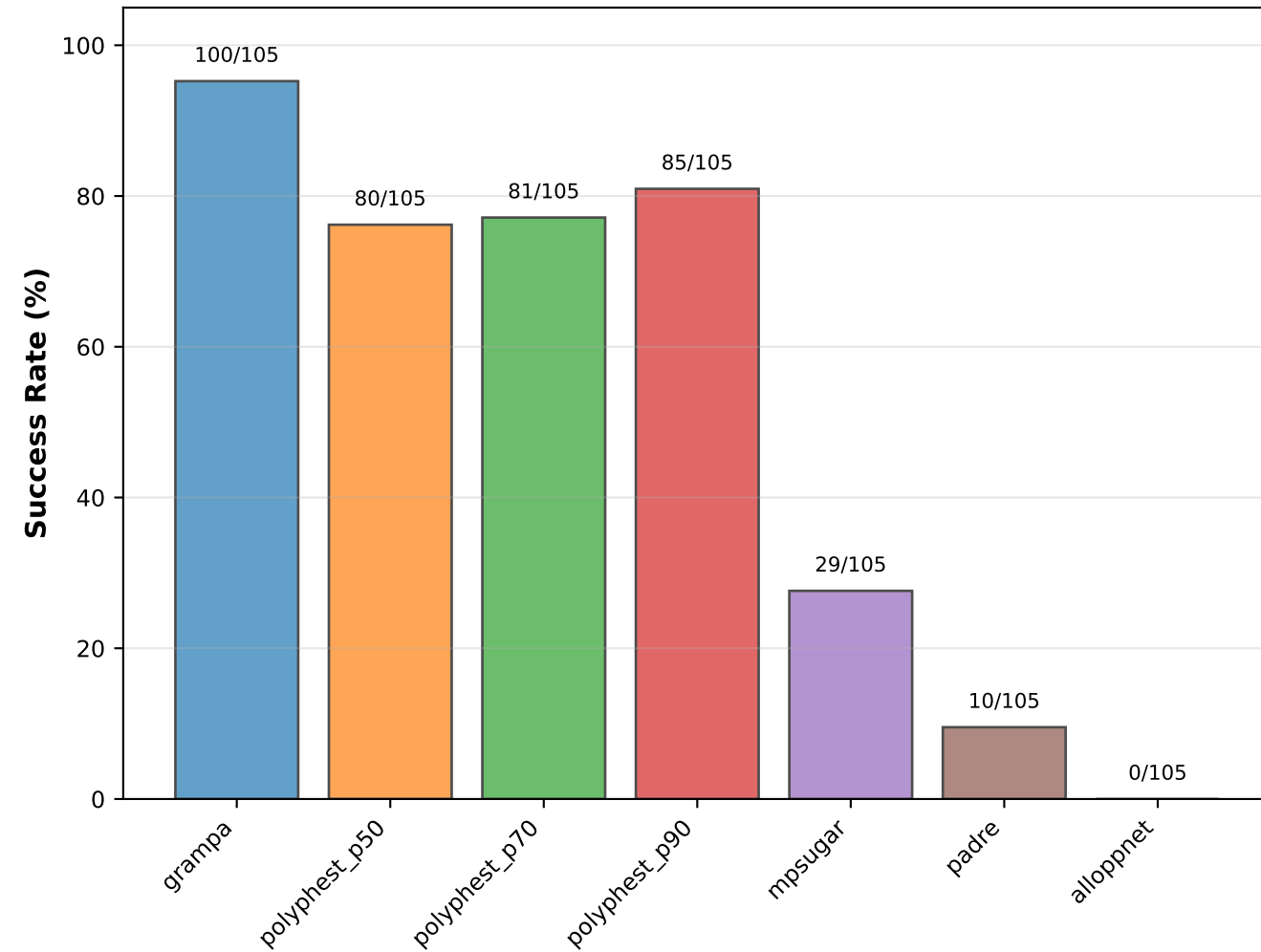
Success Rate
