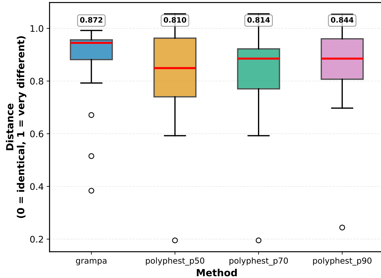
Network Edit Distance
