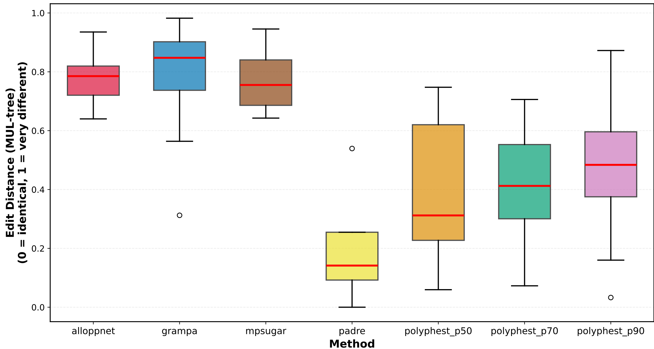
Edit Distance Distribution - MUL-tree (ILS Low)
