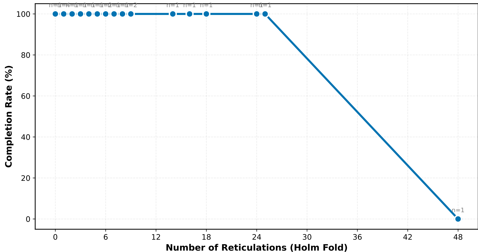
grampa Completion Rate vs Number of Reticulations (Holm Fold) (ILS Low)
