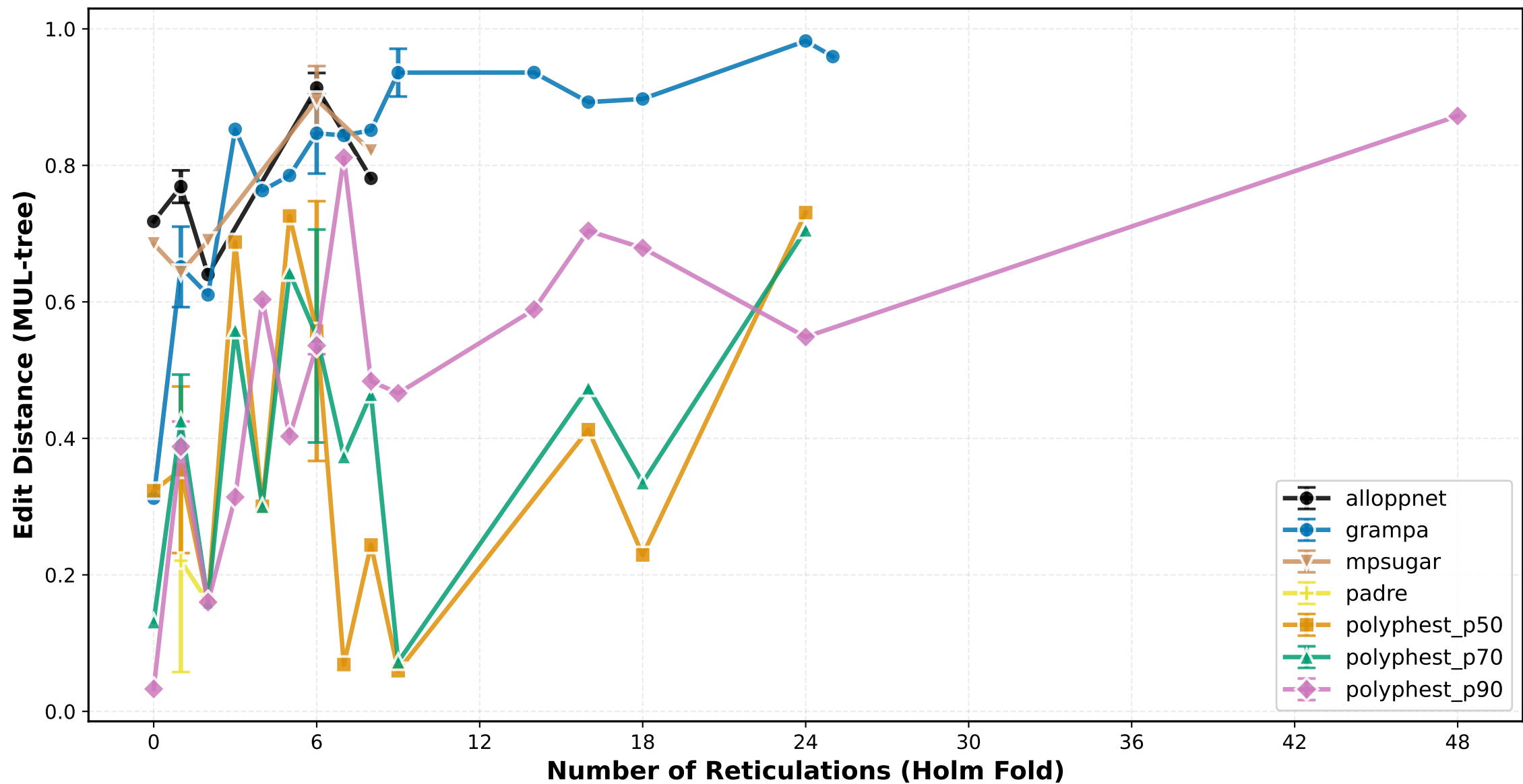
Edit Distance (MUL-tree) vs Number of Reticulations (Holm Fold) ILS Low
