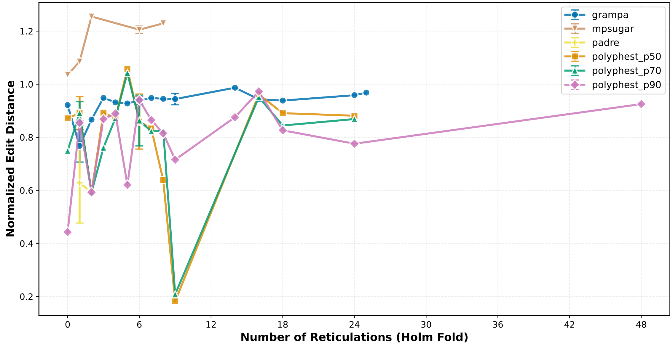
Normalized Edit Distance vs Number of Reticulations (Holm Fold) ILS Low
