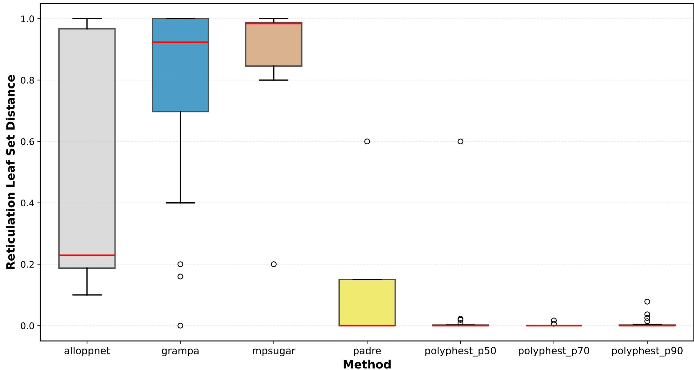
Reticulation Leaf Set Distance Distribution (ILS Low)
