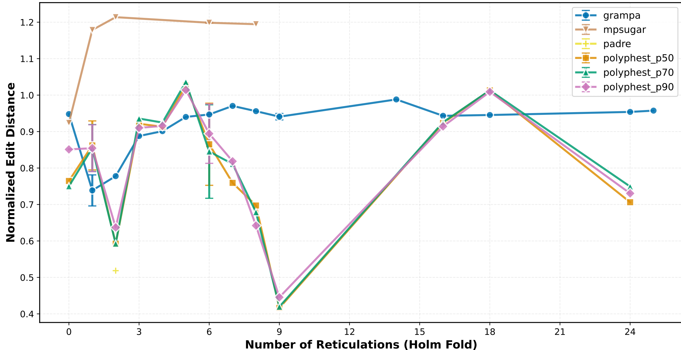
Normalized Edit Distance vs Number of Reticulations (Holm Fold) ILS Medium
