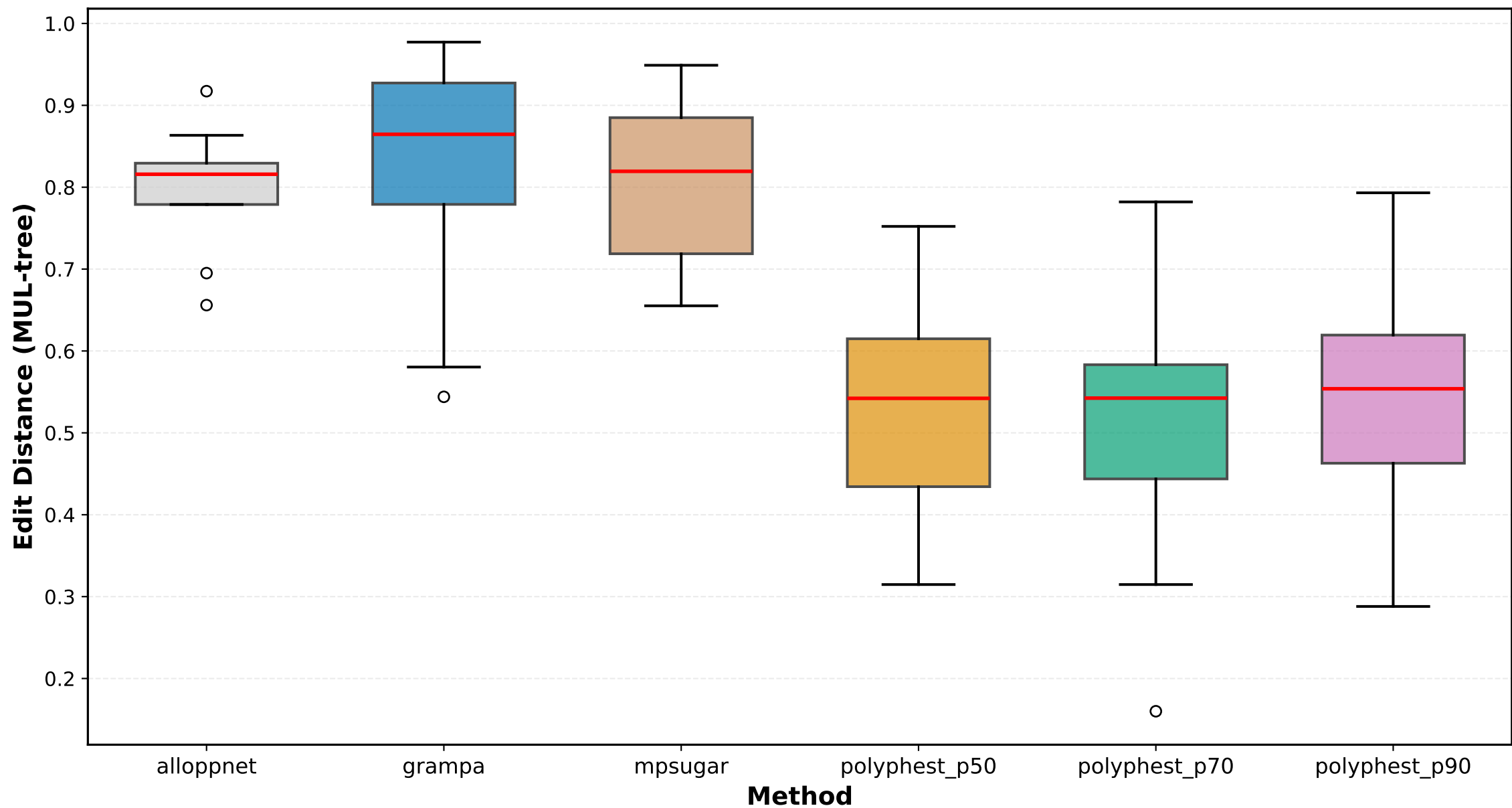
Edit Distance (MUL-tree) Distribution (ILS High)
