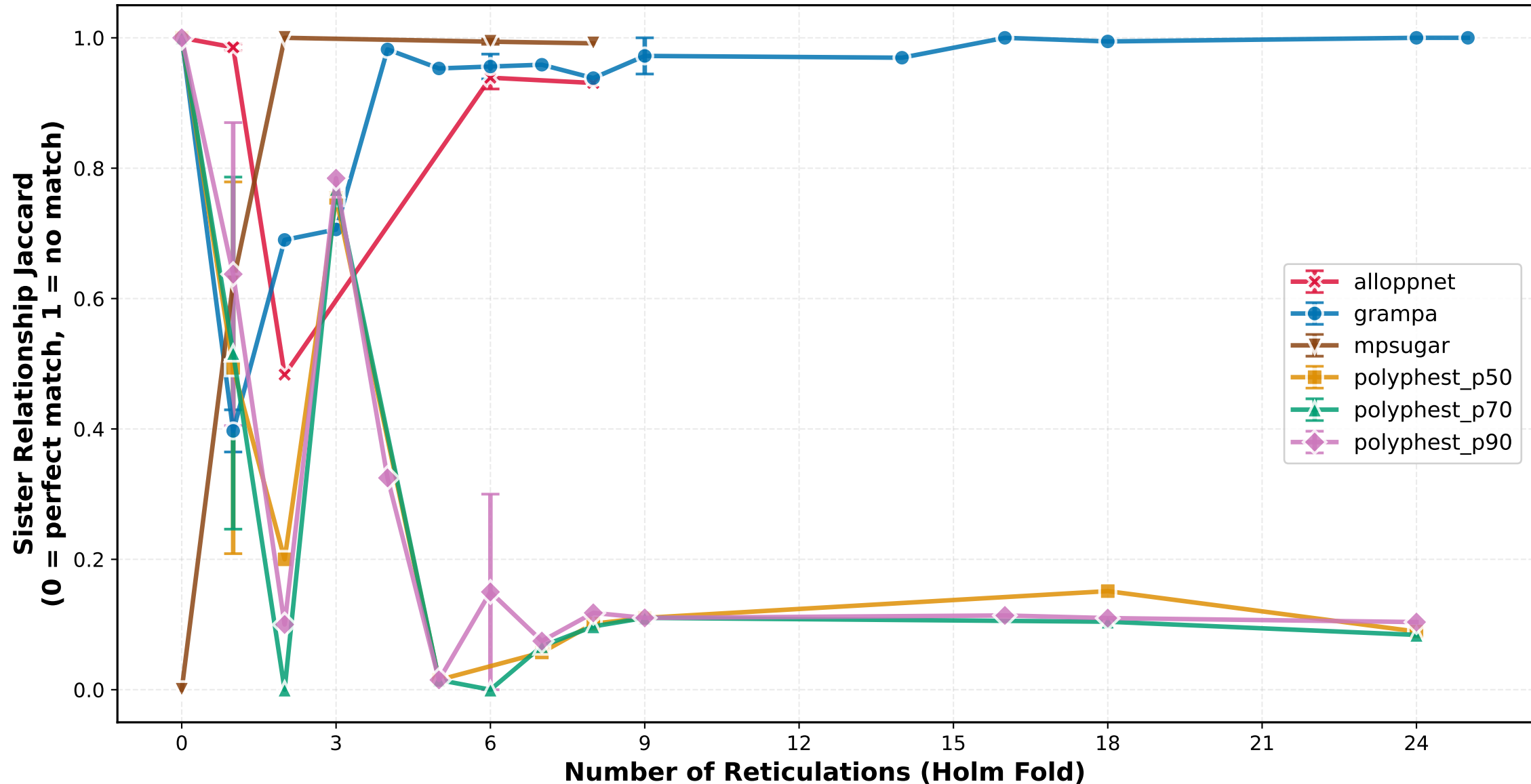
Sister Relationship Jaccard vs Number of Reticulations (Holm Fold) ILS High
