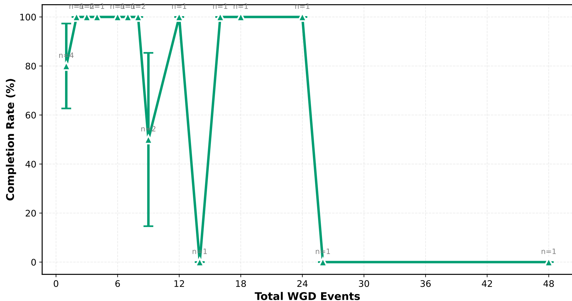
polypest_p70 Completion Rate vs Total WGD Events (ILS Low)
