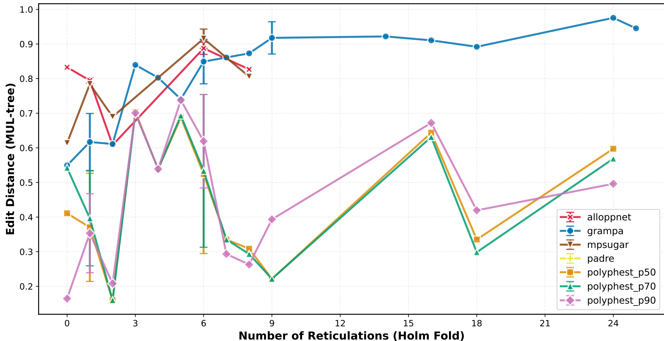
Edit Distance (MUL-tree) vs Number of Reticulations (Holm Fold) ILS Medium
