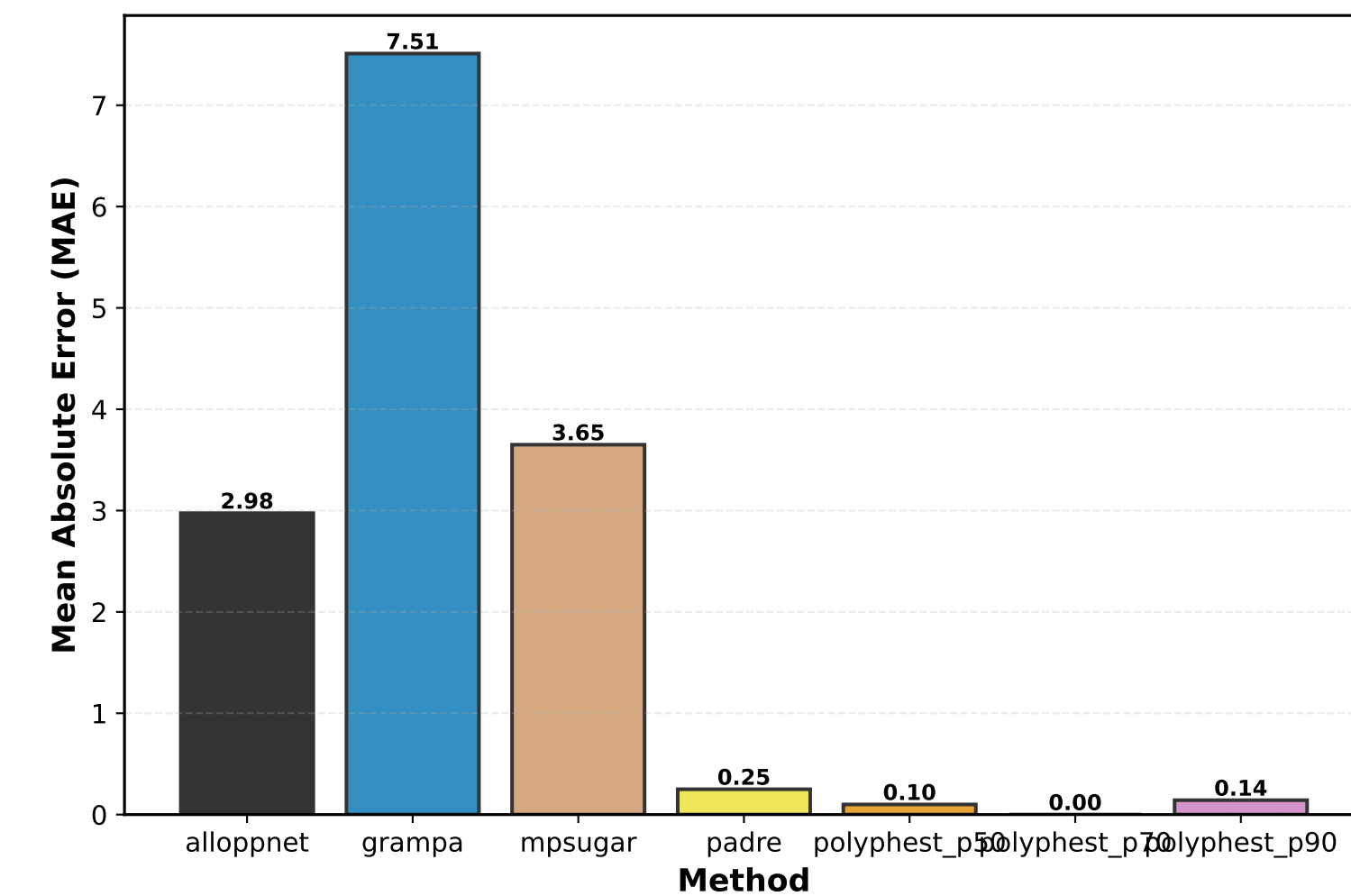
Reticulation Count: Absolute Error
