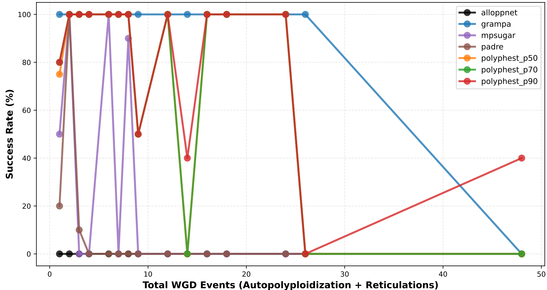
Success Rate vs Total WGD Events conf_ils_low_10M (ILS low)
