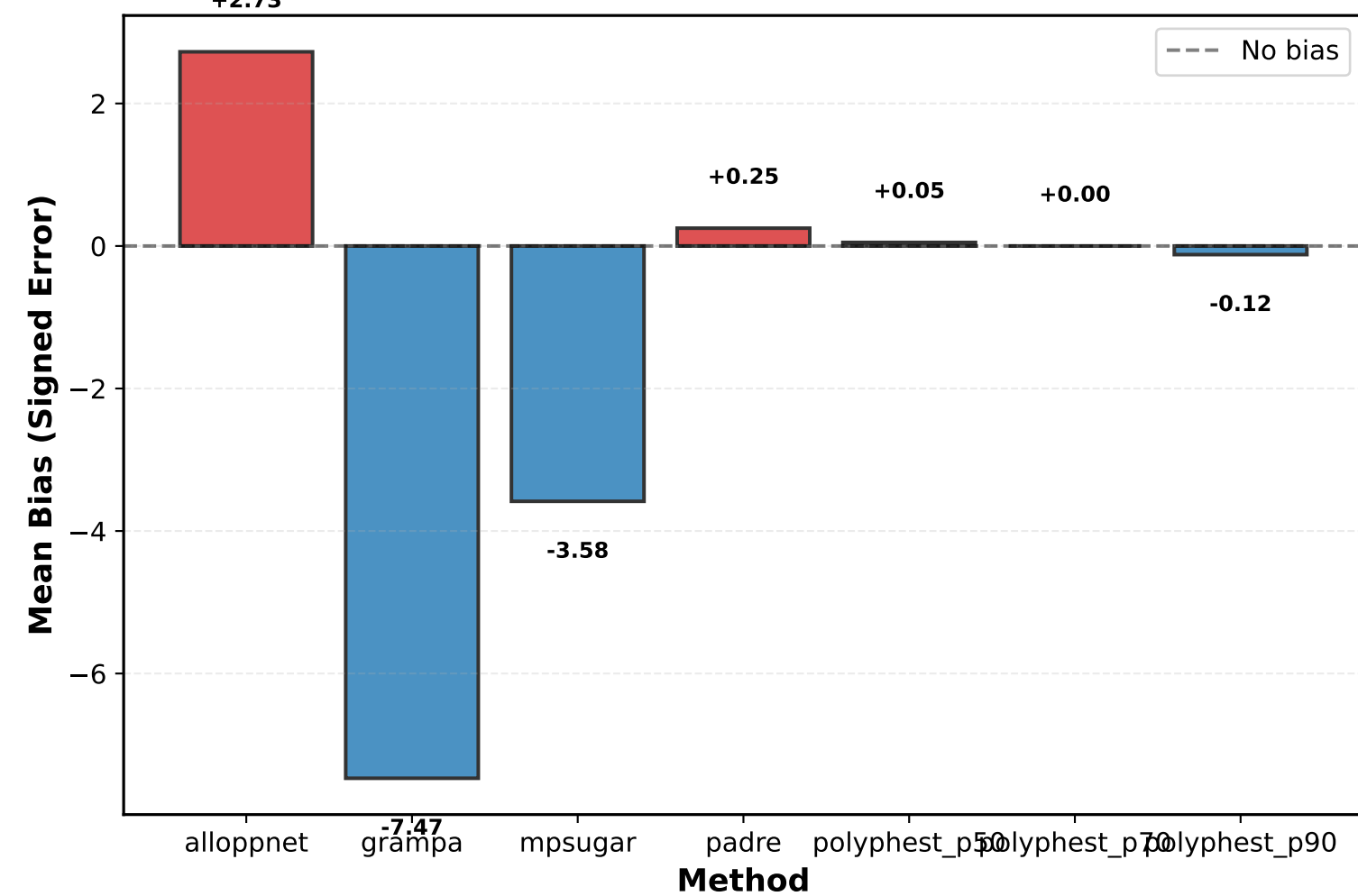
Reticulation Count: Bias [+ = Over-estimation, - = Under-estimation]
