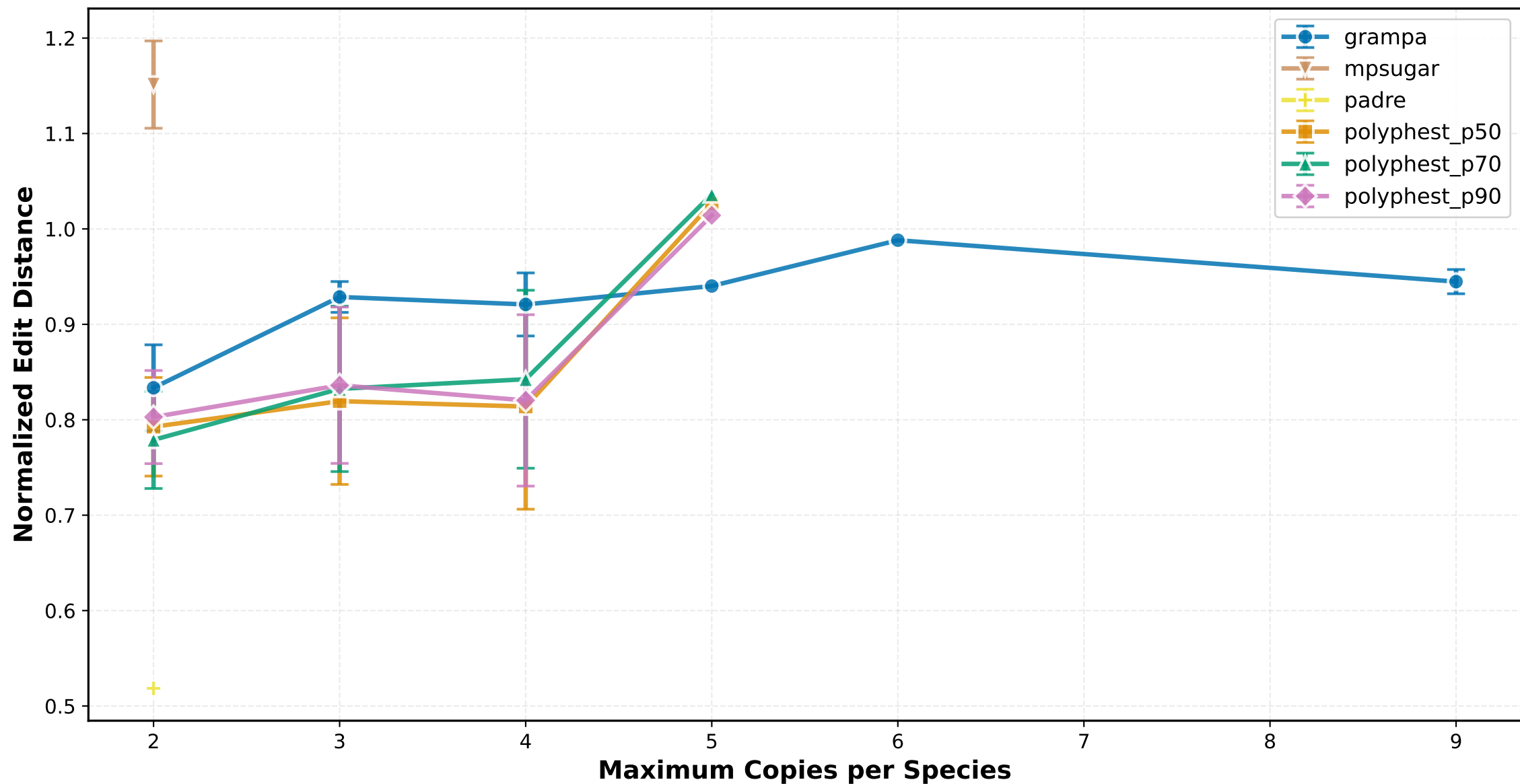
Normalized Edit Distance vs Maximum Copies per Species ILS Medium
