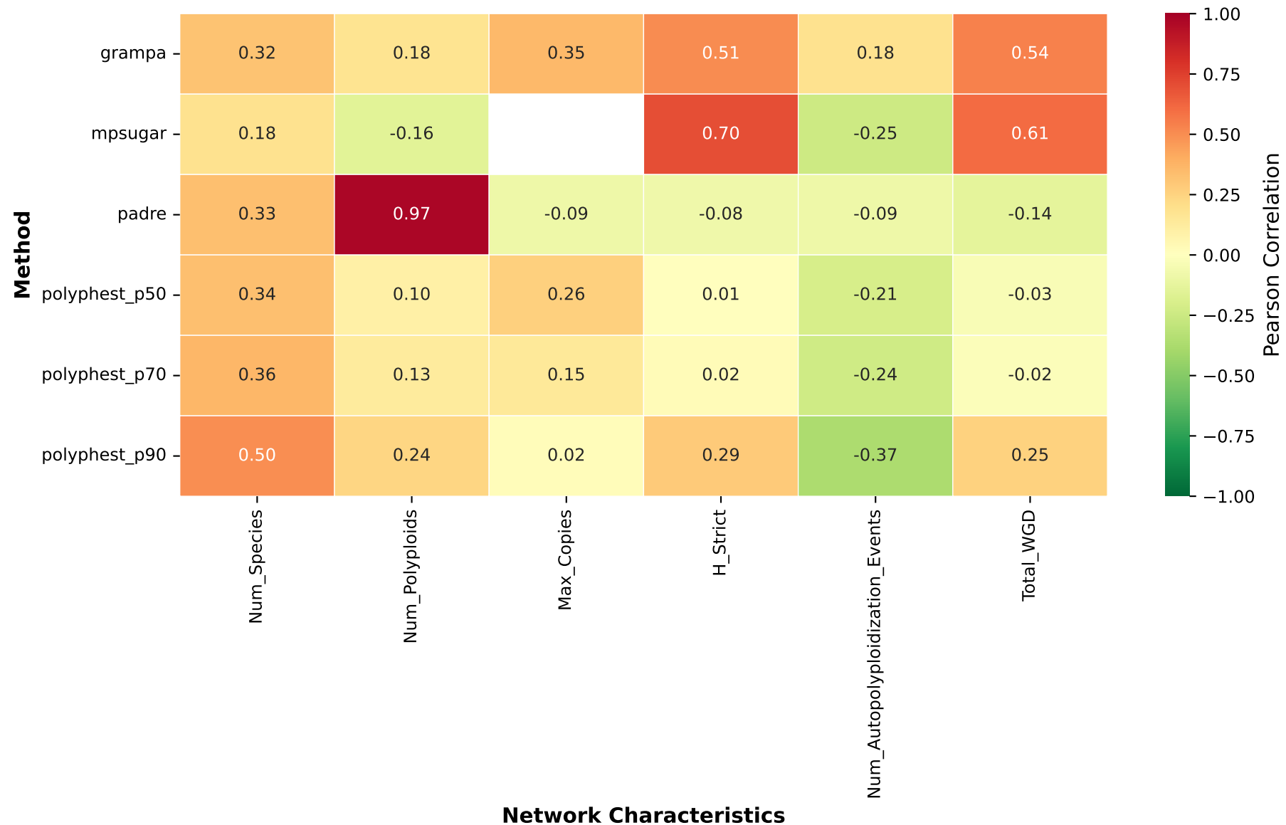
Network Characteristics vs Edit Distance conf_ils_low_10M (ILS low) (Red = harder with more, Green = easier with more)
