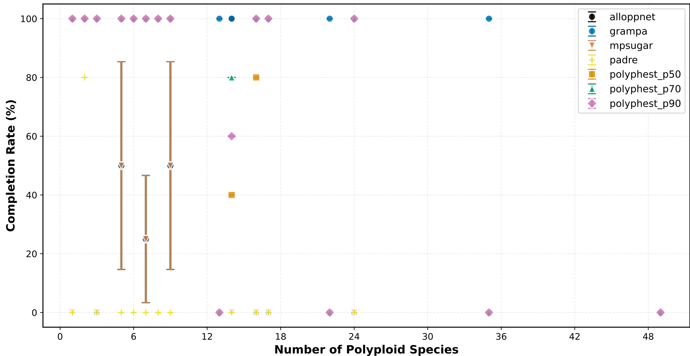
Completion Rate vs Number of Polyploid Species ILS Medium
