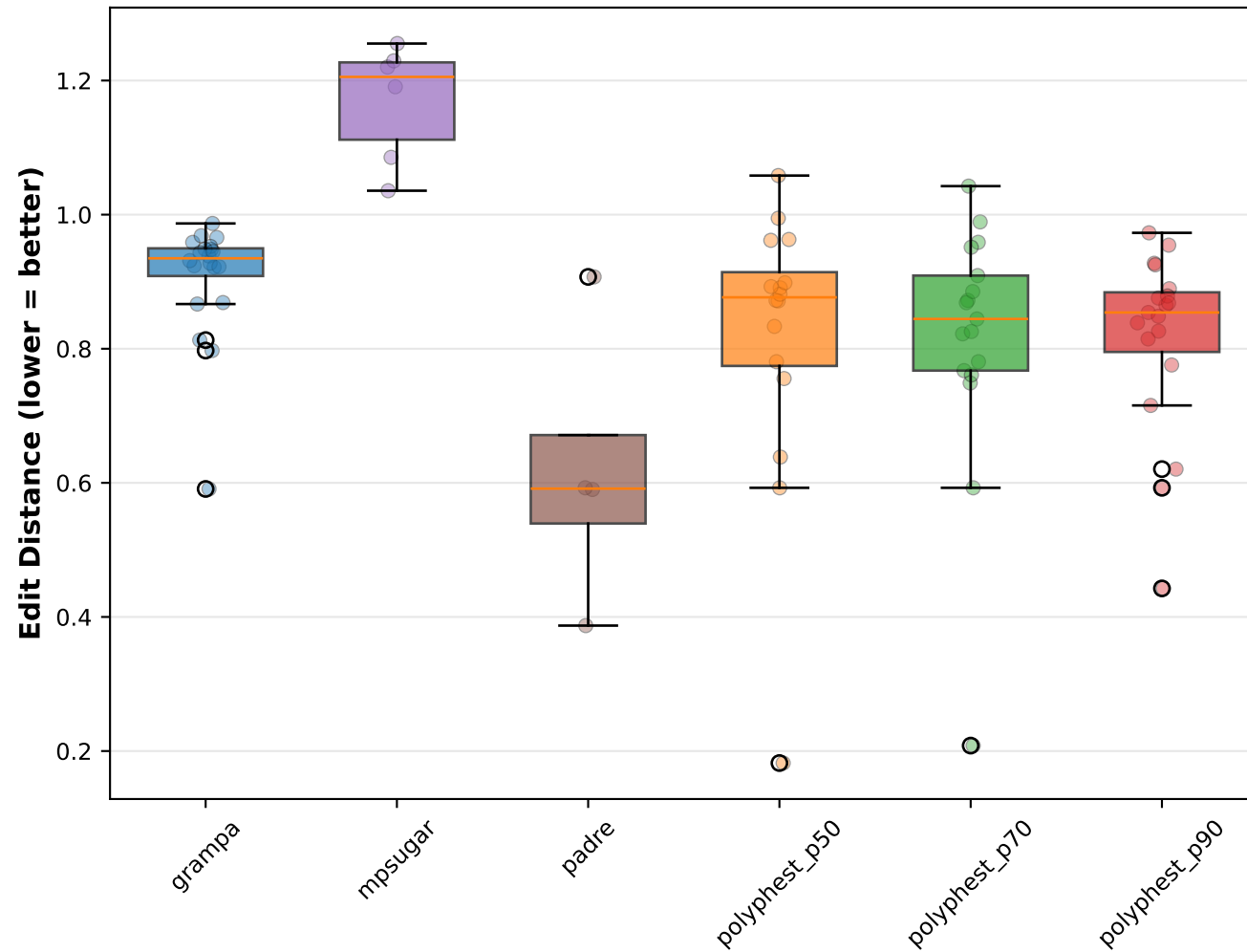
Edit Distance Distribution
