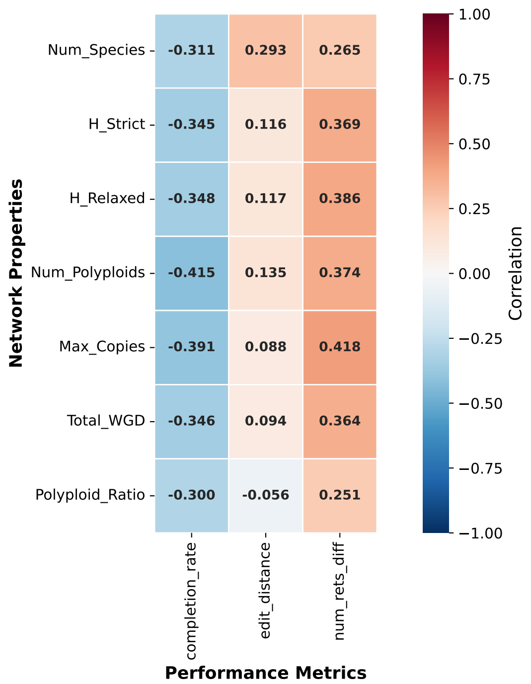
Network Properties vs Performance Metrics Correlation (Aggregated Across All Methods) ILS Low
