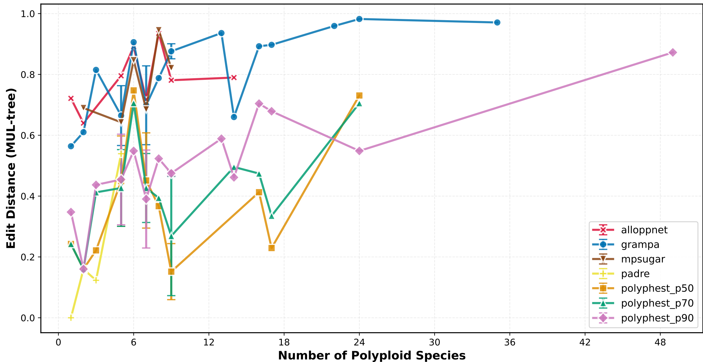
Edit Distance (MUL-tree) vs Number of Polyploid Species ILS Low
