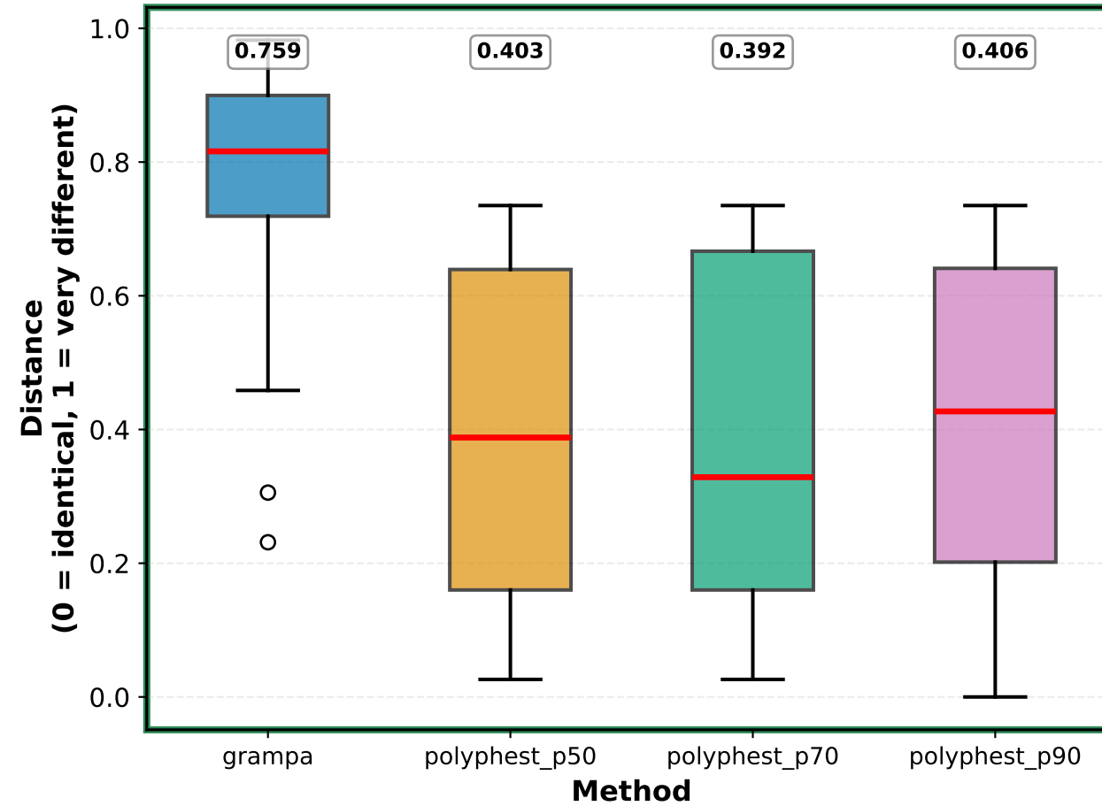
MUL-tree Edit Distance
