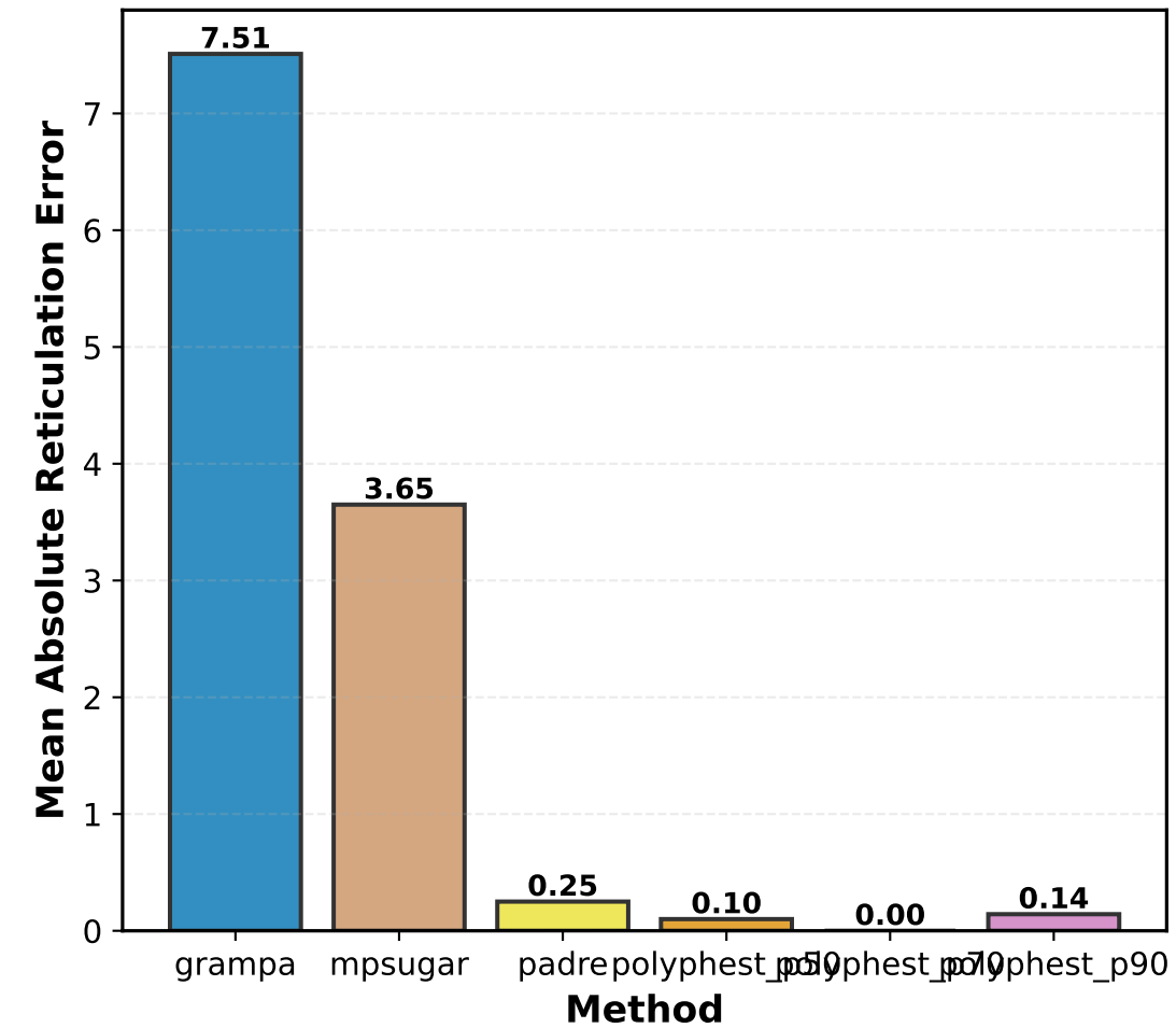
Reticulation Accuracy (lower = better)
