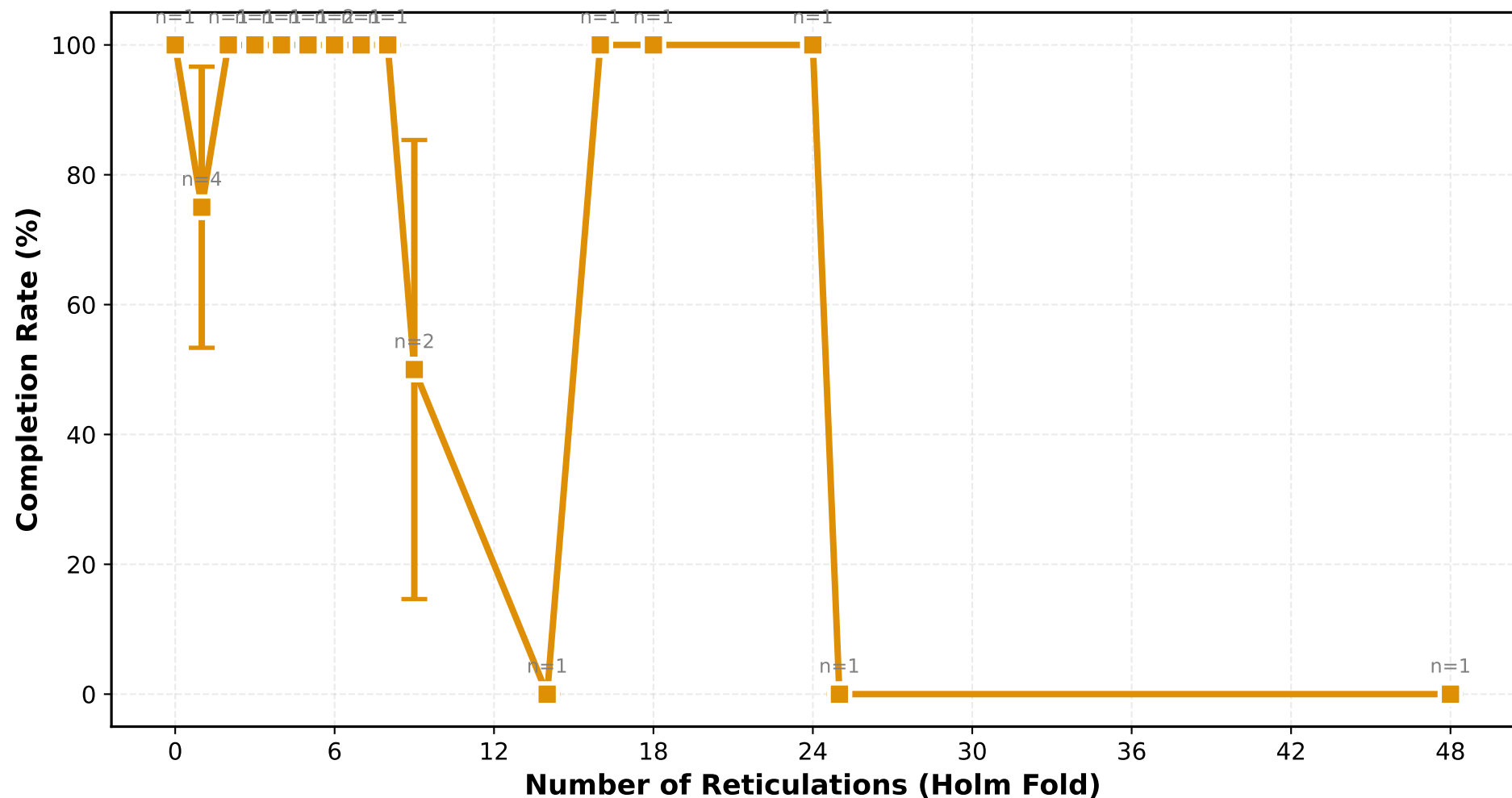
polypest_p50 Completion Rate vs Number of Reticulations (Holm Fold) (ILS Low)
