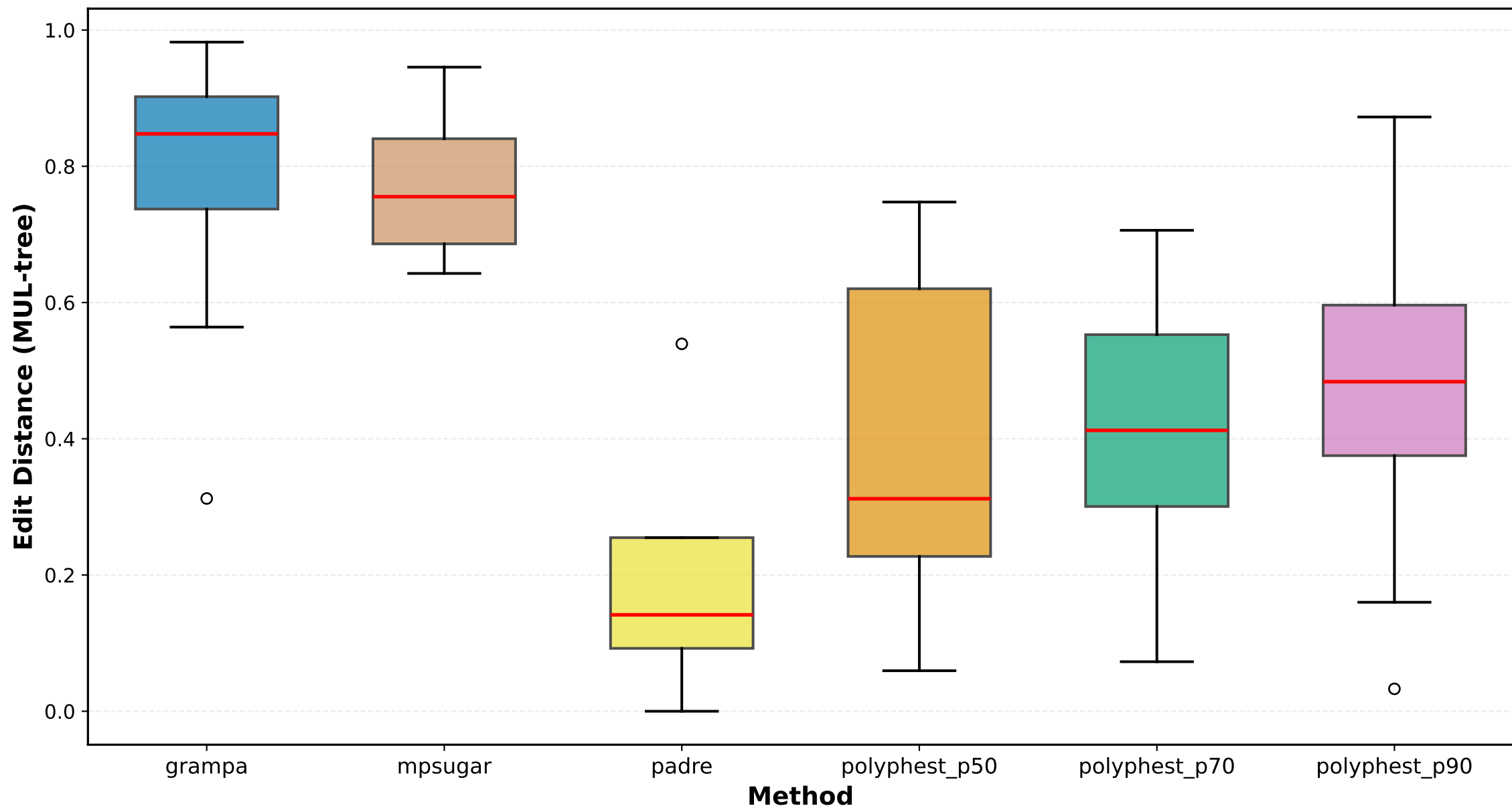
Edit Distance (MUL-tree) Distribution (ILS Low)
