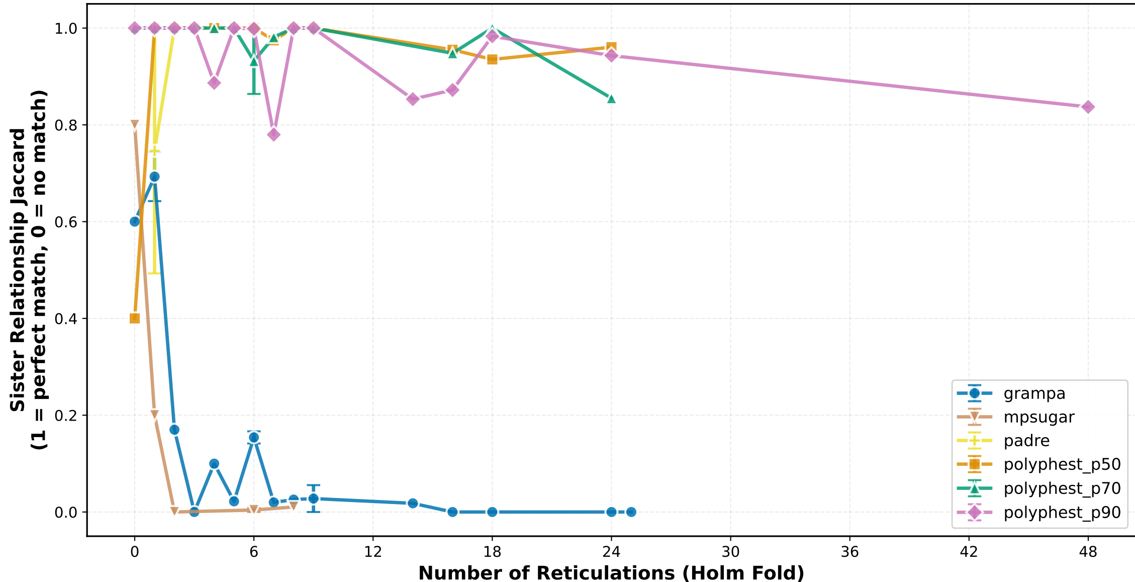
Sister Relationship Jaccard vs Number of Reticulations (Holm Fold) ILS Low
