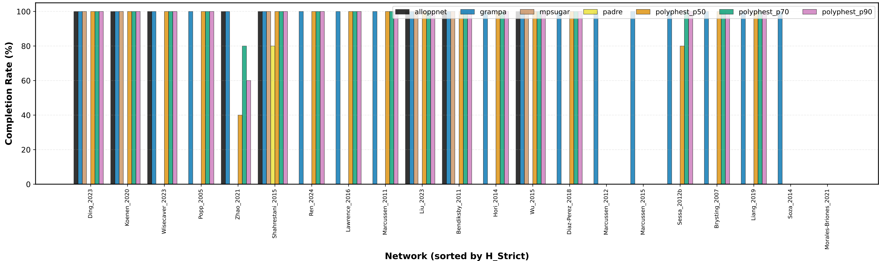
Per-Network Completion Rates (ILS Medium)
