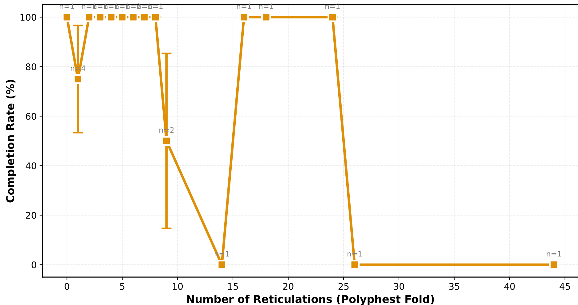
polyphest_p50 Completion Rate vs Number of Reticulations (Polyphest Fold) (ILS Low)
