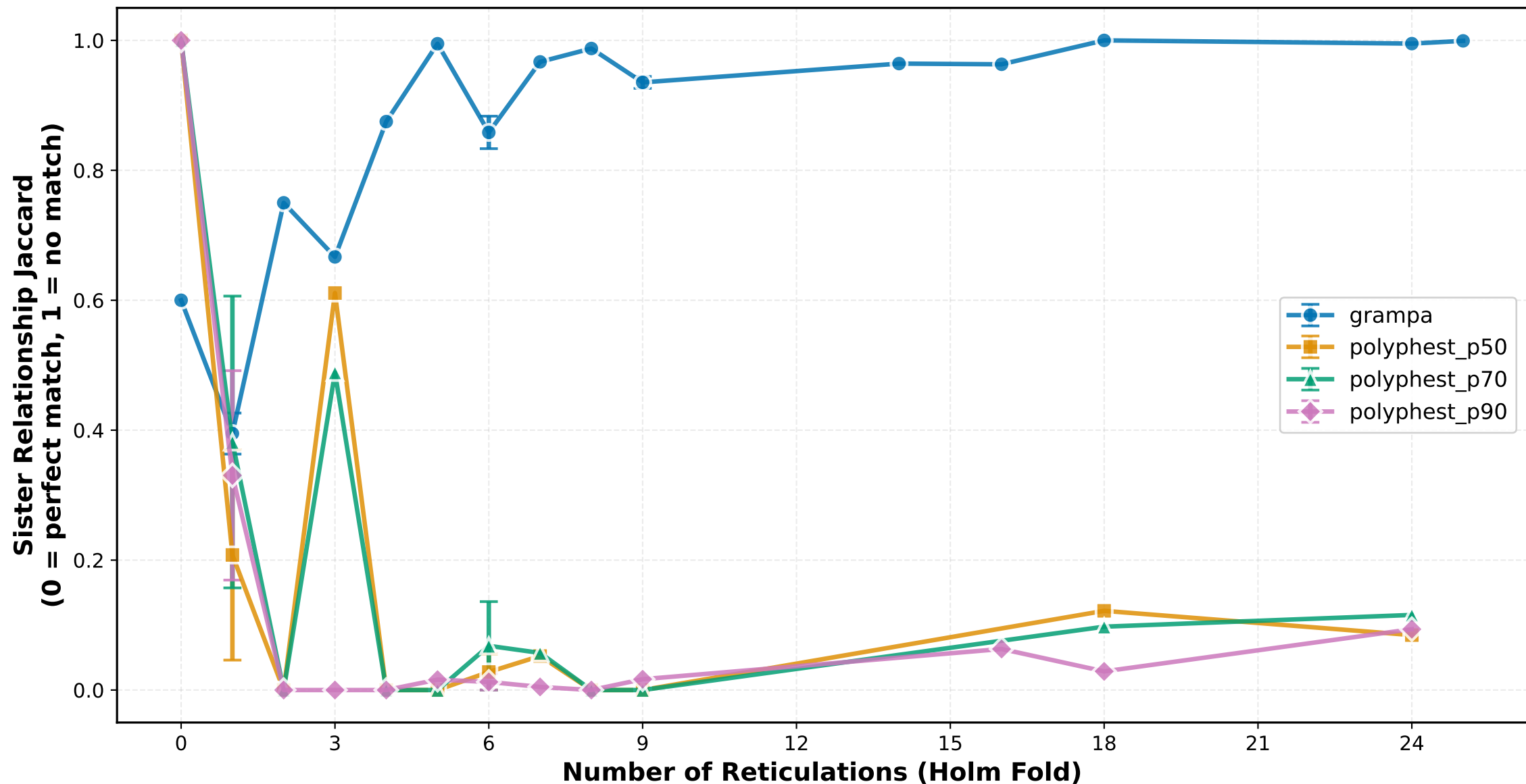
Sister Relationship Jaccard vs Number of Reticulations (Holm Fold) ILS Medium
