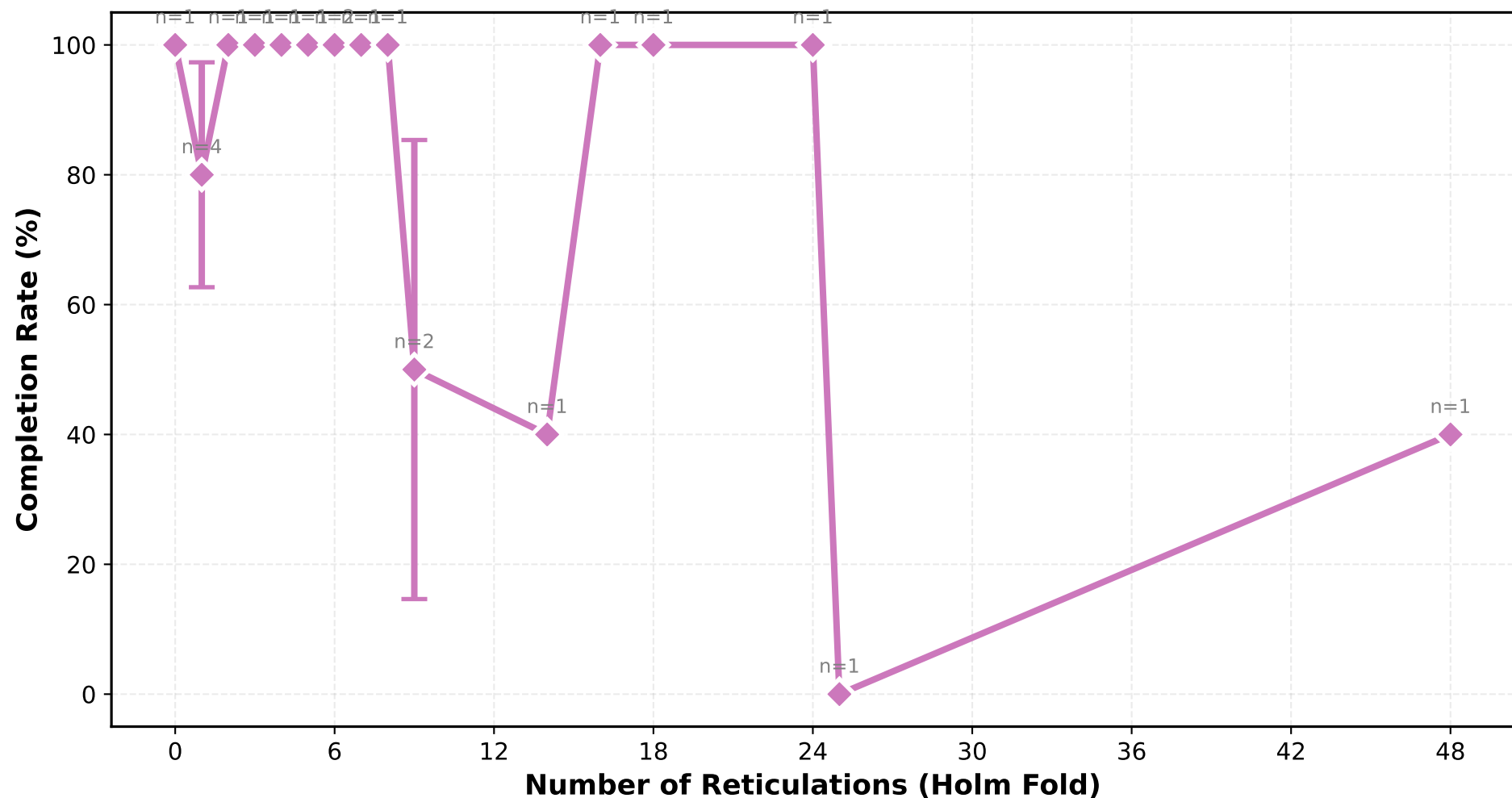
polyphest_p90 Completion Rate vs Number of Reticulations (Holm Fold) (ILS Low)
