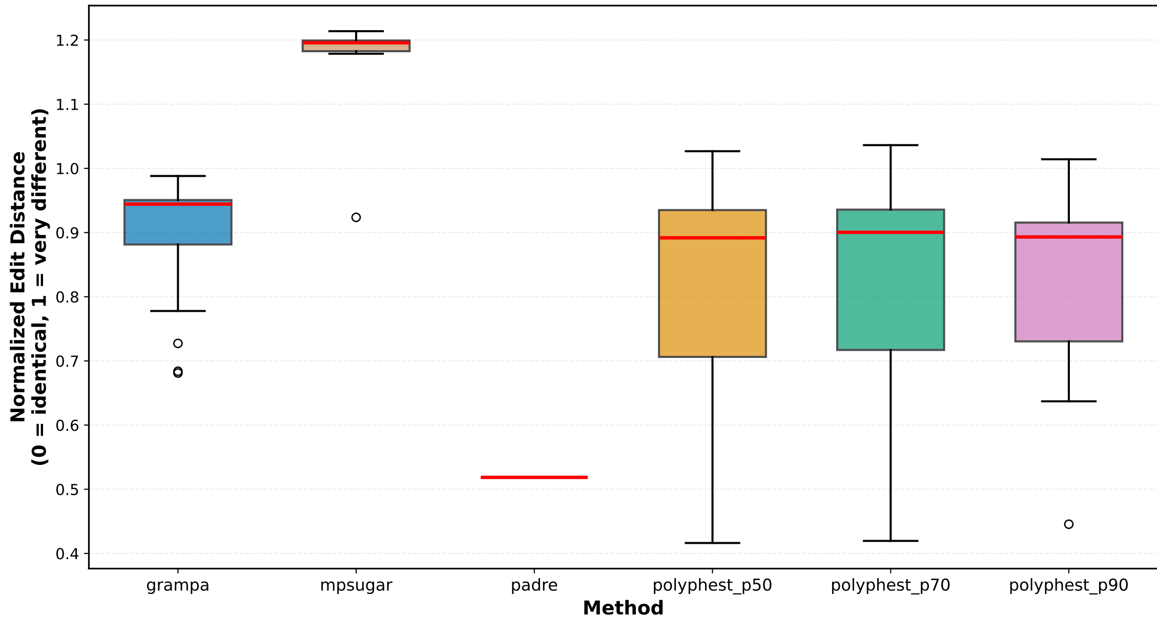
Edit Distance Distribution (ILS Medium)
