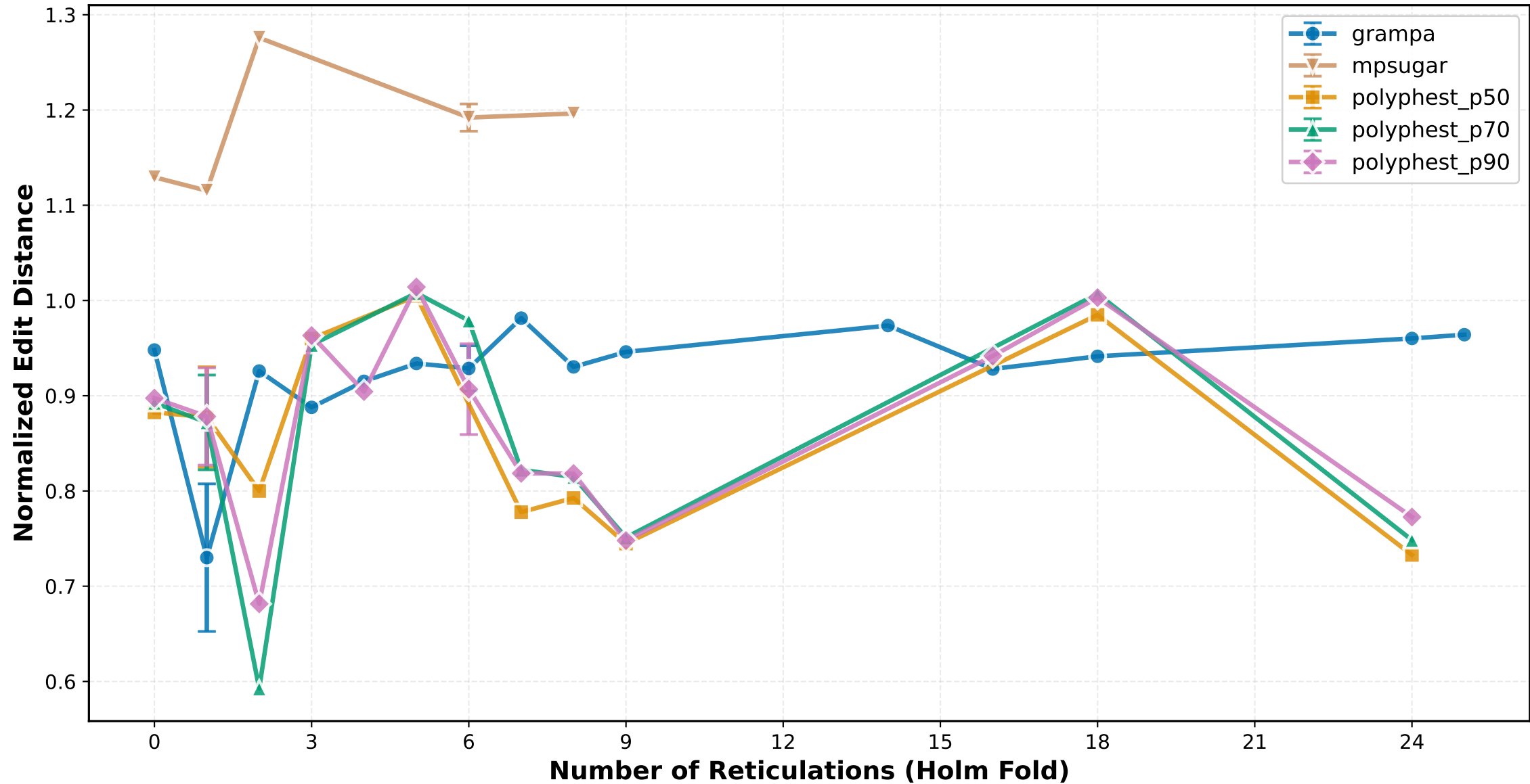
Normalized Edit Distance vs Number of Reticulations (Holm Fold) ILS High
