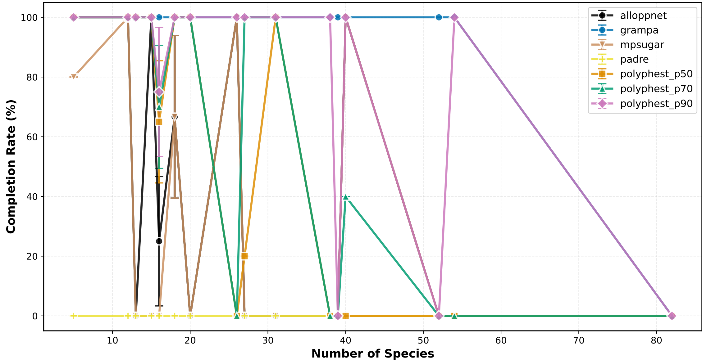
Completion Rate vs Number of Species ILS High
