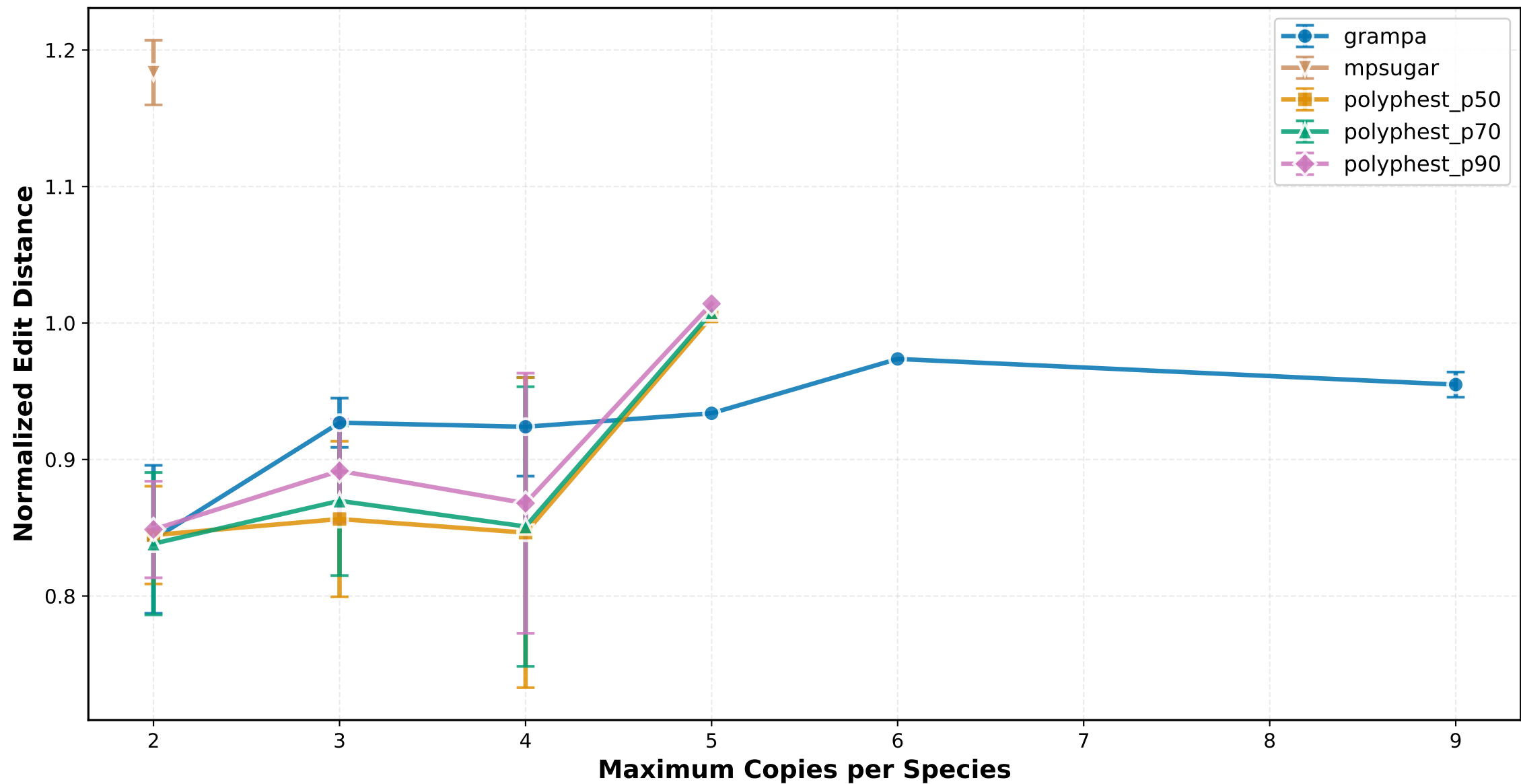
Normalized Edit Distance vs Maximum Copies per Species ILS High
