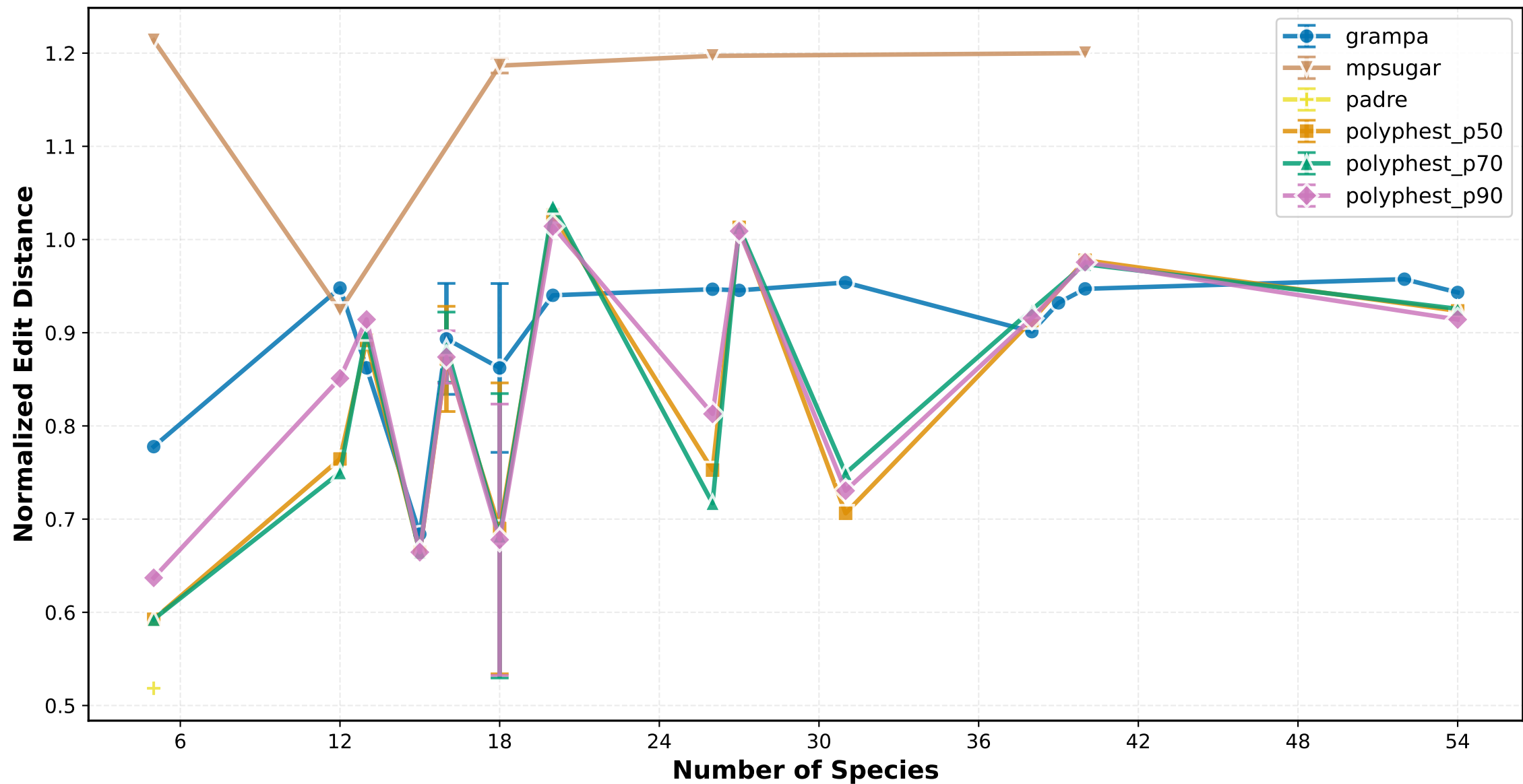
Normalized Edit Distance vs Number of Species ILS Medium
