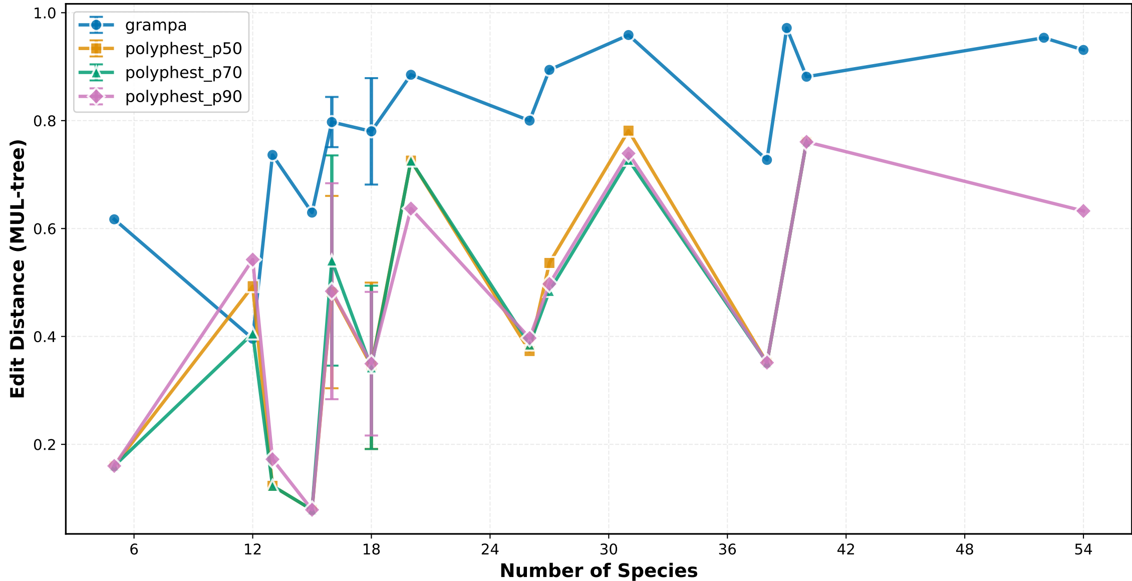
Edit Distance (MUL-tree) vs Number of Species ILS Medium
