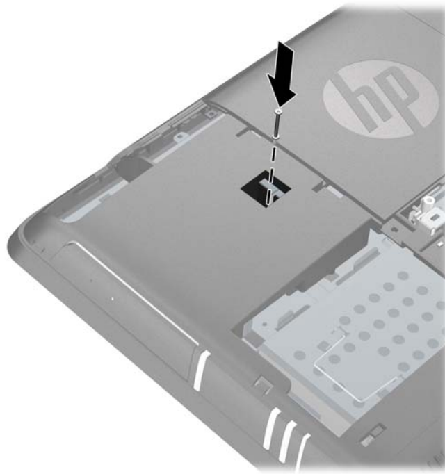
Figure 2-18 Installing the Optical Drive Security Screw
