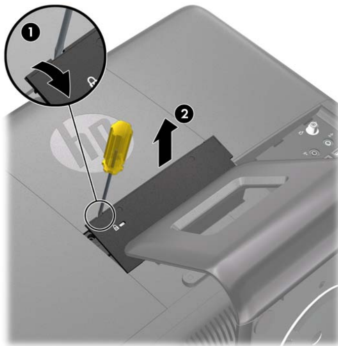
Figure 2-1 Removing the Center Access Panel
