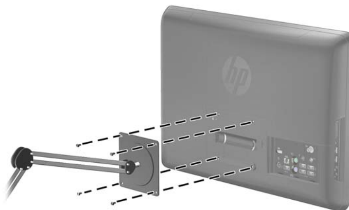
Figure 2-32 Mounting the Computer
