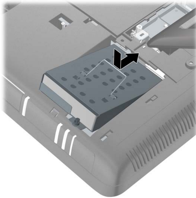
Figure 2-25 Installing the Hard Drive Cage
