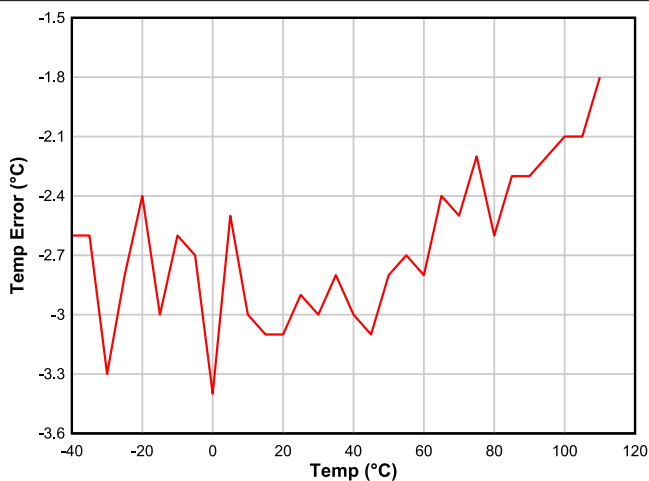
Figure 8-5. Thermistor Temperature Error
