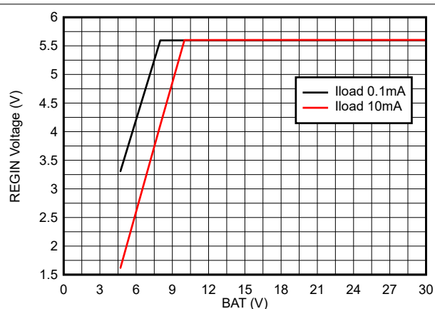
Figure 6-24. RGIN Voltage vs BAT Voltage
