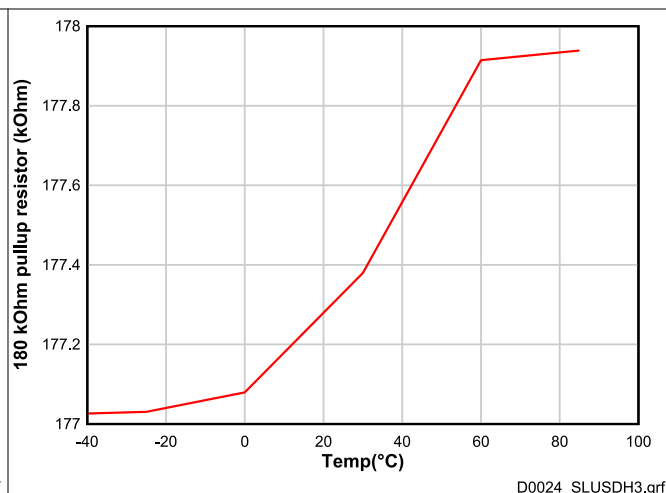
Figure 6-20. Thermistor Pullup Resistance vs Temperature (180-kΩ Setting)
