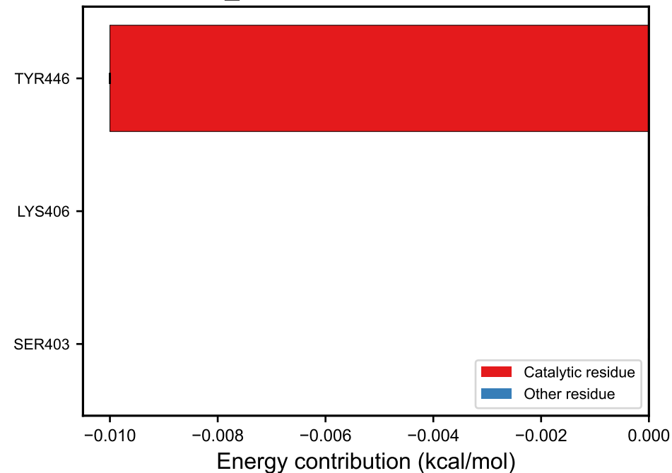
ALL_QU04: \Delta G = 0.13 kcal/mol
