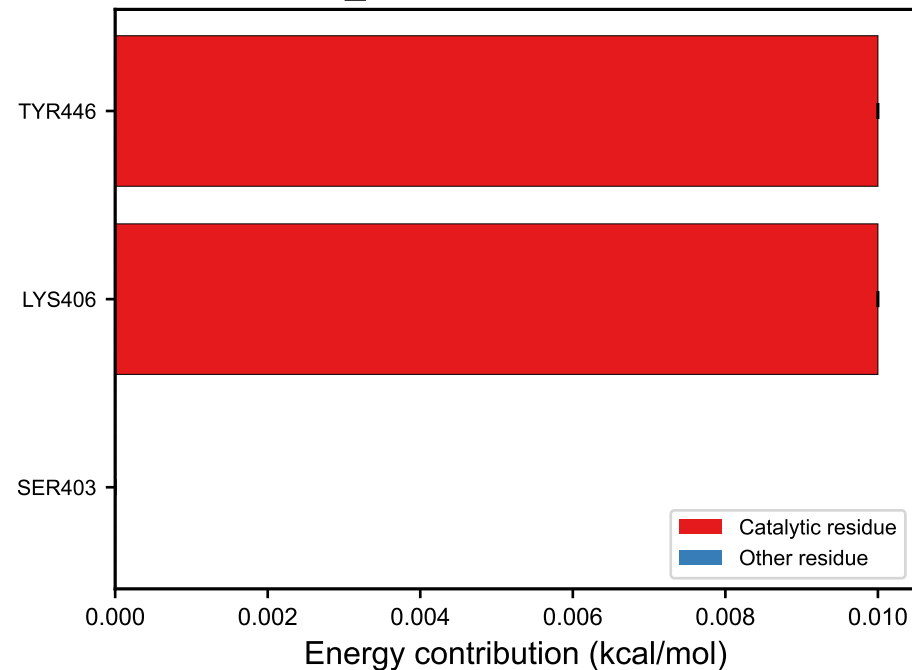
BRICS_0022: \Delta G = 0.45 kcal/mol
