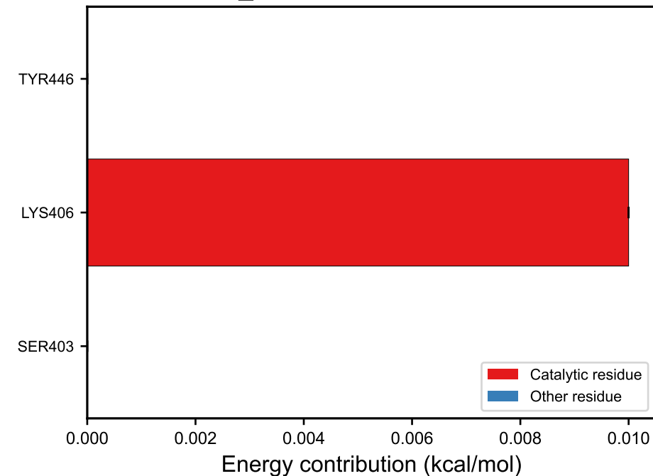
SEED_01150: \Delta G = 0.12 kcal/mol
