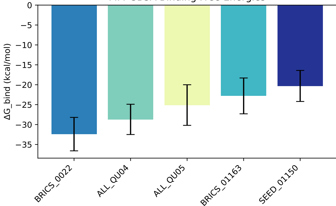
MM-GBSA Binding Free Energies
