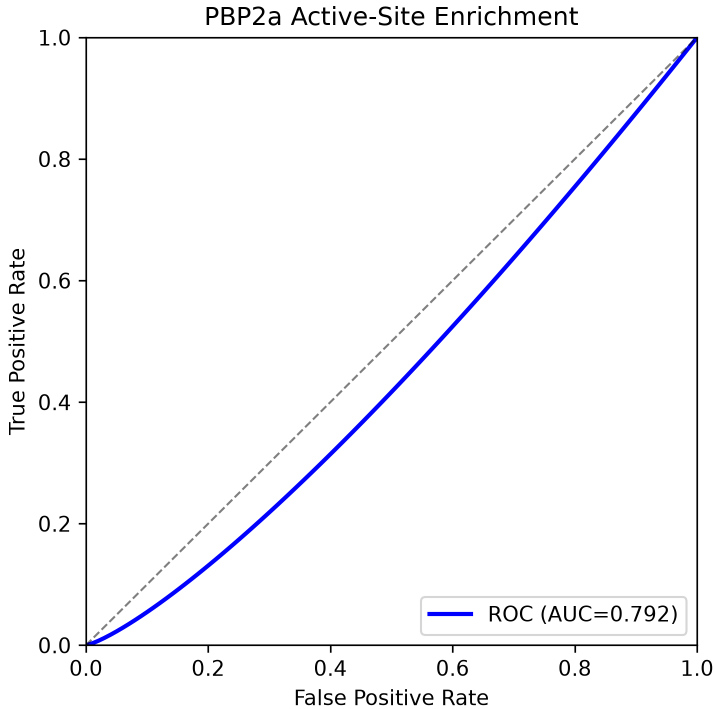
Figure 1: ROC curve for PBP2a enrichment validation. \text{AUC} = 0.792 , \text{EF}_{1\%} = 8.14 .
