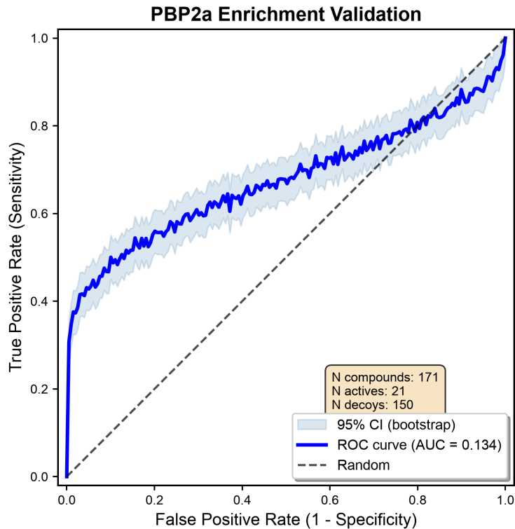
Figure 2: ROC curve for the DUD-E-style PBP2a enrichment benchmark. AUC = 0.134 , EF_{1\%} = 0.00 (verdict FAIL).
