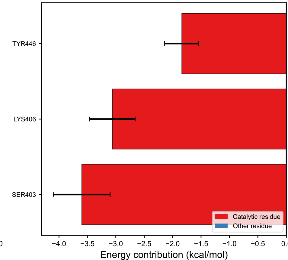
ALL_QU04: \Delta G = -34.4 kcal/mol
