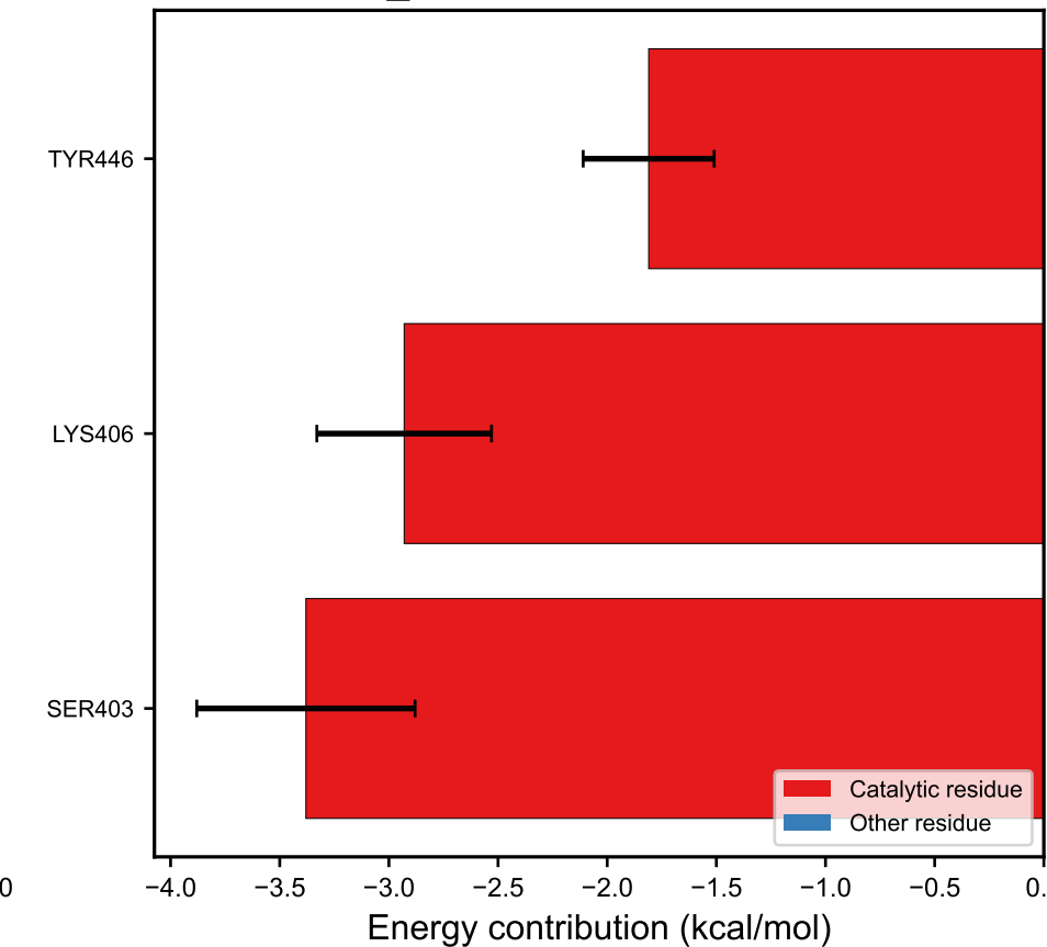
SEED_01150: \Delta G = -31.6 kcal/mol
