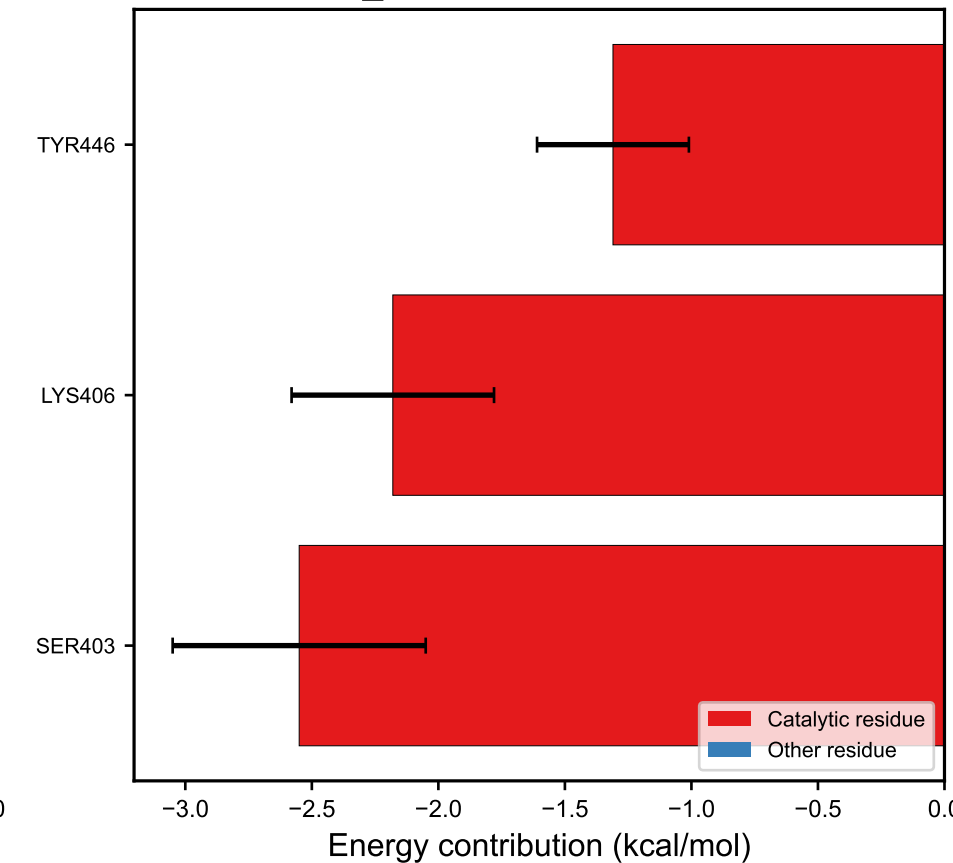
BRICS_0022: \Delta G = -20.4 kcal/mol
