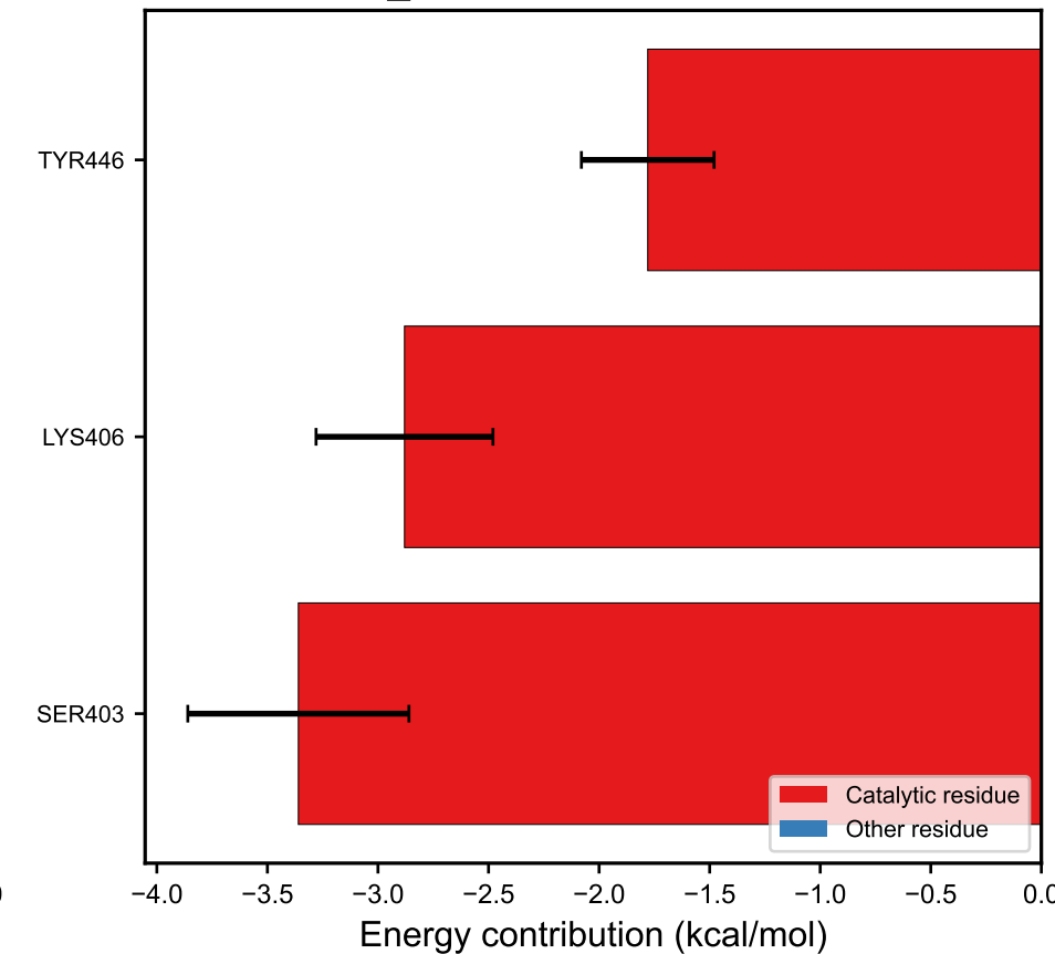
BRICS_01163: \Delta G = -31.4 kcal/mol
