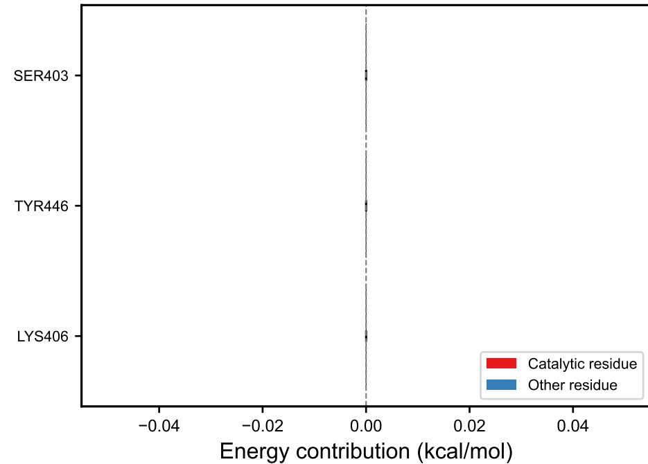
SEED_01150: \Delta G = 0.12 kcal/mol
