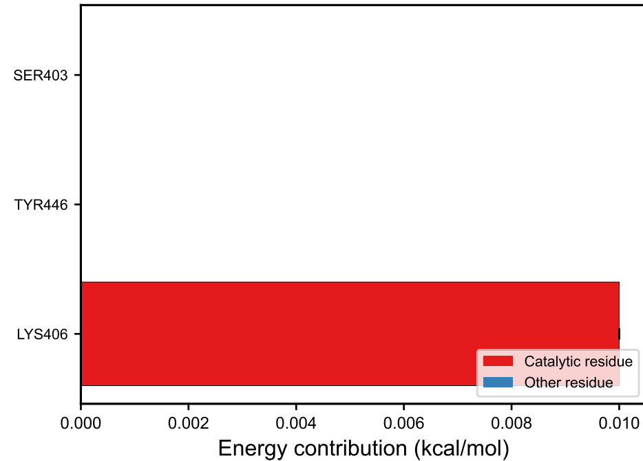
ALL_QU04: \Delta G = 0.13 kcal/mol
