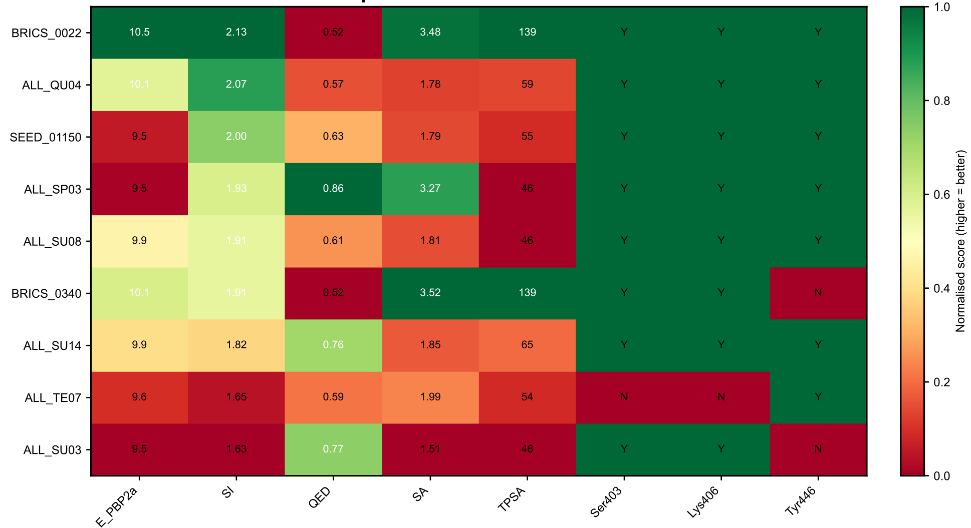
Comparative SAR of Lead Scaffolds
